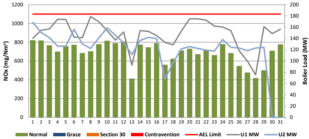
Figure 9: Camden Stack 1 NOx Emissions - August 2023
