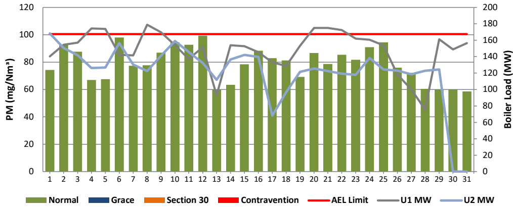
Figure 1: Camden Stack 1 PM Emissions - August 2023
