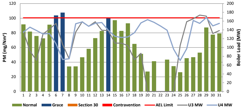
Figure 2: Camden Stack 2 PM Emissions - August 2023
