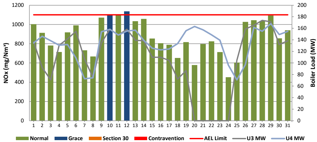
Figure 10: Camden Stack 2 NOx Emissions - August 2023
