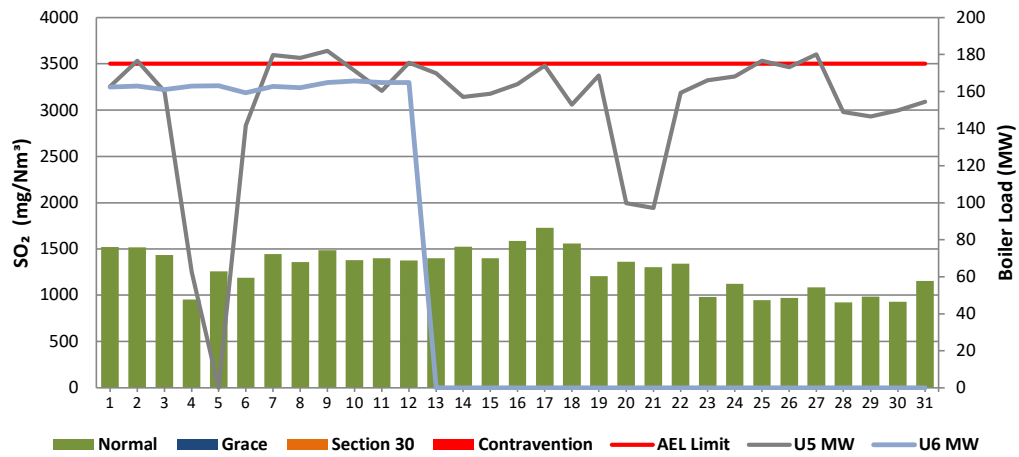
Figure 7: Camden Stack 3 SO 2 Emissions - August 2023
