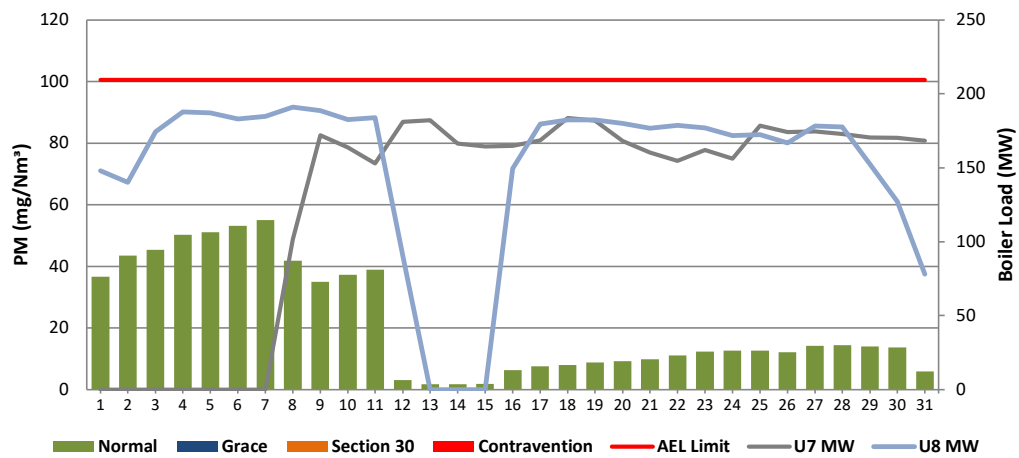
Figure 4: Camden Stack 4 PM Emissions - August 2023
