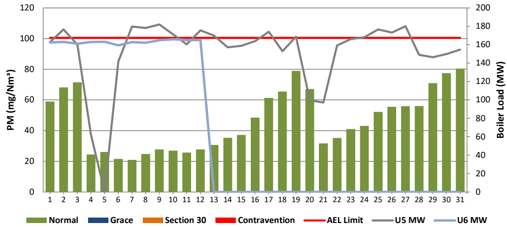
Figure 3: Camden Stack 3 PM Emissions - August 2023
