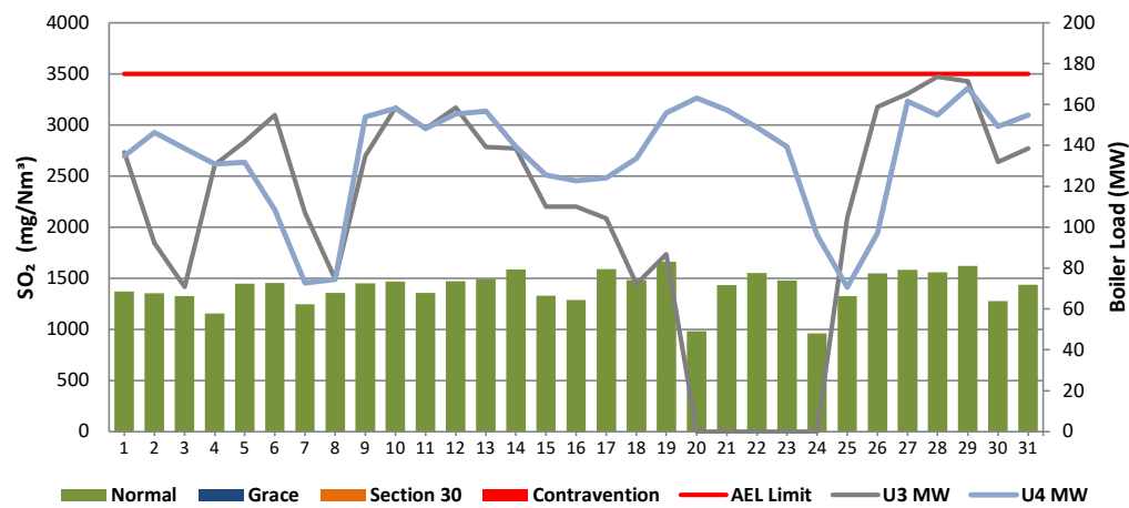
Figure 6: Camden Stack 2 SO 2 Emissions - August 2023
