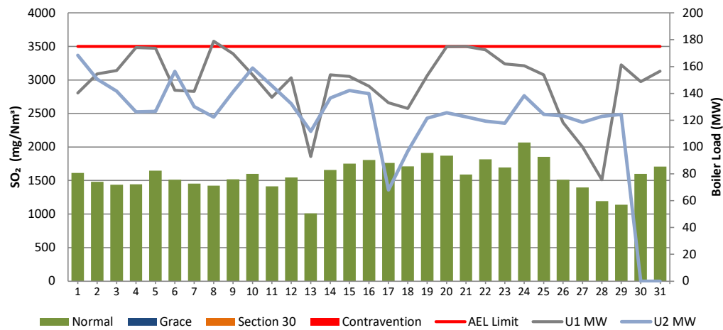
Figure 5: Camden Stack 1 SO 2 Emissions - August 2023
