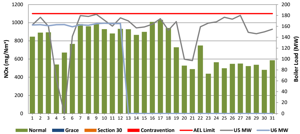
Figure 11: Camden Stack 3 NOx Emissions - August 2023
