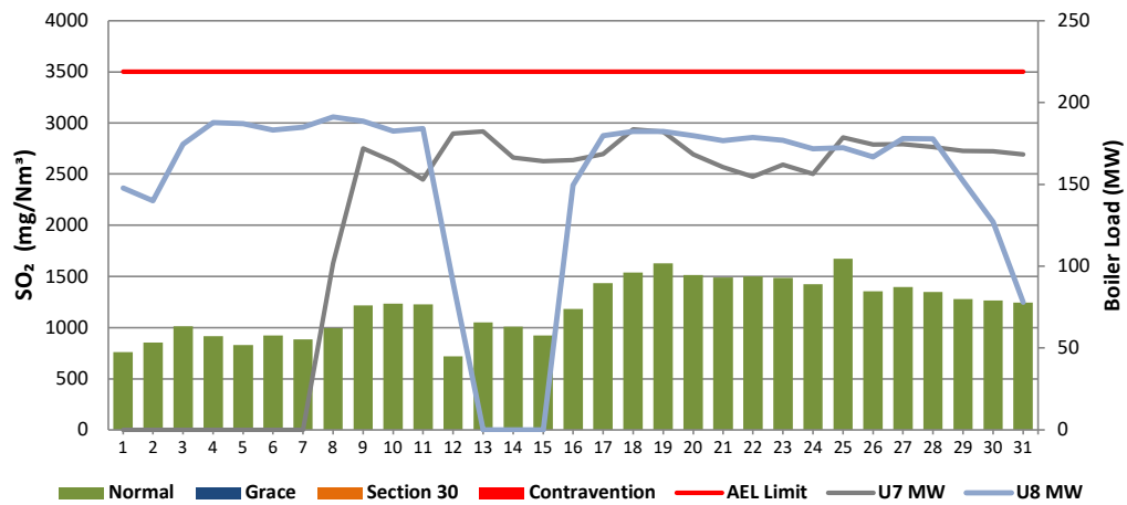
Figure 8: Camden Stack 4 SO 2 Emissions - August 2023
