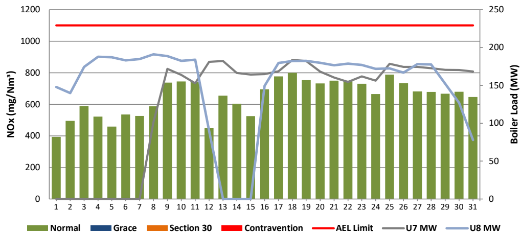
Figure 12: Camden Stack 4 NOx Emissions - August 2023
