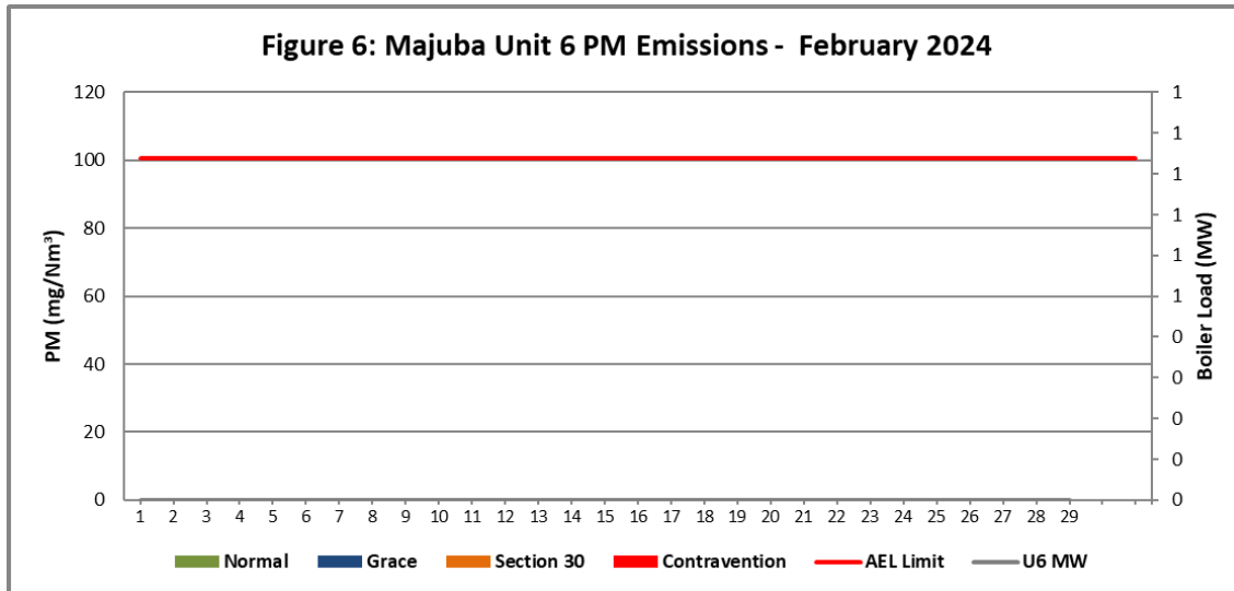
Figure 6. Particulate Matter emissions (daily averages) for the month of February 2024 against emission limit for Unit 6.
