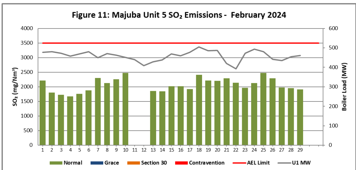
Figure 11. SO 2 emissions (daily averages) for the month of February 2024 against emission limit for Unit 5
