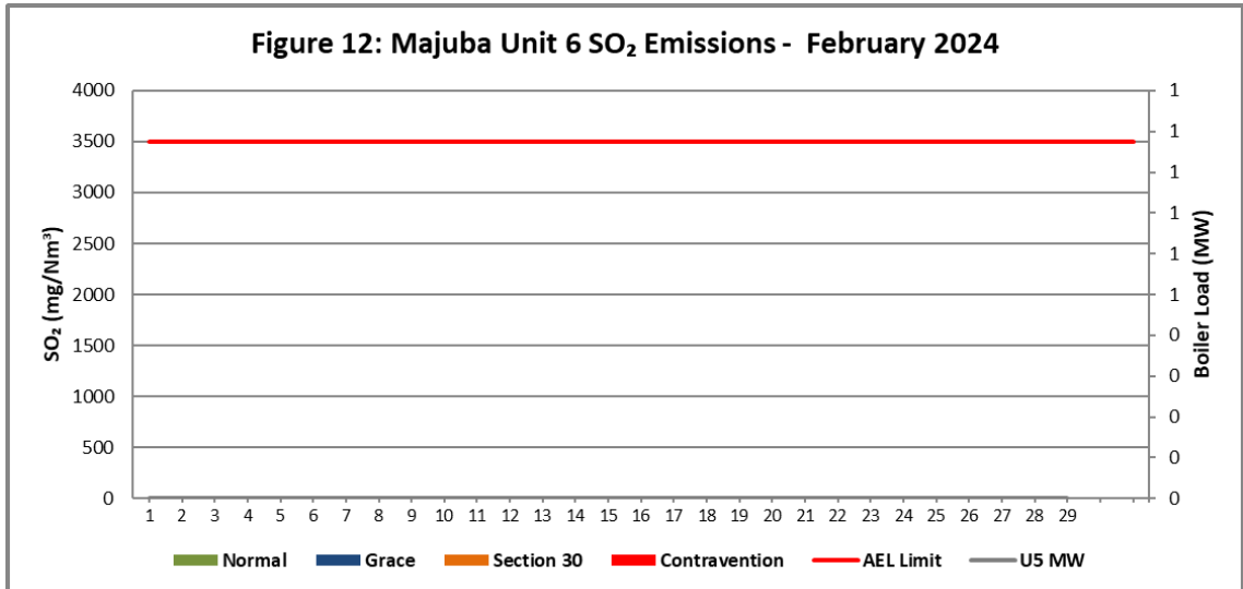
Figure 12. SO 2 emissions (daily averages) for the month of February 2024 against emission limit for Unit 6.
