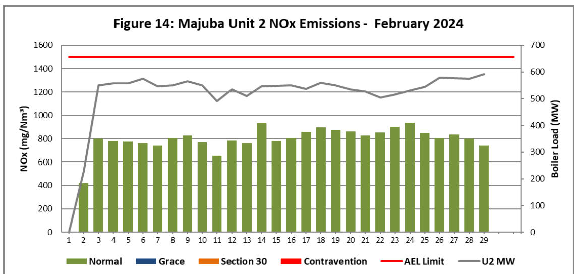
Figure 14. NO x emissions (daily averages) for the month of February 2024 against emission limit for Unit 2.
