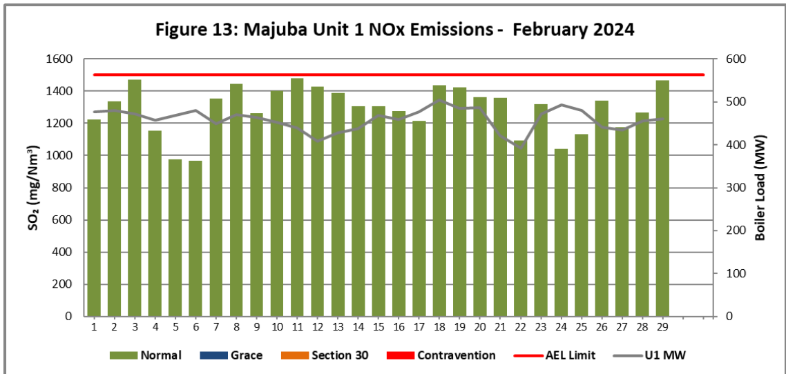
Figure 13. NO x emissions (daily averages) for the month of February 2024 against emission limit for Unit 1.
