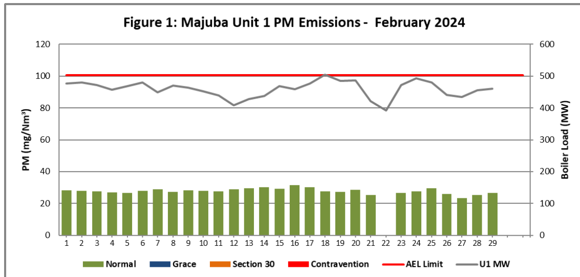
Figure 1. Particulate Matter emissions (daily averages) for the month of February 2024 against emission limit for Unit 1.
