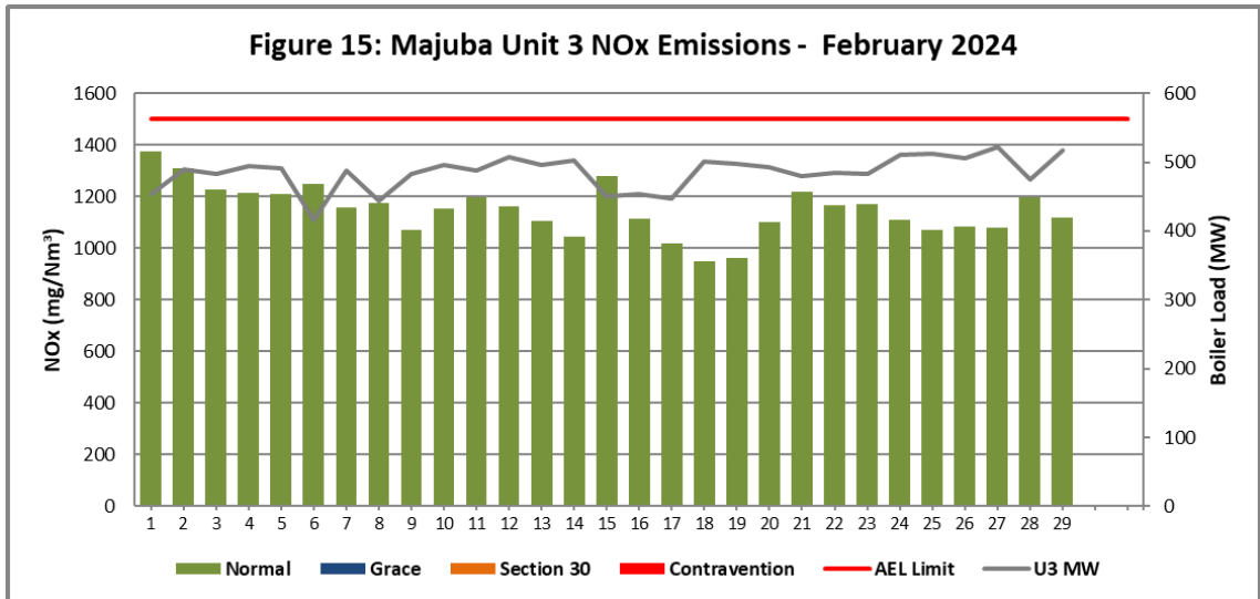
Figure 15. NOx emissions (daily averages) for the month of February 2024 against emission limit for Unit 3.
