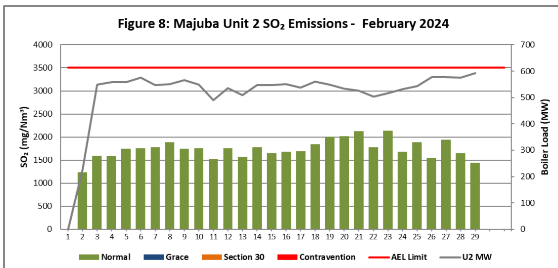
Figure 8. SO 2 emissions (daily averages) for the month of February 2024 against emission limit for Unit 2.
