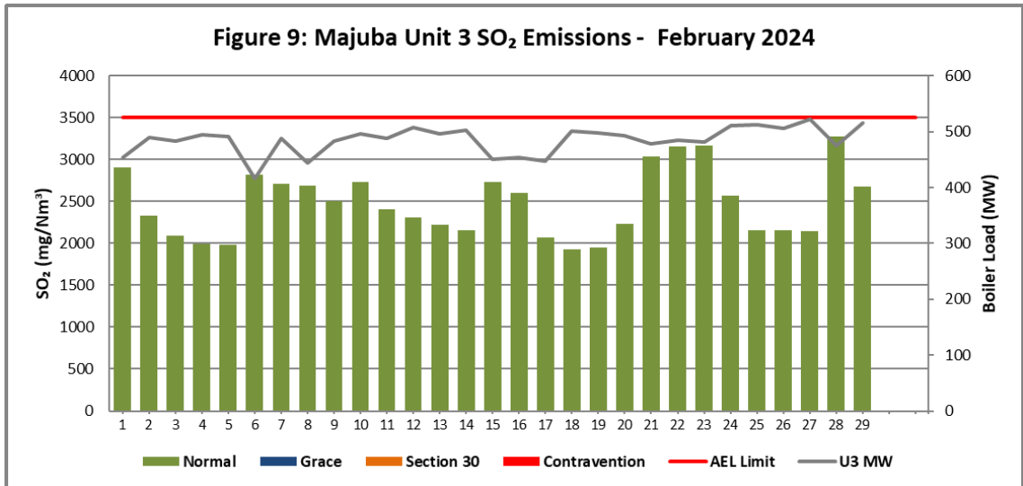
Figure 9. SO 2 emissions (daily averages) for the month of February 2024 against emission limit for Unit 3.
