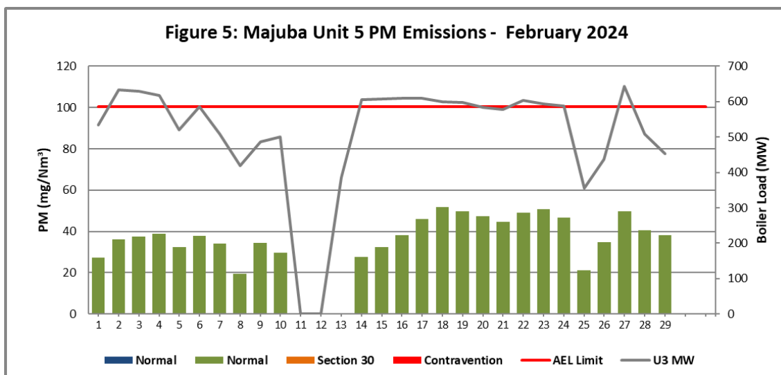
Figure 5. Particulate Matter emissions (daily averages) for the month of February 2024 against emission limit for Unit 5.
