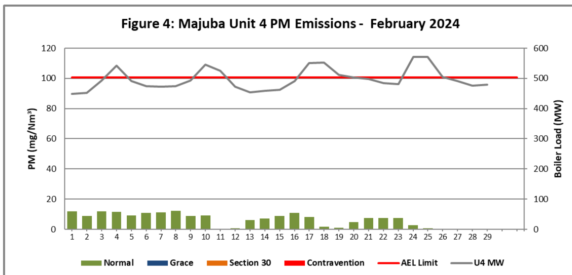
Figure 4. Particulate Matter emissions (daily averages) for the month of February 2024 against emission limit for Unit 4.
