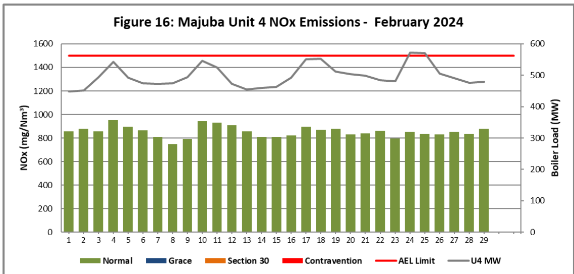
Figure 16. NOx emissions (daily averages) for the month of February 2024 against emission limit for Unit 4
