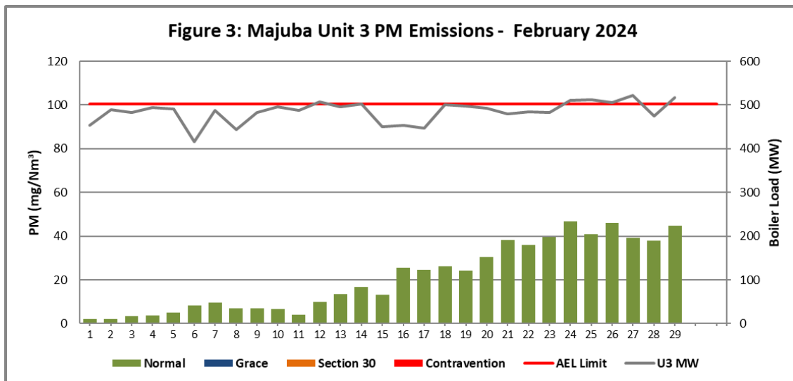
Figure 3. Particulate Matter emissions (daily averages) for the month of February 2024 against emission limit for Unit 3.
