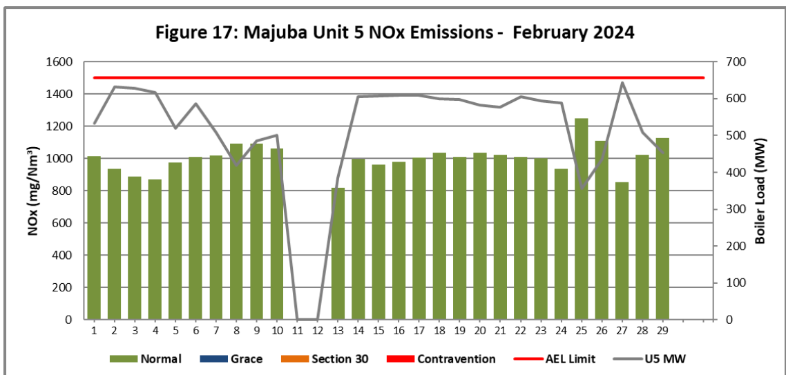
Figure 17. NOx emissions (daily averages) for the month of February 2024 against emission limit for Unit 5
