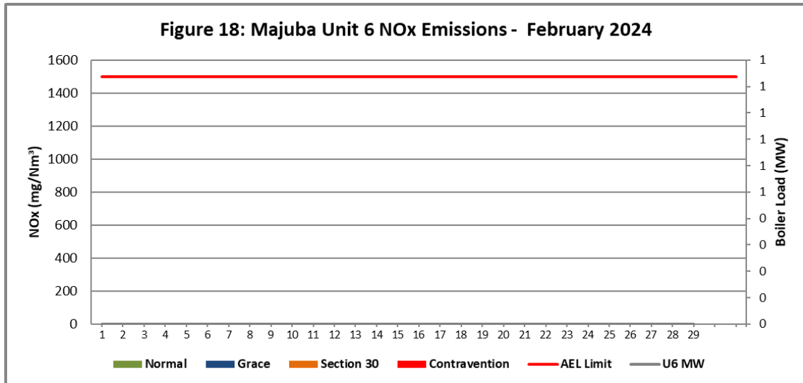
Figure 18. NOx emissions (daily averages) for the month February 2024 against emission limit for Unit 6
