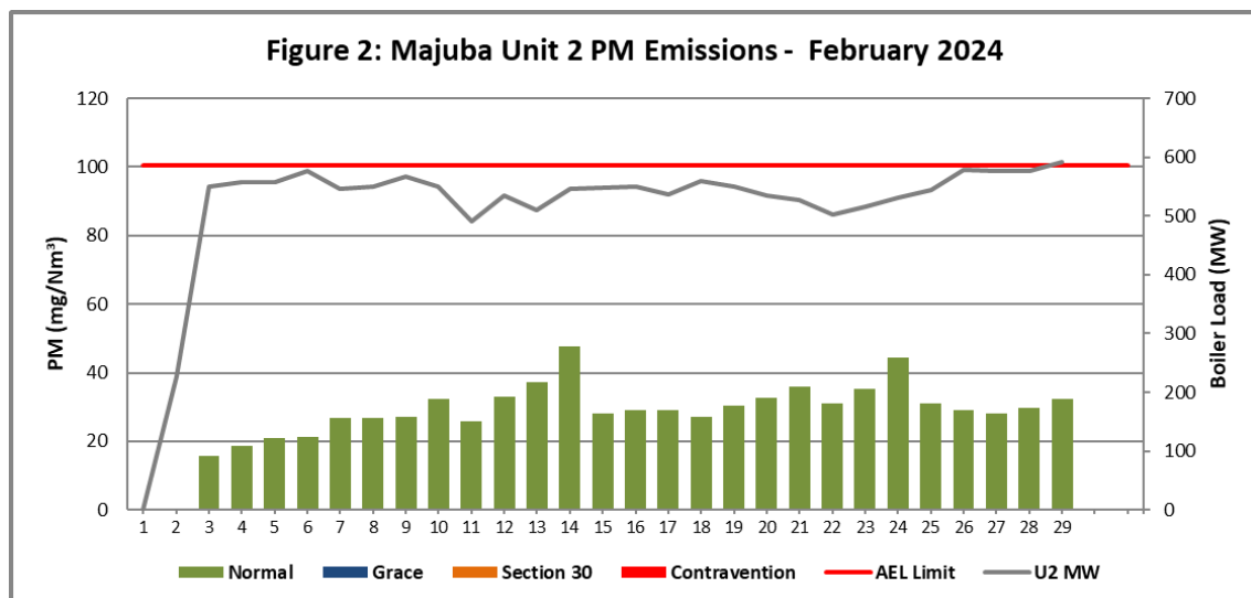
Figure 2. Particulate Matter emissions (daily averages) for the month of February 2024 against emission limit for Unit 2.
