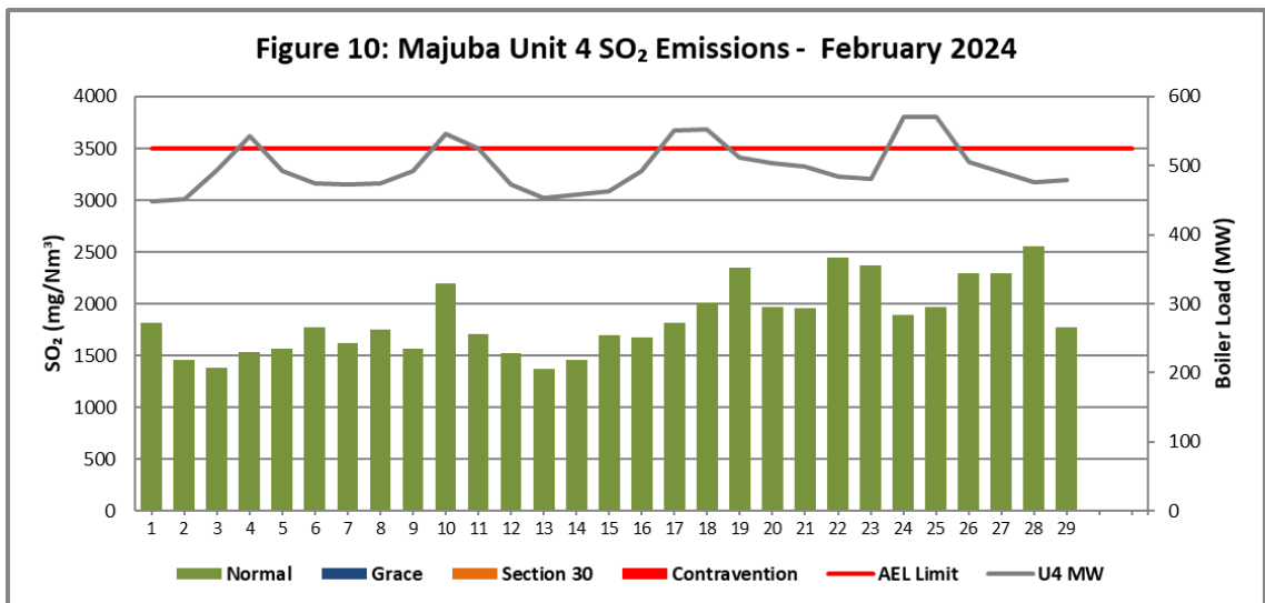
Figure 10. SO 2 emissions (daily averages) for the month of February 2024 against emission limit for Unit 4.
