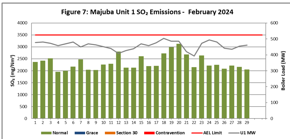
Figure 7. SO 2 emissions (daily averages) for the month of February 2024 against emission limit for Unit 1.
