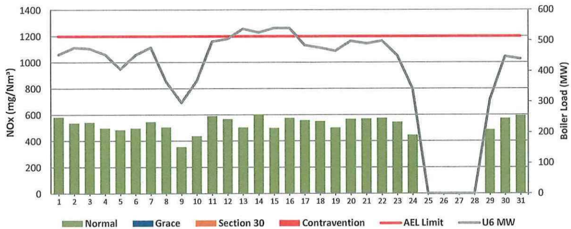
Figure 12: Matla Unit 6 NOx Emissions - December 2023
