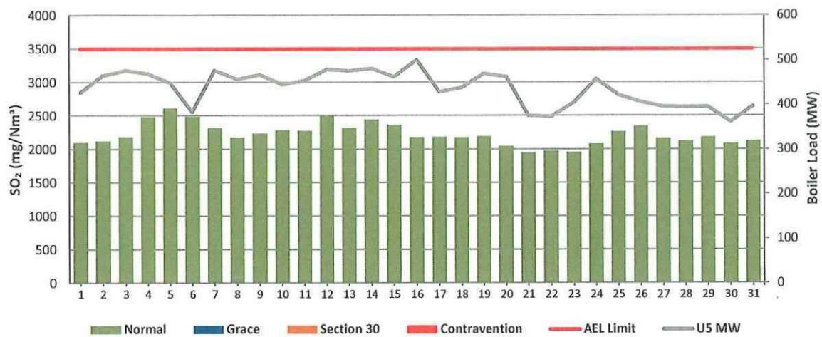
Figure 7: Matla Unit 5 SO 2 Emissions - December 2023
