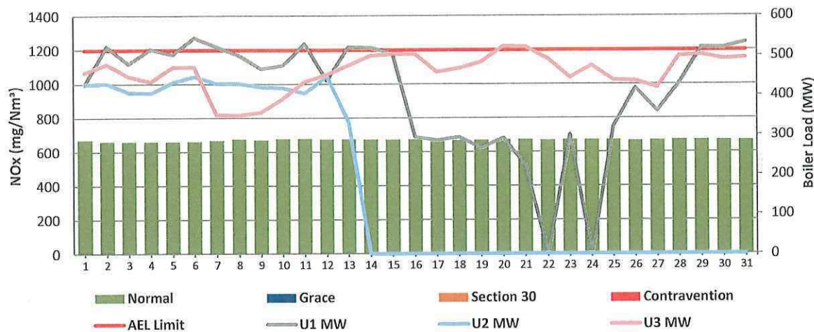
Figure 9: Matla South Stack NOx Emissions - December 2023
