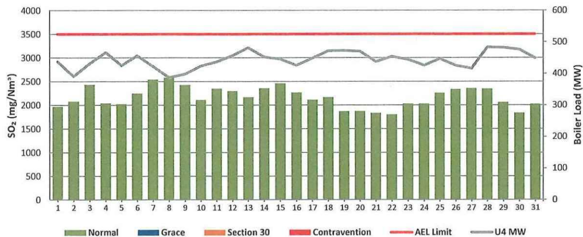
Figure 6: Matla Unit 4 SO 2 Emissions - December 2023
