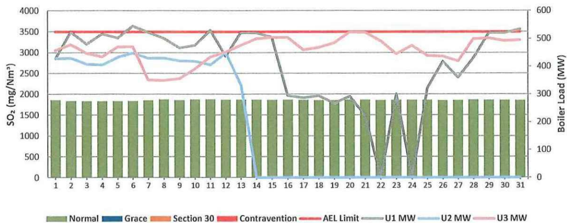
Figure 5: Matla South Stack SO 2 Emissions - December 23
