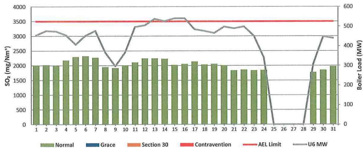
Figure 8: Matla Unit 6 SO 2 Emissions - December 2023
