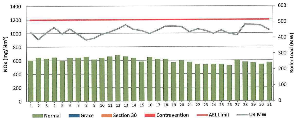
Figure 10: Matla Unit 4 NOx Emissions - December 2023
