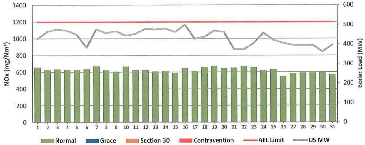
Figure 11: Matla Unit 5 NOx Emissions - December 2023
