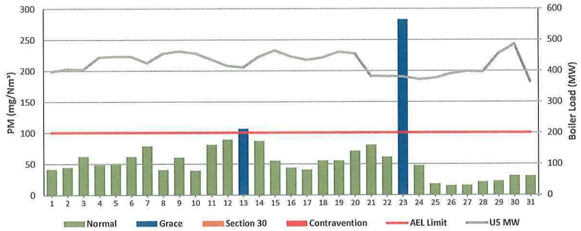
Figure 3: Matla Unit 5 PM Emissions - January 2024
