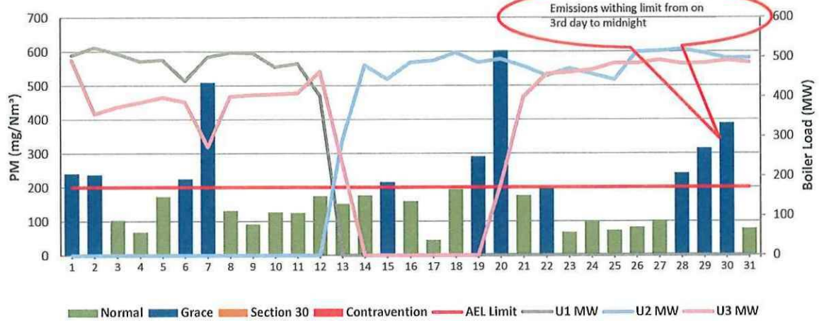
Figure 1: Matla South Stack PM Emissions - January 2024
