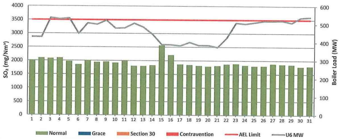
Figure 8: Matla Unit 6 SO 2 Emissions - January 2024
