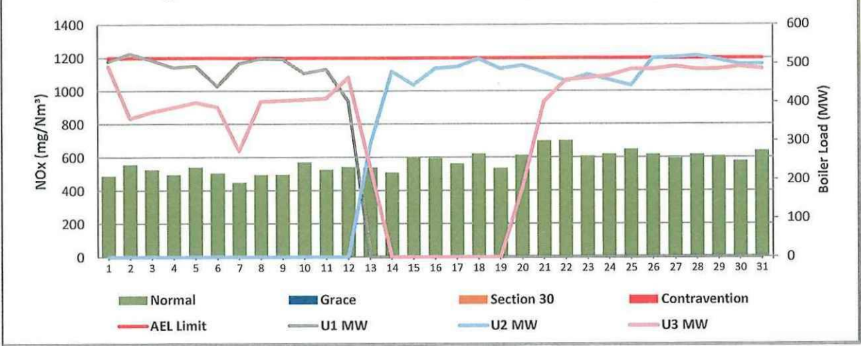
Figure 9: Matla South Stack NOx Emissions - January 2024
