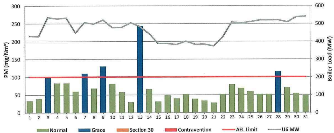
Figure 4: Matla Unit 6 PM Emissions - January 2024
