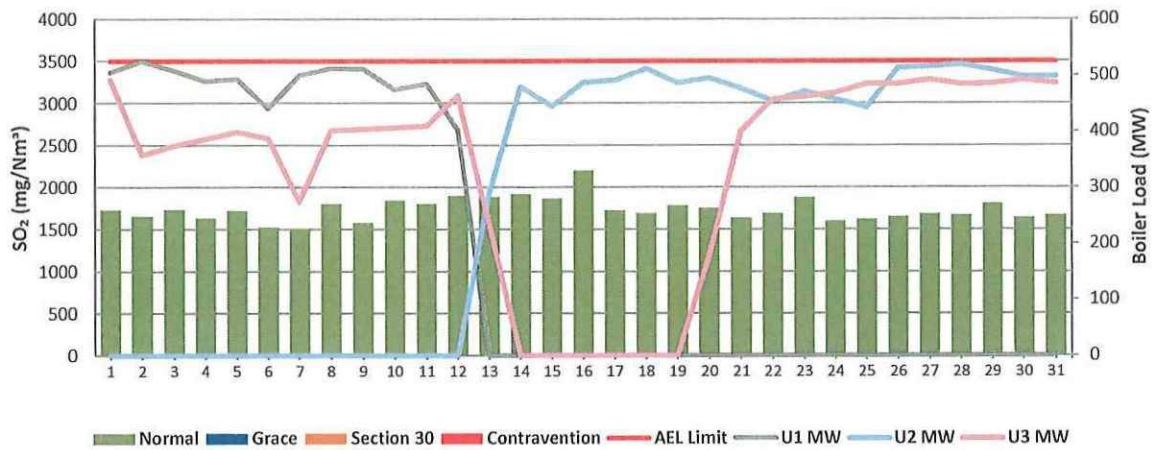
Figure 5: Matla South Stack SO 2 Emissions - January 24
