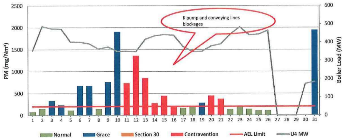
Figure 2: Matla Unit 4 PM Emissions - January 2024
