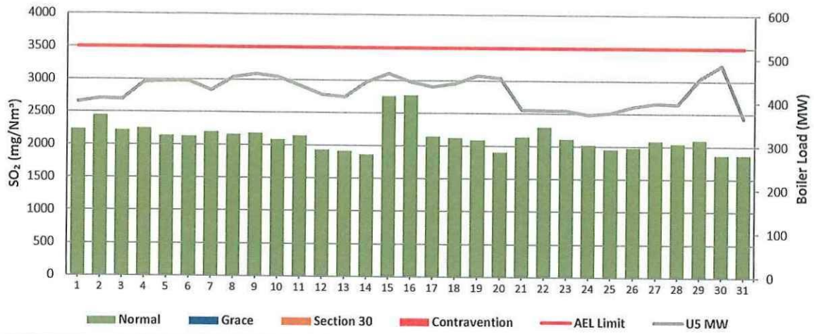
Figure 7: Matla Unit 5 SO 2 Emissions - January 2024
