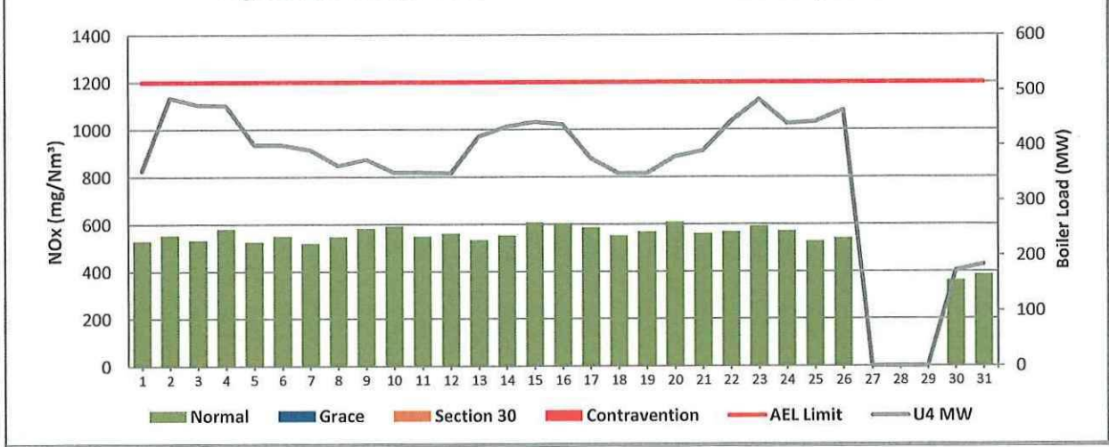
Figure 10: Matla Unit 4 NOx Emissions - January 2024
