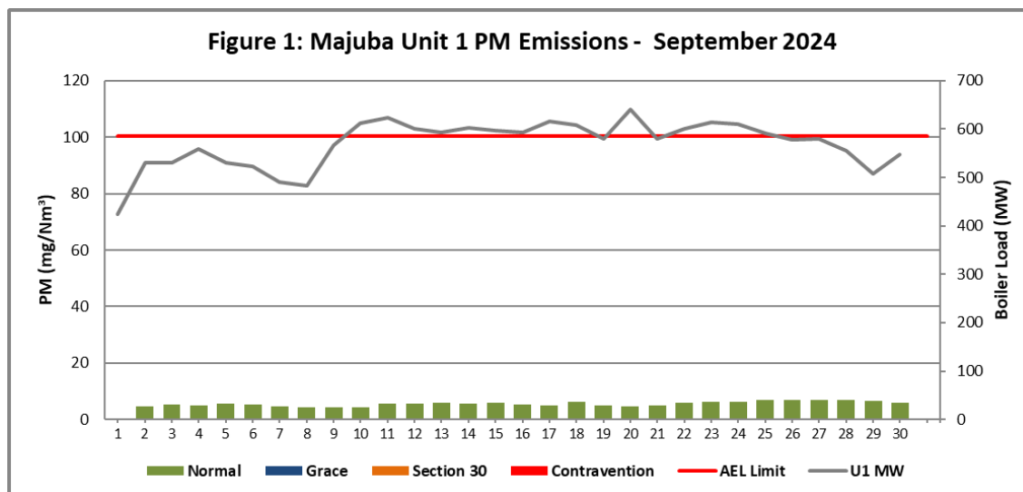
Figure 1. Particulate Matter emissions (daily averages) for the month of September 2024 against emission limit for Unit 1.
