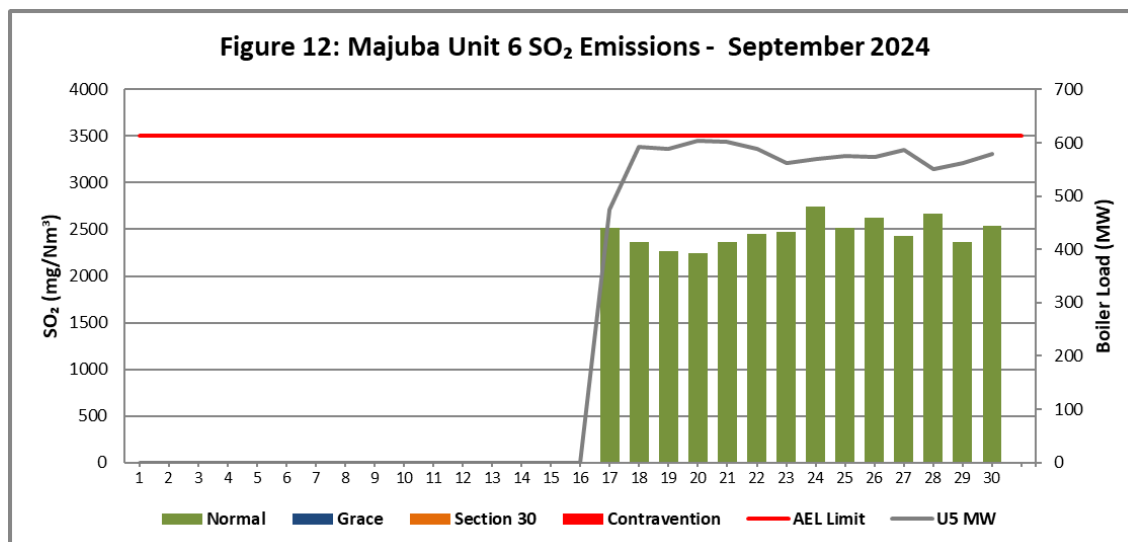
Figure 12. SO 2 emissions (daily averages) for the month of September 2024 against emission limit for Unit 6.
