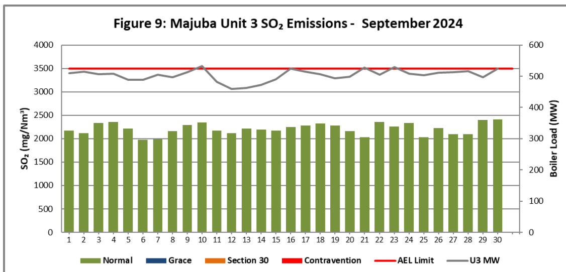
Figure 9. SO 2 emissions (daily averages) for the month of September 2024 against emission limit for Unit 3.
