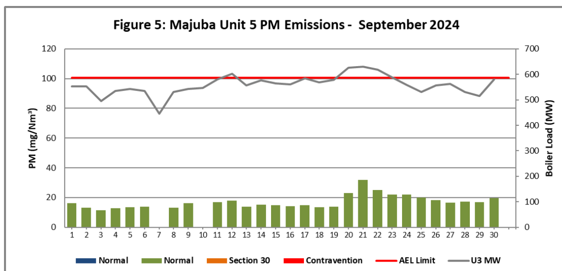
Figure 5. Particulate Matter emissions (daily averages) for the month of September 2024 against emission limit for Unit 5.
