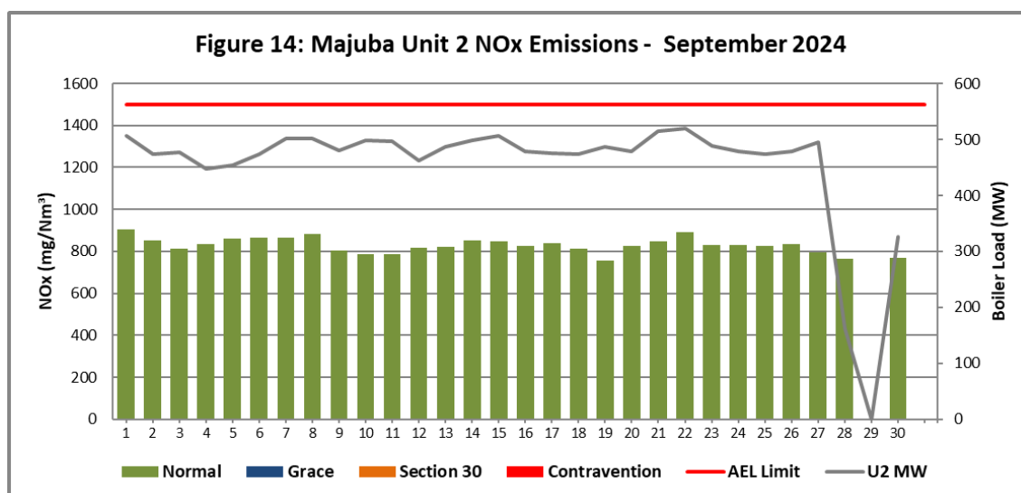
Figure 14. NO x emissions (daily averages) for the month of September 2024 against emission limit for Unit 2.
