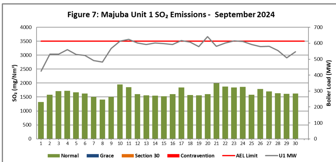
Figure 7. SO₂ emissions (daily averages) for the month of September 2024 against emission limit for Unit 1.
