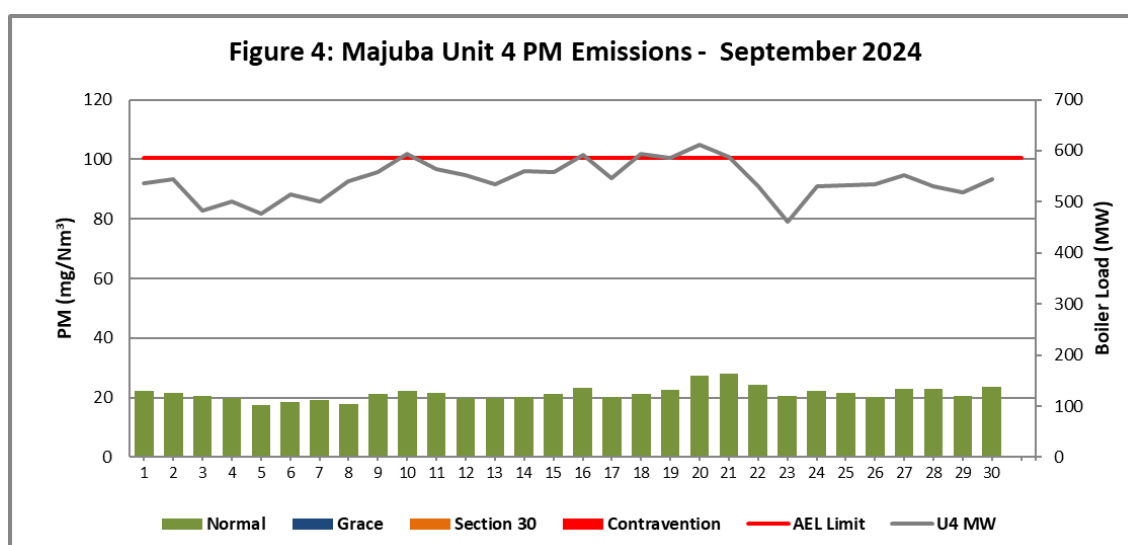
Figure 4. Particulate Matter emissions (daily averages) for the month of September 2024 against emission limit for Unit 4.
