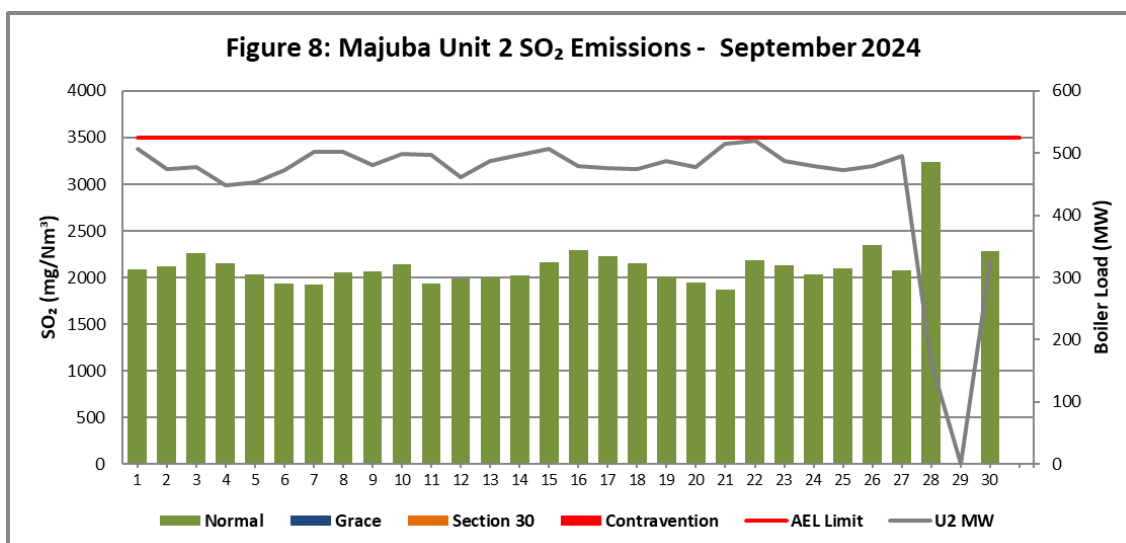
Figure 8. SO₂ emissions (daily averages) for the month of September 2024 against emission limit for Unit 2.
