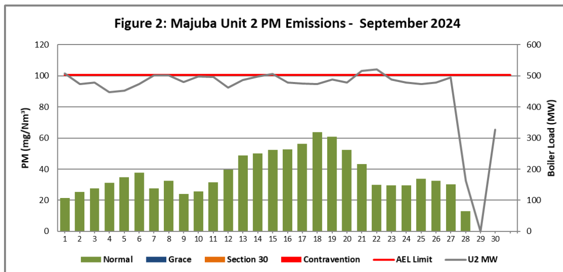
Figure 2. Particulate Matter emissions (daily averages) for the month of September 2024 against emission limit for Unit 2.
