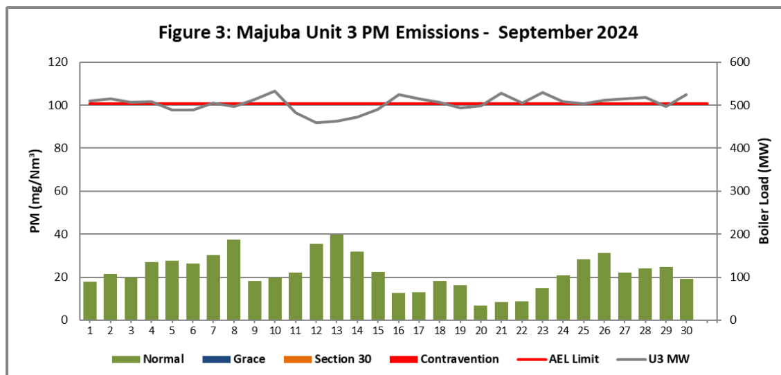
Figure 3. Particulate Matter emissions (daily averages) for the month of September 2024 against emission limit for Unit 3.
