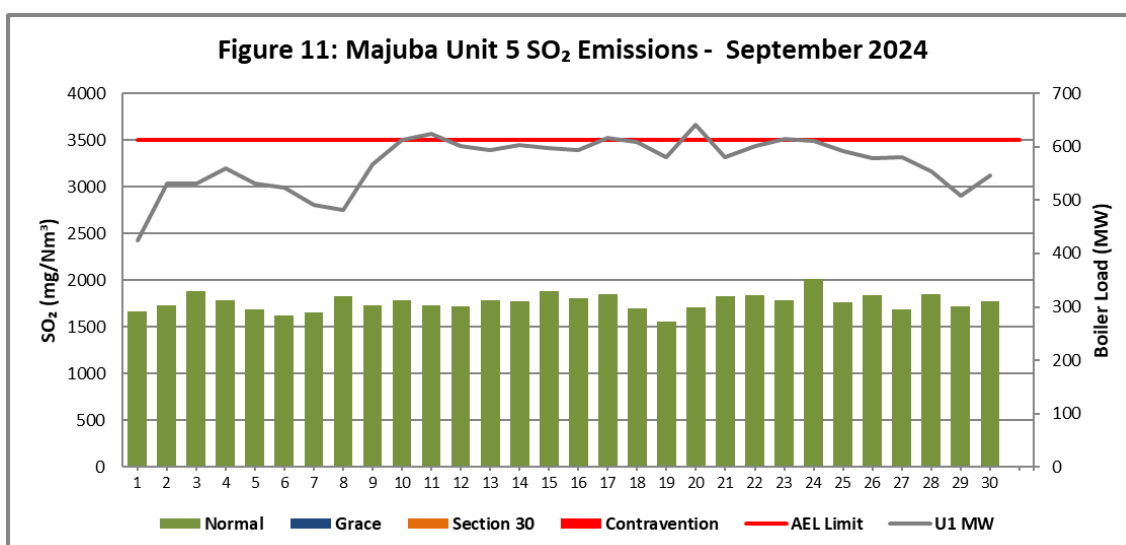
Figure 11. SO 2 emissions (daily averages) for the month of September 2024 against emission limit for Unit 5.
