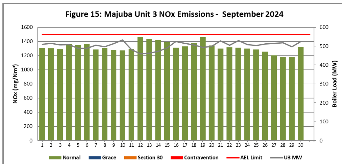
Figure 15. NOx emissions (daily averages) for the month of September 2024 against emission limit for Unit 3.
