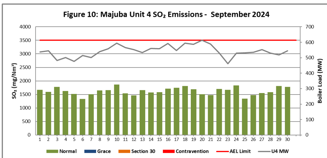
Figure 10. SO 2 emissions (daily averages) for the month of September 2024 against emission limit for Unit 4.
