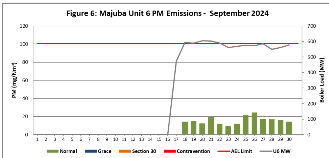
Figure 6. Particulate Matter emissions (daily averages) for the month of September 2024 against emission limit for Unit 6.
