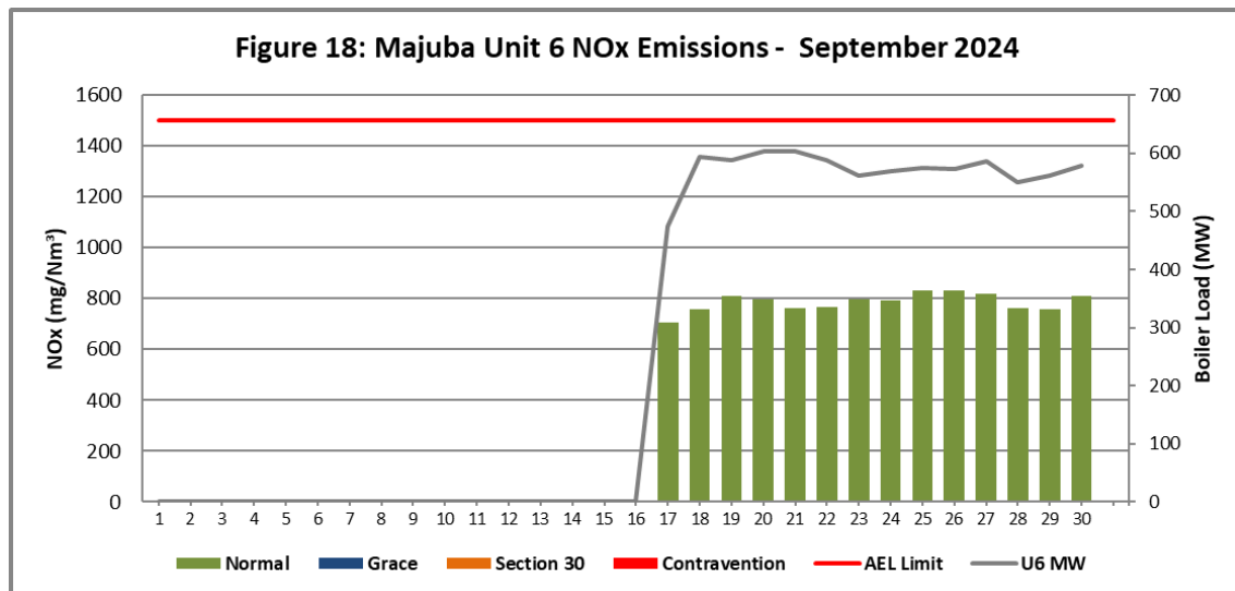
Figure 18. NO x emissions (daily averages) for the month September 2024 against emission limit for Unit 6
