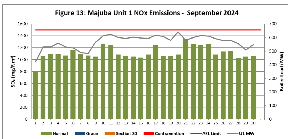
Figure 13. NO x emissions (daily averages) for the month of September 2024 against emission limit for Unit 1.
