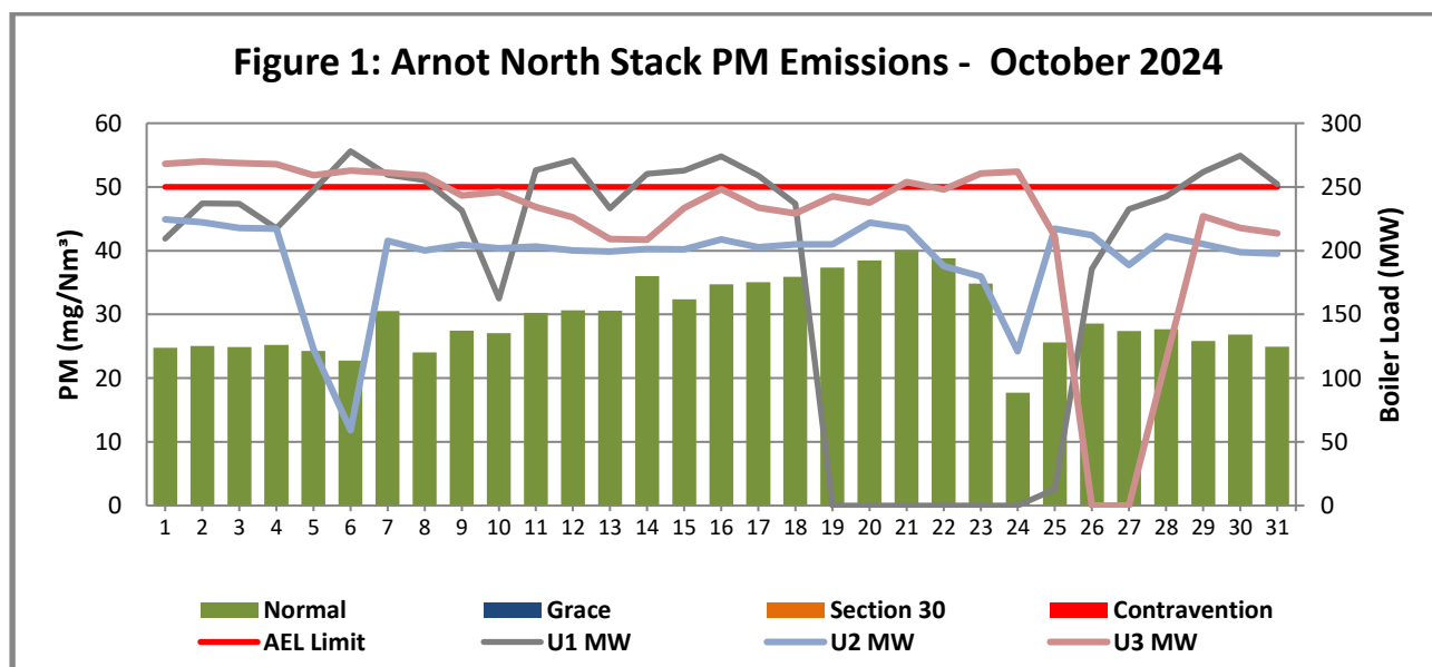
Figure 1: PM emissions (daily averages) for the month of October 2024 against the emission limit for the North Stack
