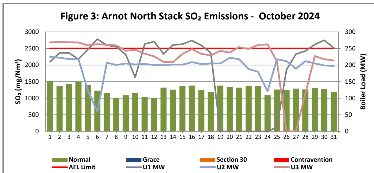
Figure 3: SO 2 emissions (daily averages) for the month of October 2024 against emission limit for the North Stack
