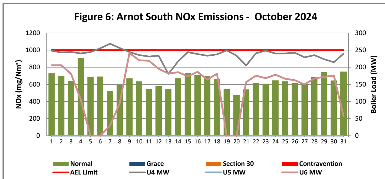
Figure 6: NO 2 emissions (daily averages) for the month of October 2024 against emission limit for the South Stack
