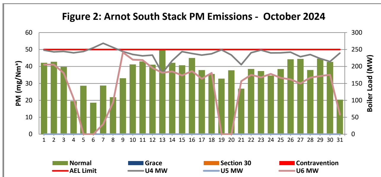
Figure 2: PM emissions (daily averages) for the month of October 2024 against emission limit for the South Stack
