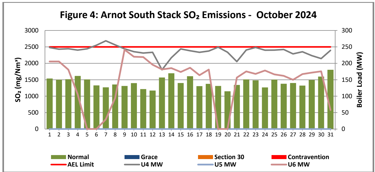
Figure 4: SO 2 emissions (daily averages) for the month of October 2024 against emission limit for the South Stack
