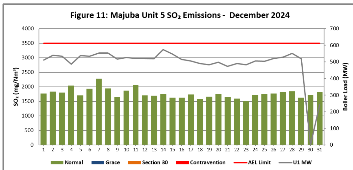
Figure 11. SO 2 emissions (daily averages) for the month of December 2024 against emission limit for Unit 5.
