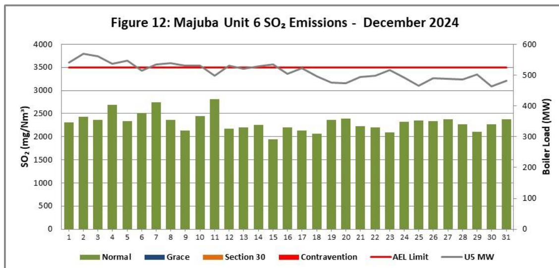
Figure 12. SO 2 emissions (daily averages) for the month of December 2024 against emission limit for Unit 6.
