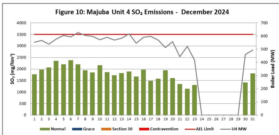
Figure 10. SO 2 emissions (daily averages) for the month of December 2024 against emission limit for Unit 4.
