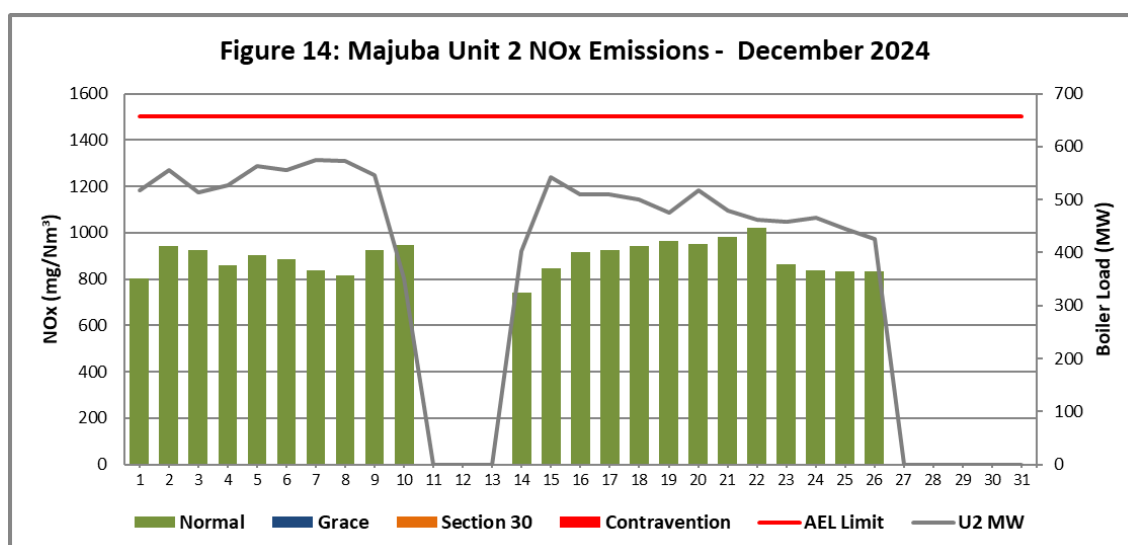
Figure 14. NO x emissions (daily averages) for the month of December 2024 against emission limit for Unit 2.
