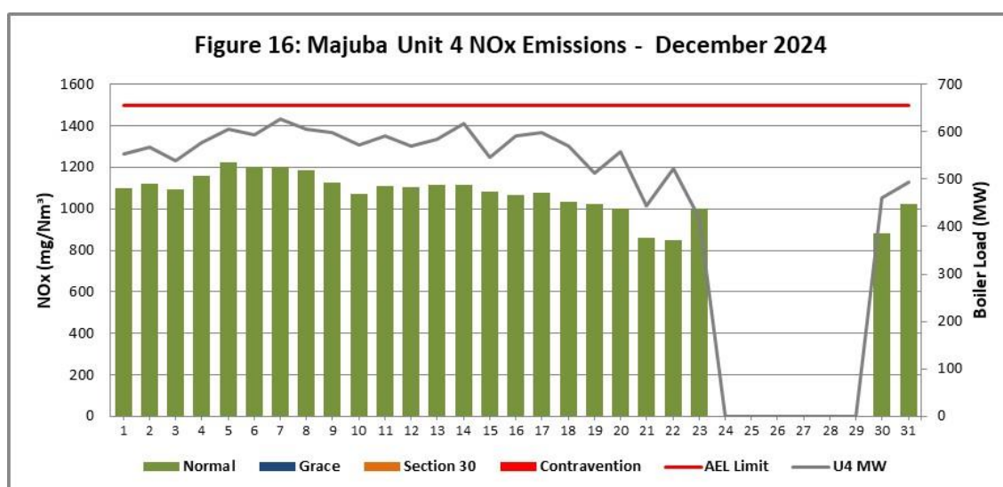
Figure 16. NOx emissions (daily averages) for the month of December 2024 against emission limit for Unit 4
