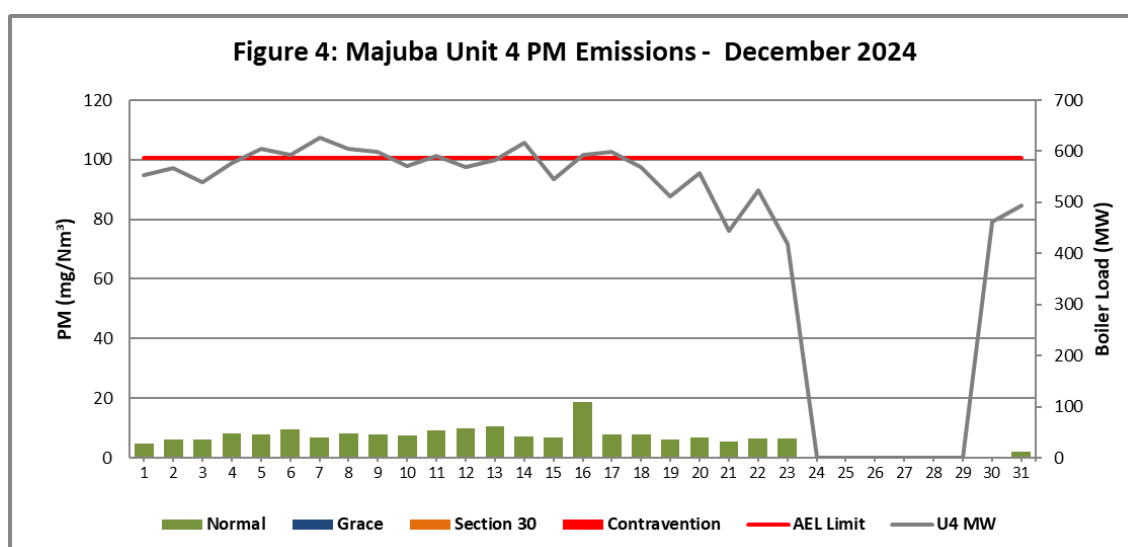
Figure 4. Particulate Matter emissions (daily averages) for the month of December 2024 against emission limit for Unit 4.
