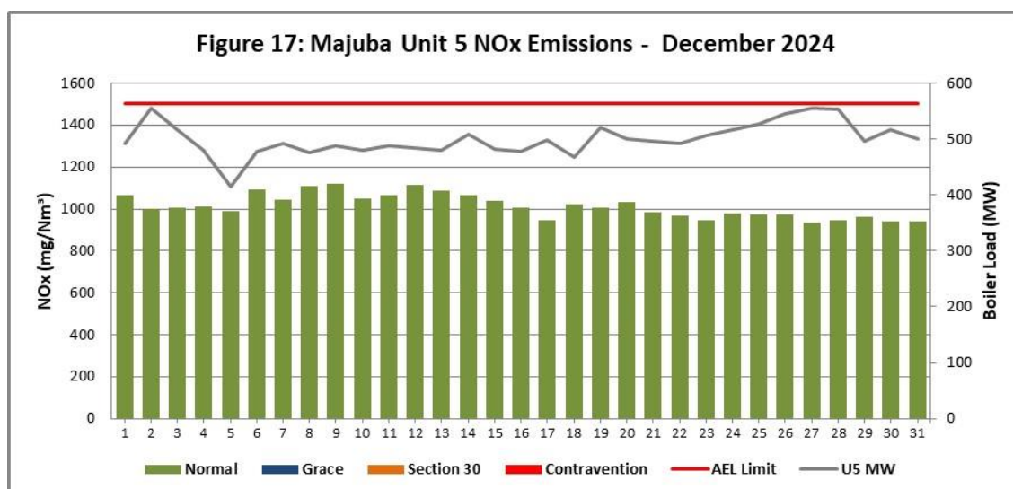
Figure 17. NOx emissions (daily averages) for the month of December 2024 against emission limit for Unit 5
