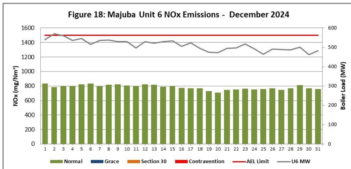
Figure 18. NOx emissions (daily averages) for the month December 2024 against emission limit for Unit 6
