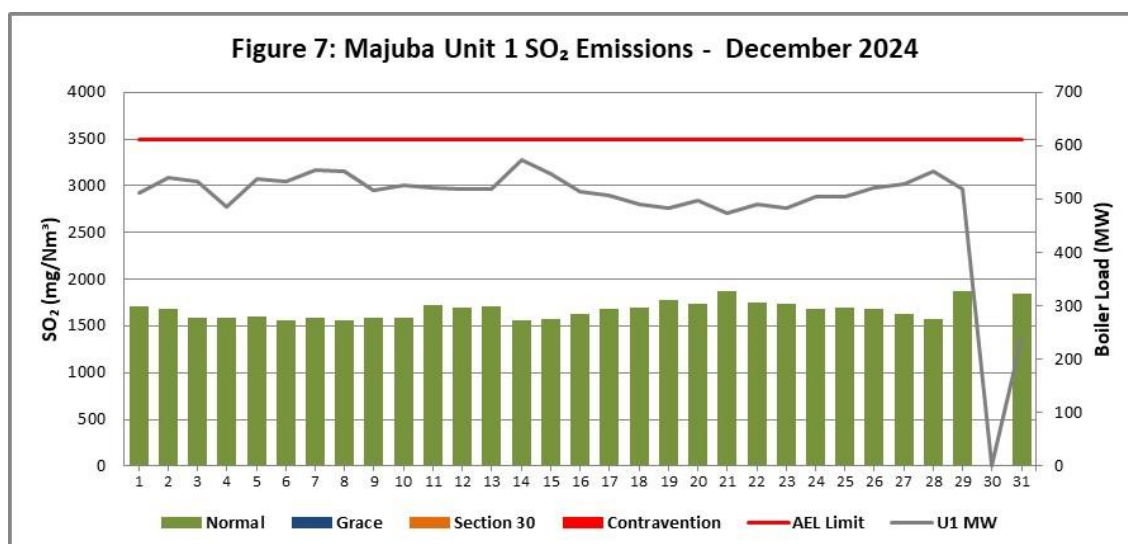
Figure 7. SO₂ emissions (daily averages) for the month of December 2024 against emission limit for Unit 1.
