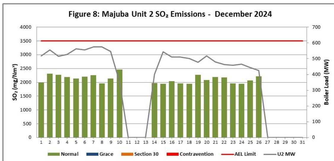
Figure 8. SO₂ emissions (daily averages) for the month of December 2024 against emission limit for Unit 2.
