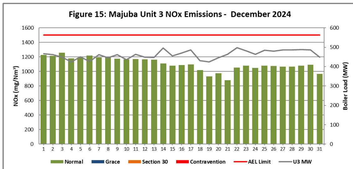
Figure 15. NOx emissions (daily averages) for the month of December 2024 against emission limit for Unit 3.
