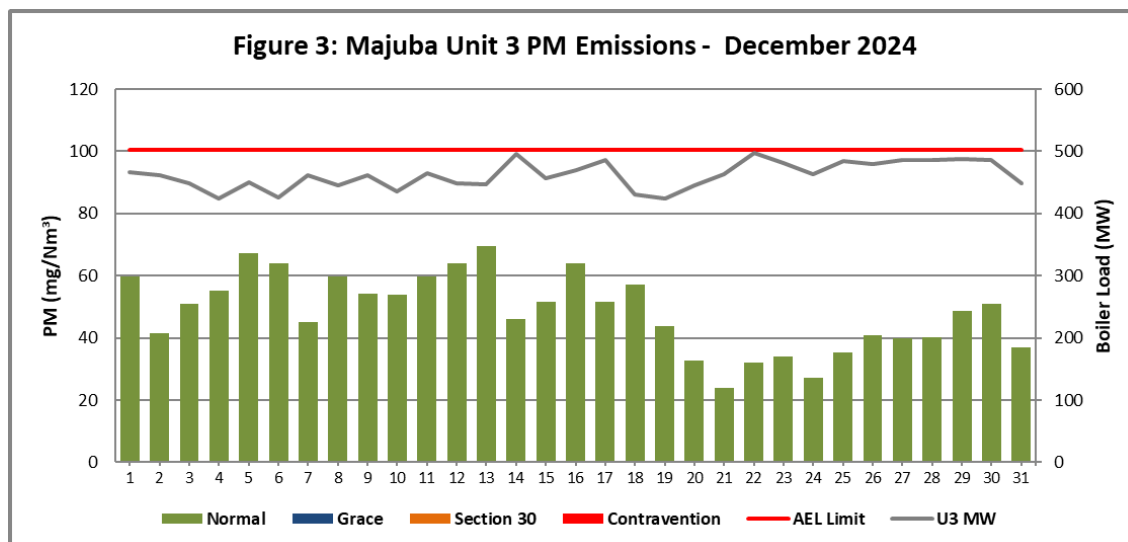
Figure 3. Particulate Matter emissions (daily averages) for the month of December 2024 against emission limit for Unit 3.
