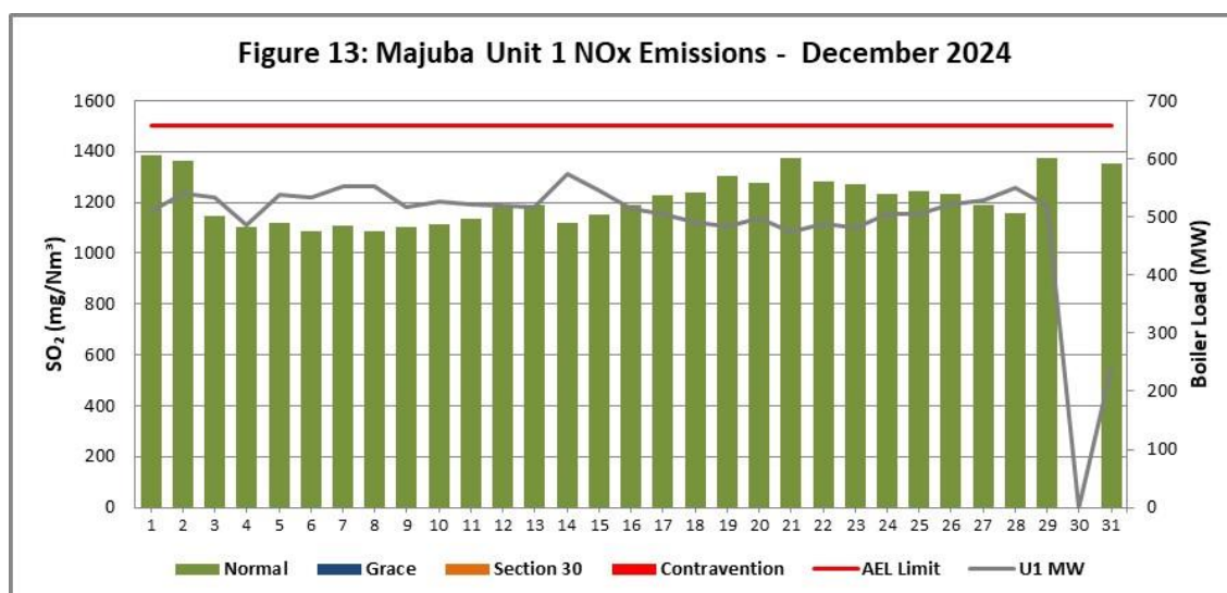
Figure 13. NO x emissions (daily averages) for the month of December 2024 against emission limit for Unit 1.
