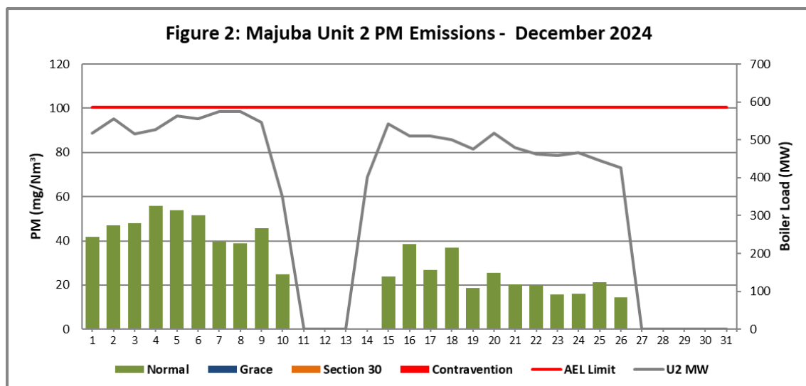
Figure 2. Particulate Matter emissions (daily averages) for the month of December 2024 against emission limit for Unit 2.
