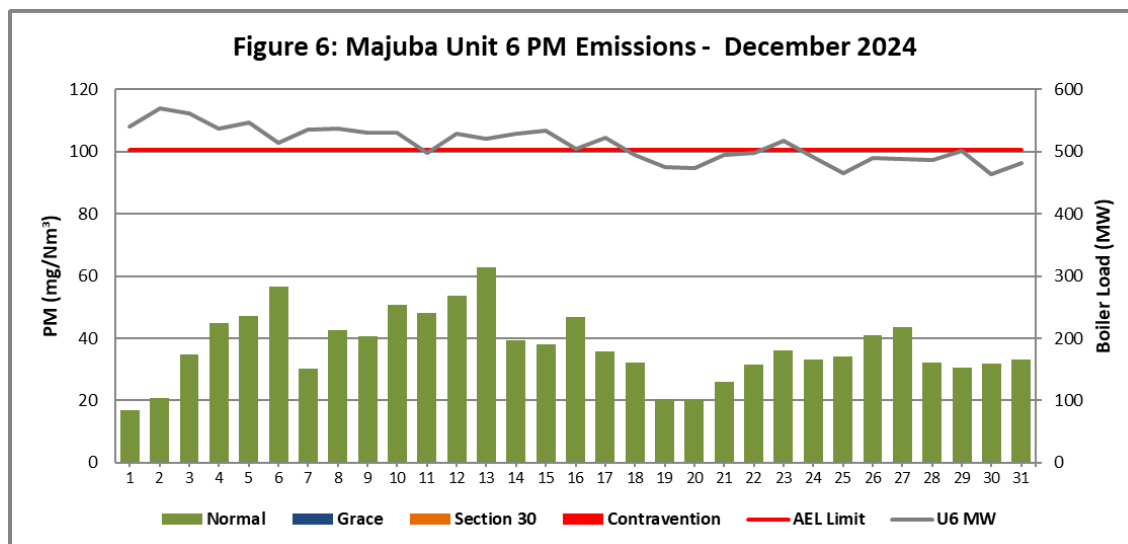
Figure 6. Particulate Matter emissions (daily averages) for the month of December 2024 against emission limit for Unit 6.
