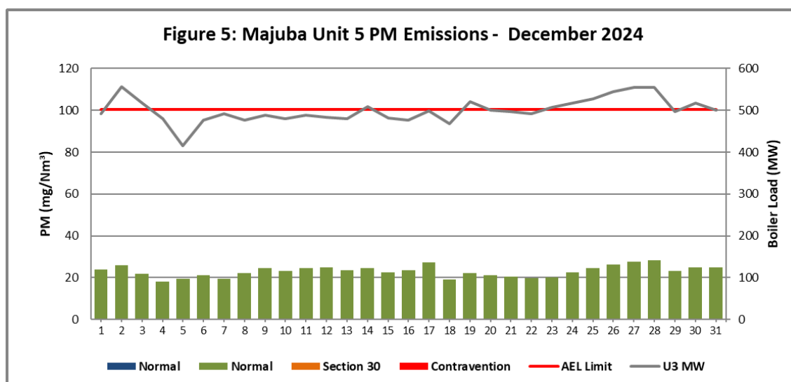
Figure 5. Particulate Matter emissions (daily averages) for the month of December 2024 against emission limit for Unit 5.
