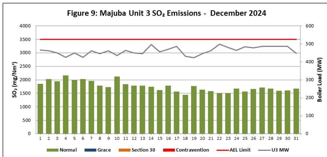
Figure 9. SO 2 emissions (daily averages) for the month of December 2024 against emission limit for Unit 3.
