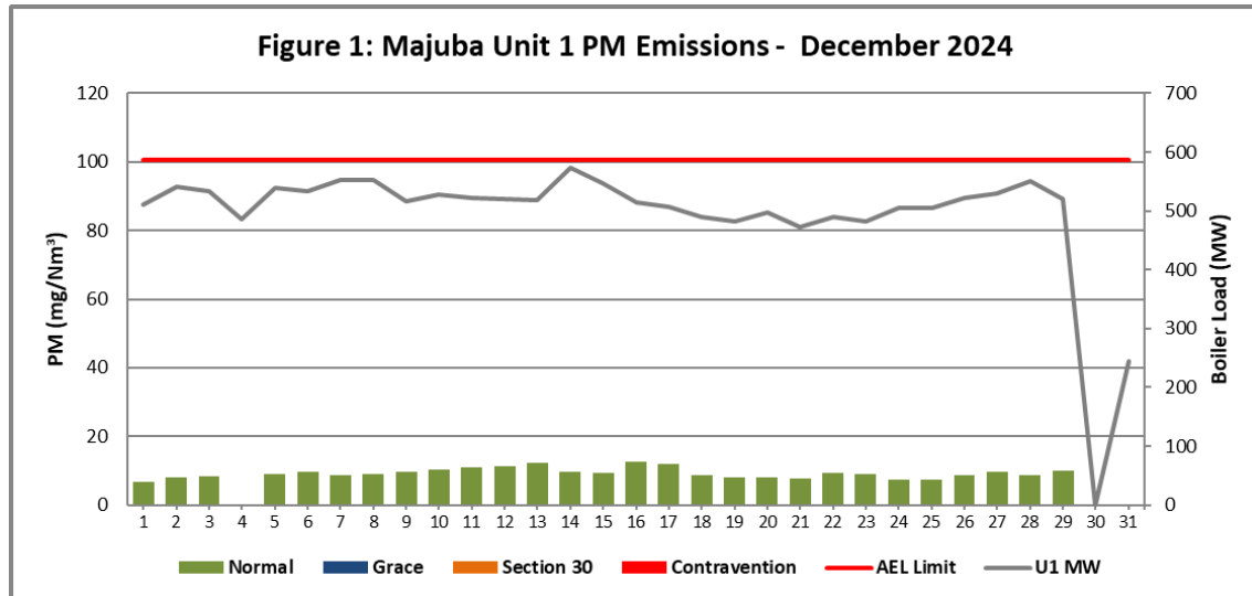
Figure 1. Particulate Matter emissions (daily averages) for the month of December 2024 against emission limit for Unit 1.
