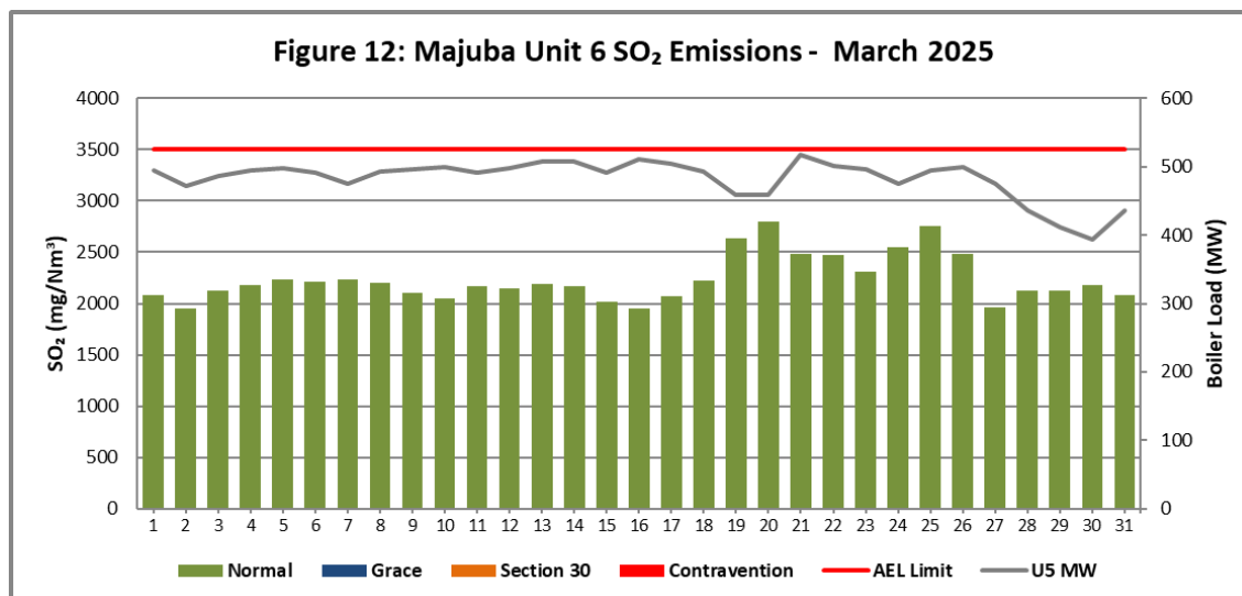
Figure 12. SO 2 emissions (daily averages) for the month of March 2025 against emission limit for Unit 6.
