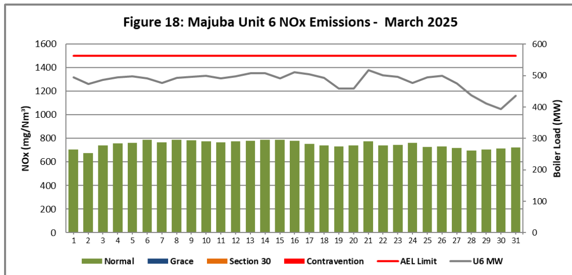
Figure 18. NO x emissions (daily averages) for the month March 2025 against emission limit for Unit 6
