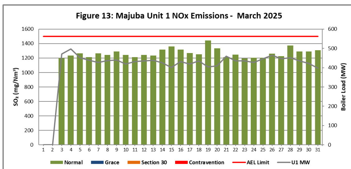
Figure 13. NO x emissions (daily averages) for the month of March 2025 against emission limit for Unit 1.
