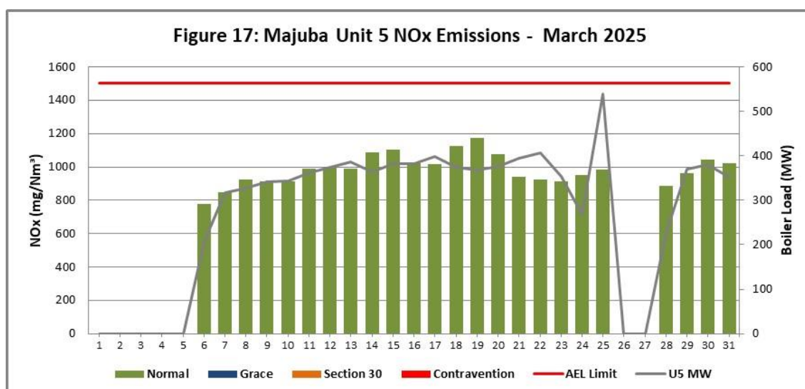
Figure 17. NOx emissions (daily averages) for the month of March 2025 against emission limit for Unit 5
