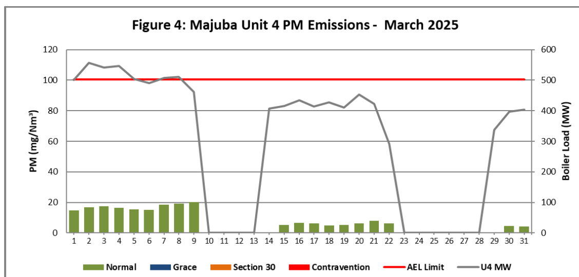
Figure 4. Particulate Matter emissions (daily averages) for the month of March 2025 against emission limit for Unit 4.
