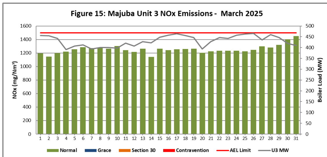
Figure 15. NOx emissions (daily averages) for the month of March 2025 against emission limit for Unit 3.
