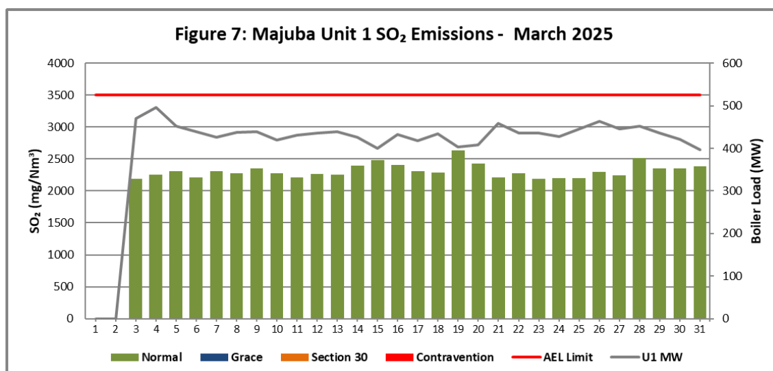
Figure 7. SO₂ emissions (daily averages) for the month of March 2025 against emission limit for Unit 1.
