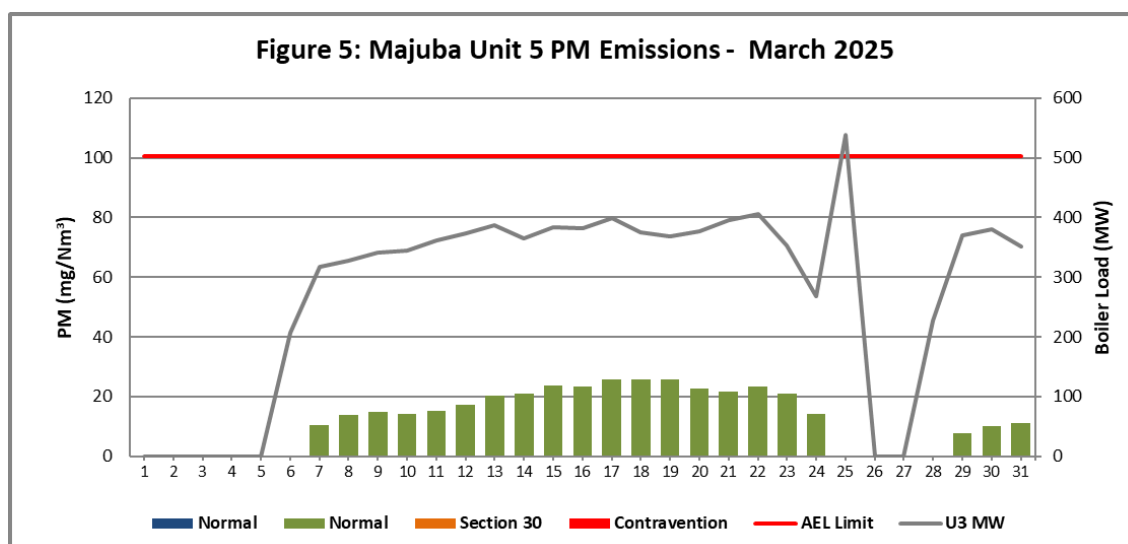
Figure 5. Particulate Matter emissions (daily averages) for the month of March 2025 against emission limit for Unit 5.
