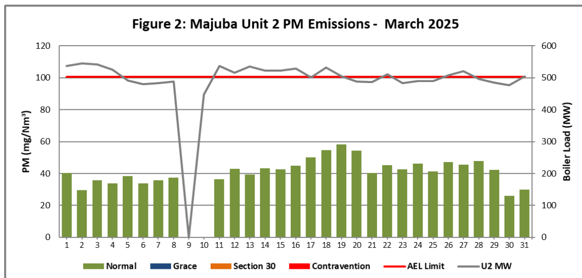
Figure 2. Particulate Matter emissions (daily averages) for the month of March 2025 against emission limit for Unit 2.
