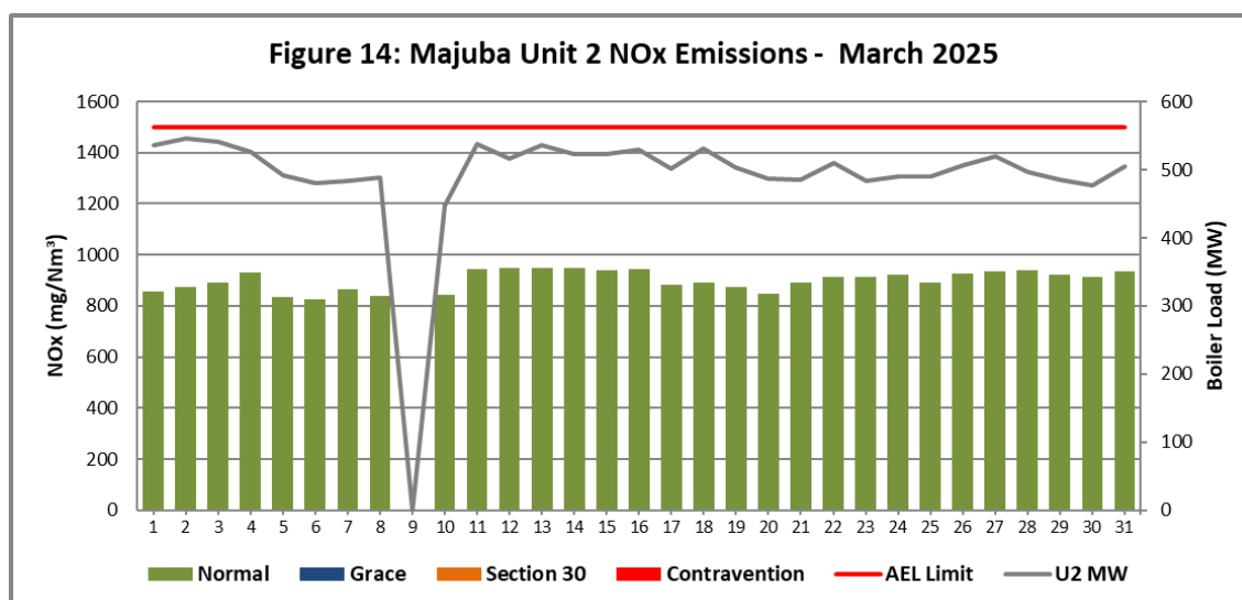
Figure 14. NO x emissions (daily averages) for the month of March 2025 against emission limit for Unit 2.
