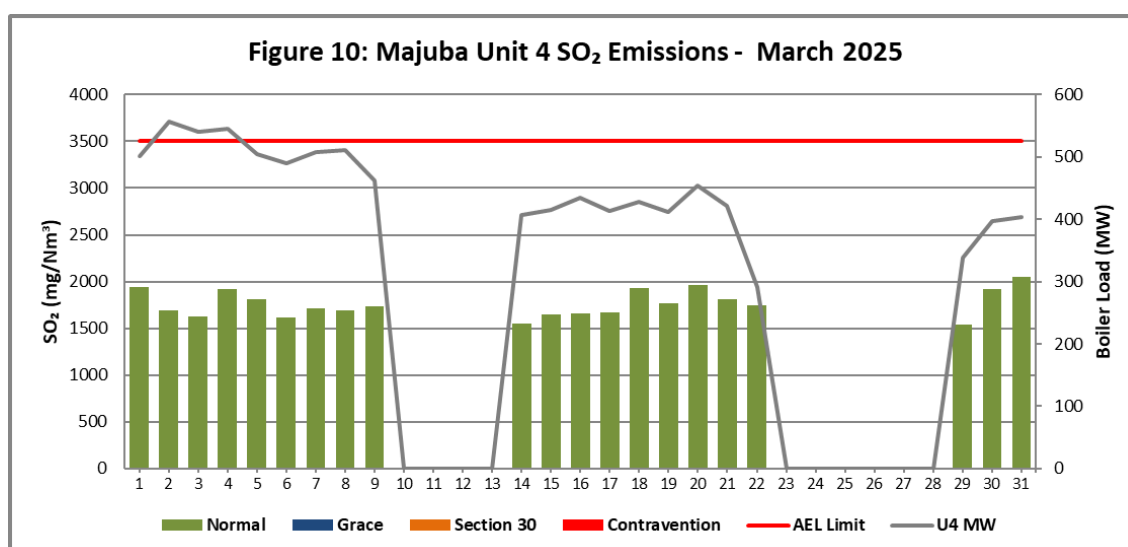
Figure 10. SO 2 emissions (daily averages) for the month of March 2025 against emission limit for Unit 4.
