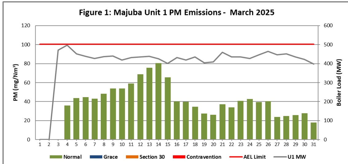
Figure 1. Particulate Matter emissions (daily averages) for the month of March 2025 against emission limit for Unit 1.
