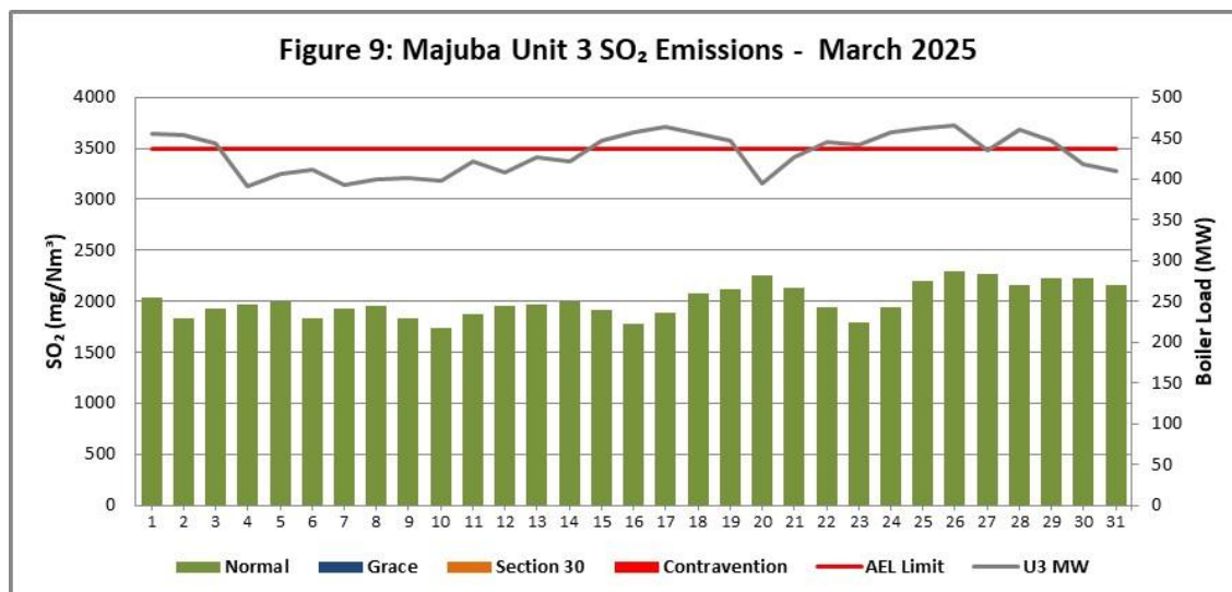
Figure 9. SO 2 emissions (daily averages) for the month of March 2025 against emission limit for Unit 3.
