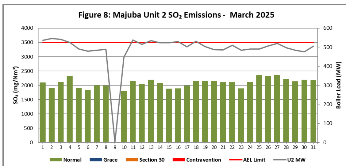
Figure 8. SO₂ emissions (daily averages) for the month of March 2025 against emission limit for Unit 2.
