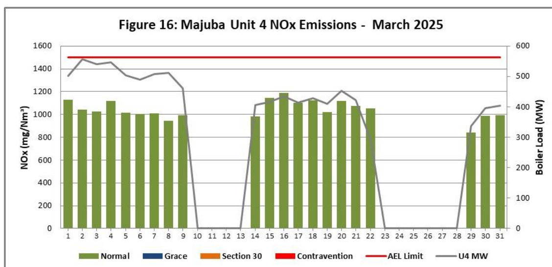
Figure 16. NOx emissions (daily averages) for the month of March 2025 against emission limit for Unit 4
