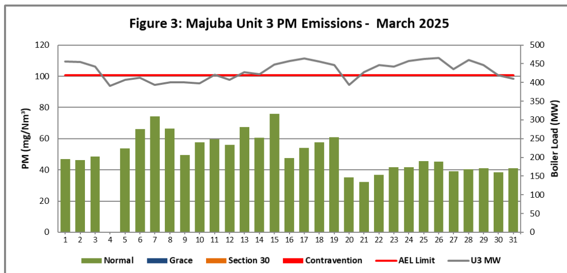
Figure 3. Particulate Matter emissions (daily averages) for the month of March 2025 against emission limit for Unit 3.
