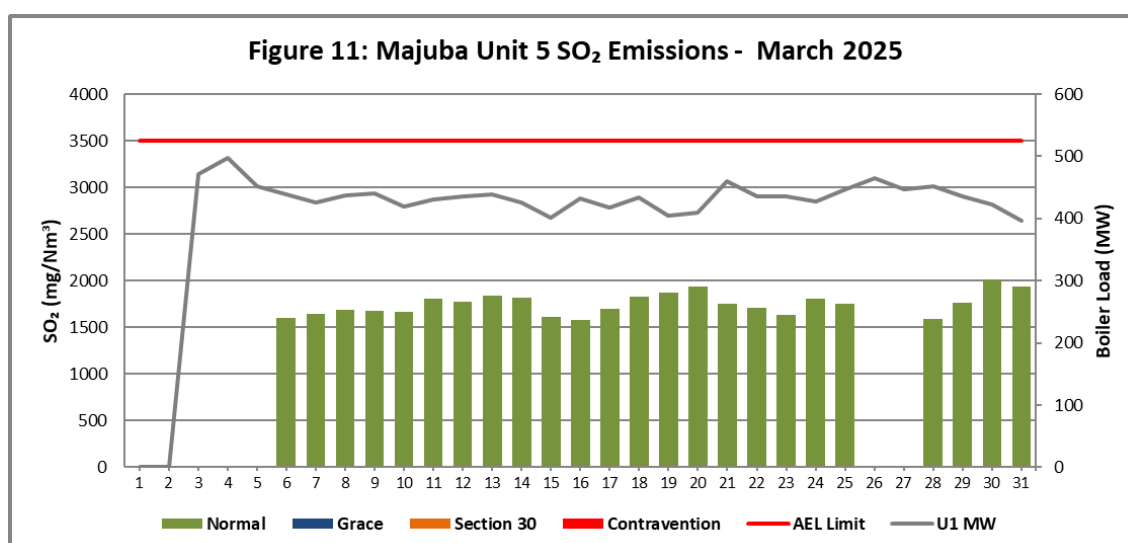
Figure 11. SO 2 emissions (daily averages) for the month of March 2025 against emission limit for Unit 5.
