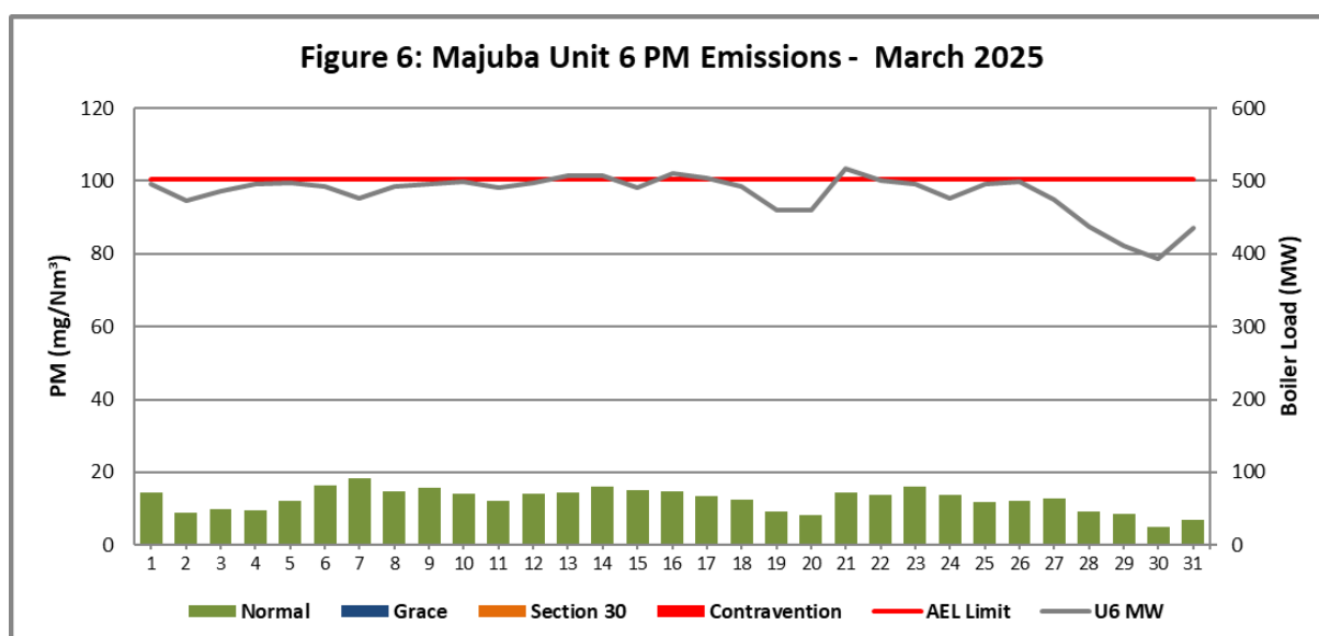
Figure 6. Particulate Matter emissions (daily averages) for the month of March 2025 against emission limit for Unit 6.
