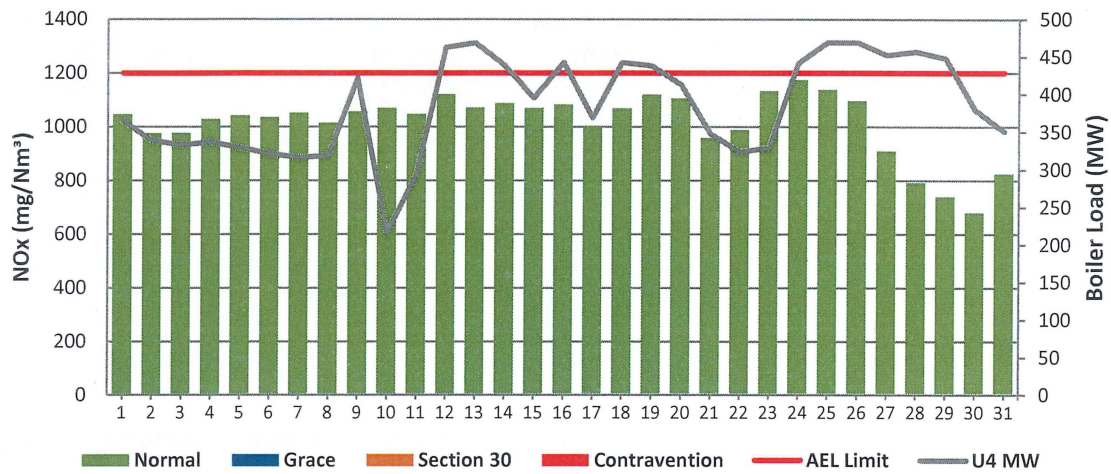
Figure 16: Tutuka Unit 4 NOx Emissions - January 2025
