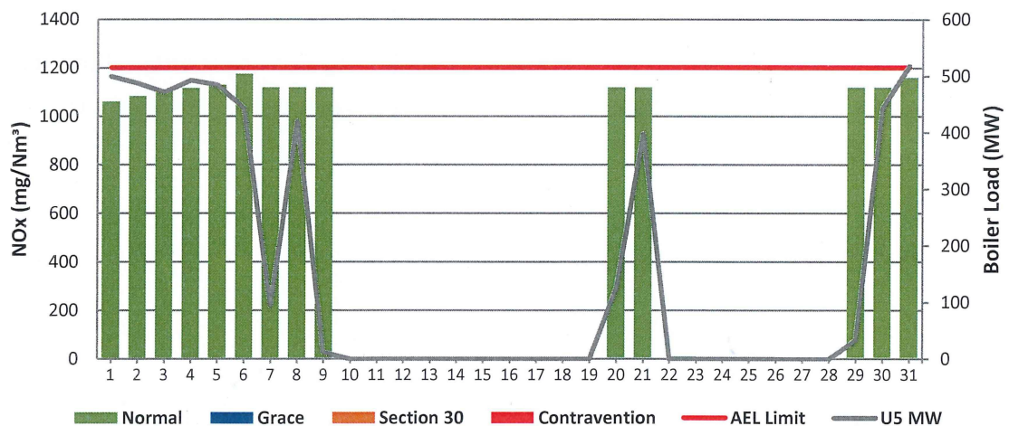
Figure 17: Tutuka Unit 5 NOx Emissions - January 2025
