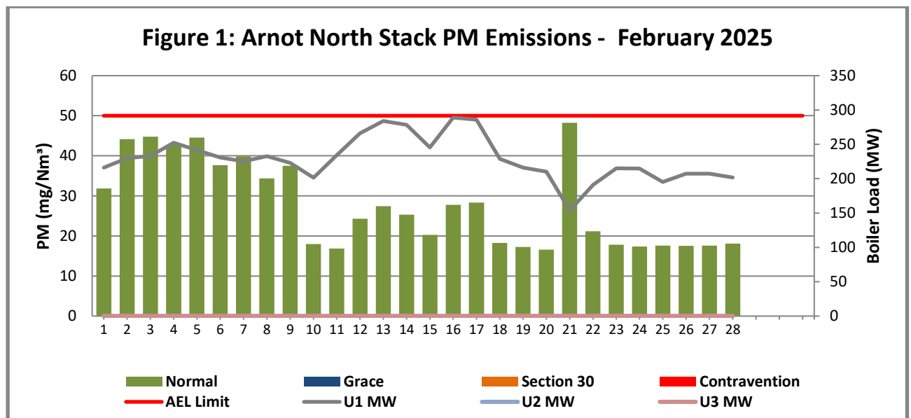
Figure 1: PM emissions (daily averages) for the month of February 2025 against the emission limit for the North Stack
