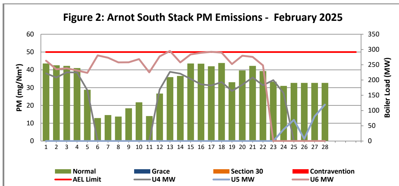
Figure 2: PM emissions (daily averages) for the month of February 2025 against emission limit for the South Stack
