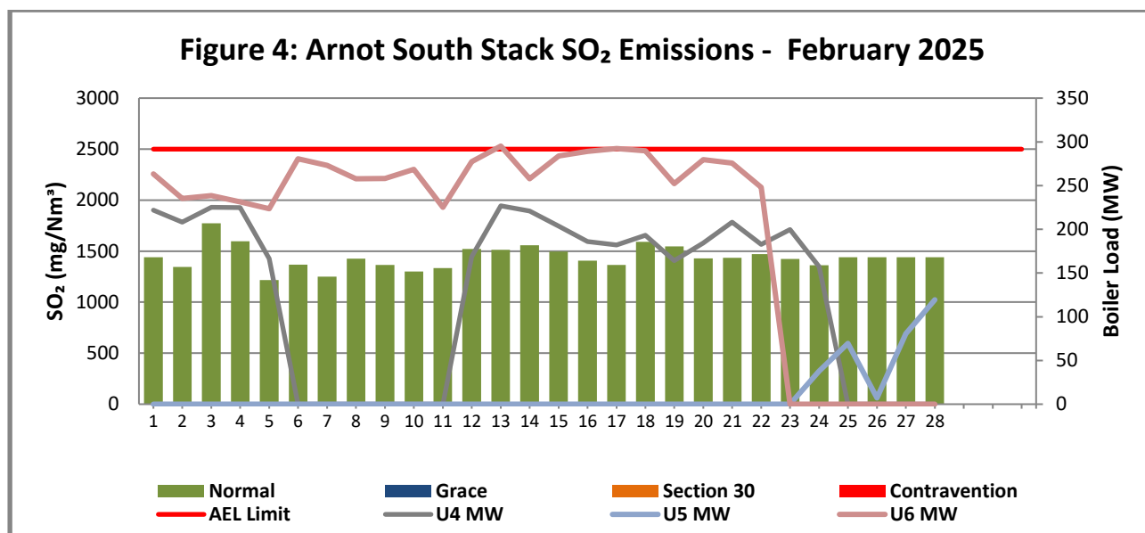
Figure 4: SO 2 emissions (daily averages) for the month of February 2025 against emission limit for the South Stack
