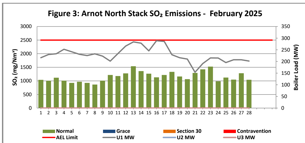
Figure 3: SO 2 emissions (daily averages) for the month of February 2025 against emission limit for the North Stack
