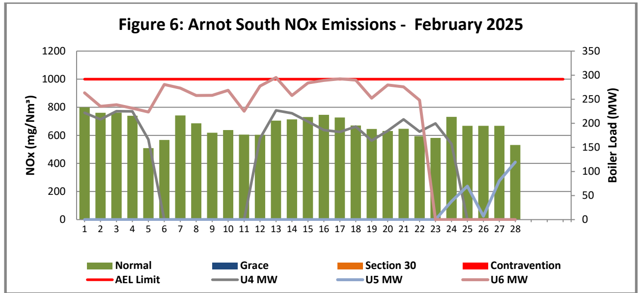
Figure 6: NO 2 emissions (daily averages) for the month of February 2025 against emission limit for the South Stack
