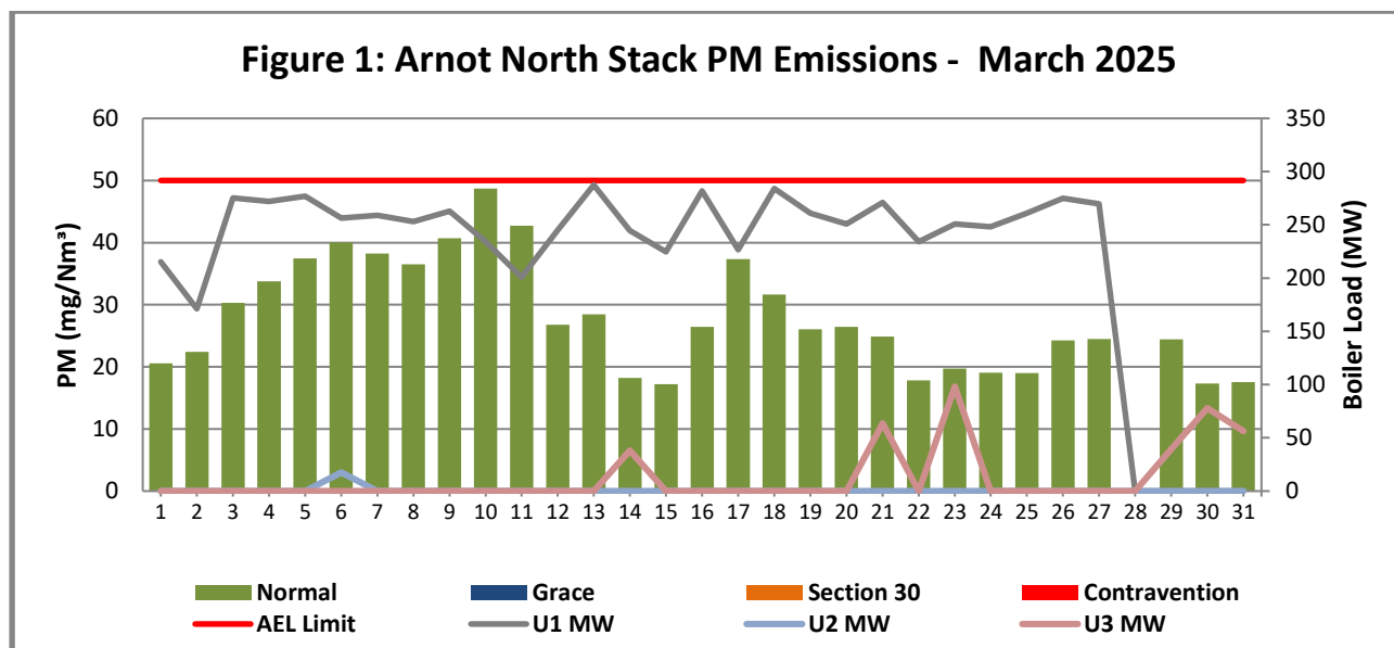
Figure 1: PM emissions (daily averages) for the month of March 2025 against the emission limit for the North Stack
