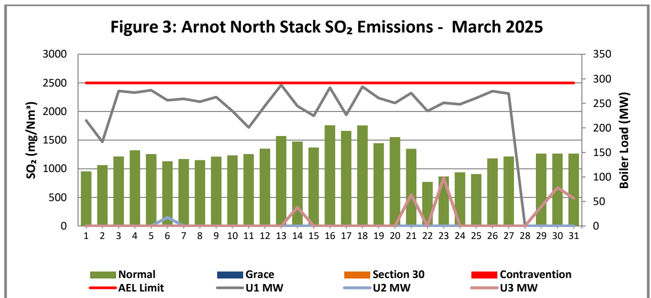
Figure 3: SO 2 emissions (daily averages) for the month of March 2025 against emission limit for the North Stack
