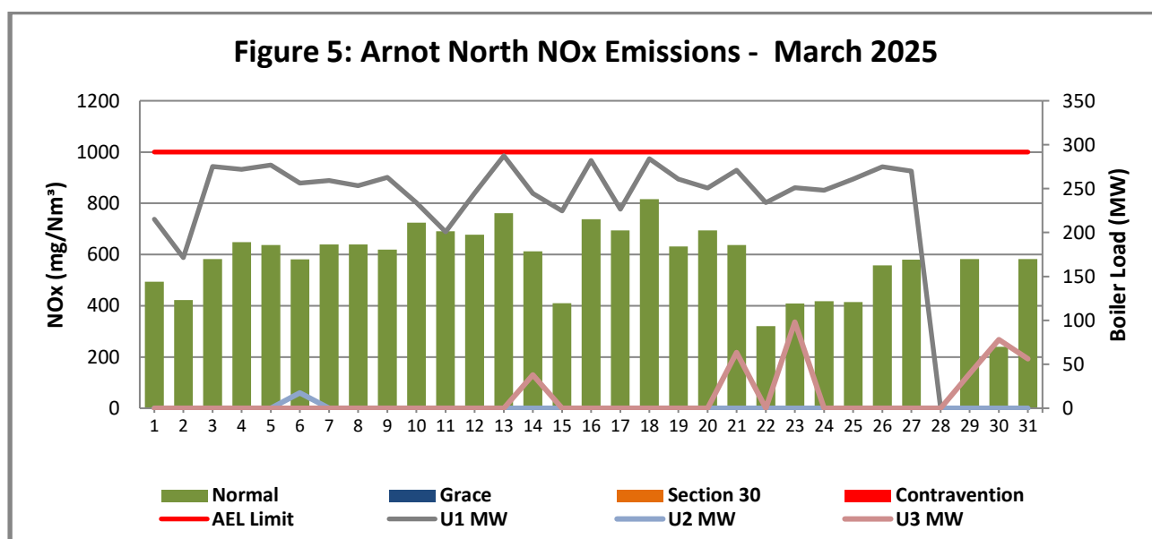
Figure 5: NO 2 emissions (daily averages) for the month of March 2025 against emission limit for the North Stack
