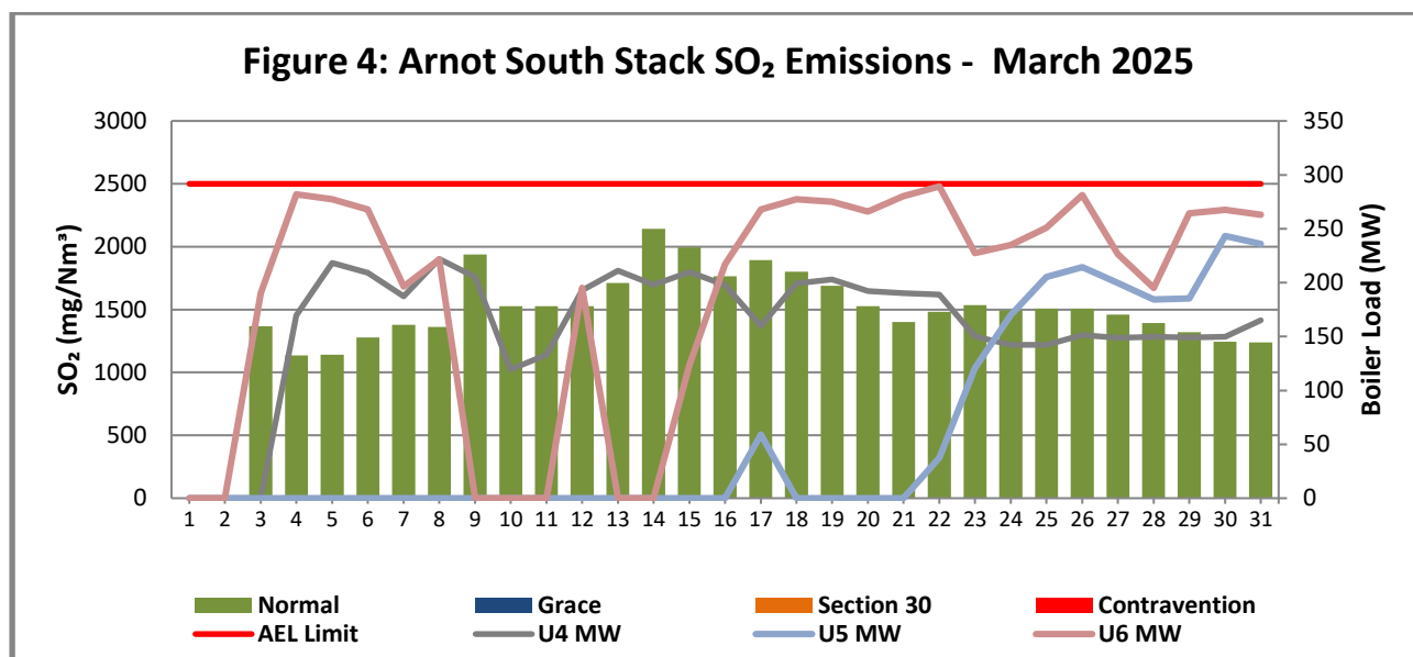
Figure 4: SO 2 emissions (daily averages) for the month of March 2025 against emission limit for the South Stack
