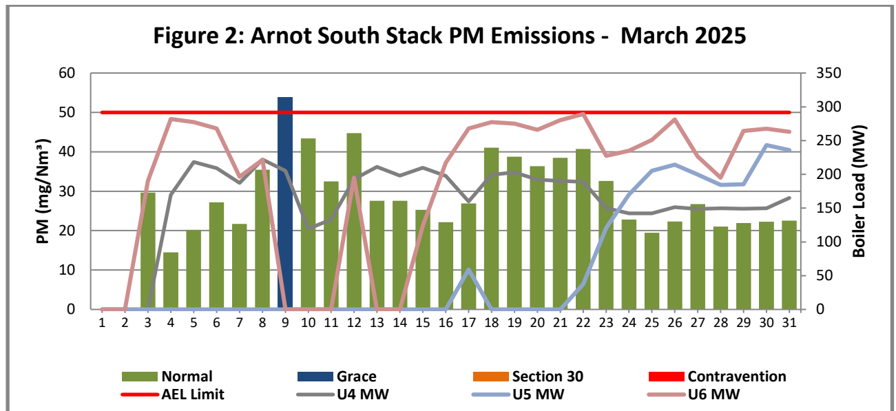
Figure 2: PM emissions (daily averages) for the month of March 2025 against emission limit for the South Stack
