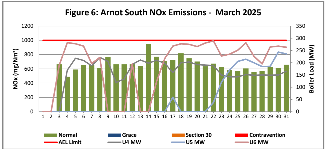
Figure 6: NO 2 emissions (daily averages) for the month of March 2025 against emission limit for the South Stack
