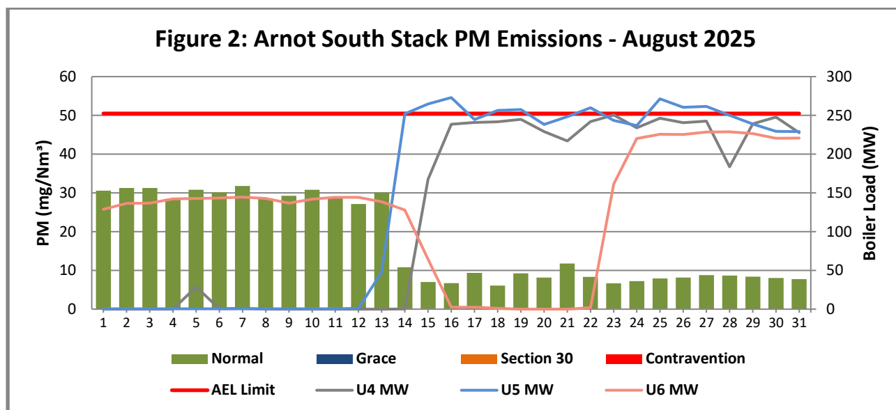
Figure 2: PM emissions (daily averages) for the month of August 2025 against emission limit for the South Stack
