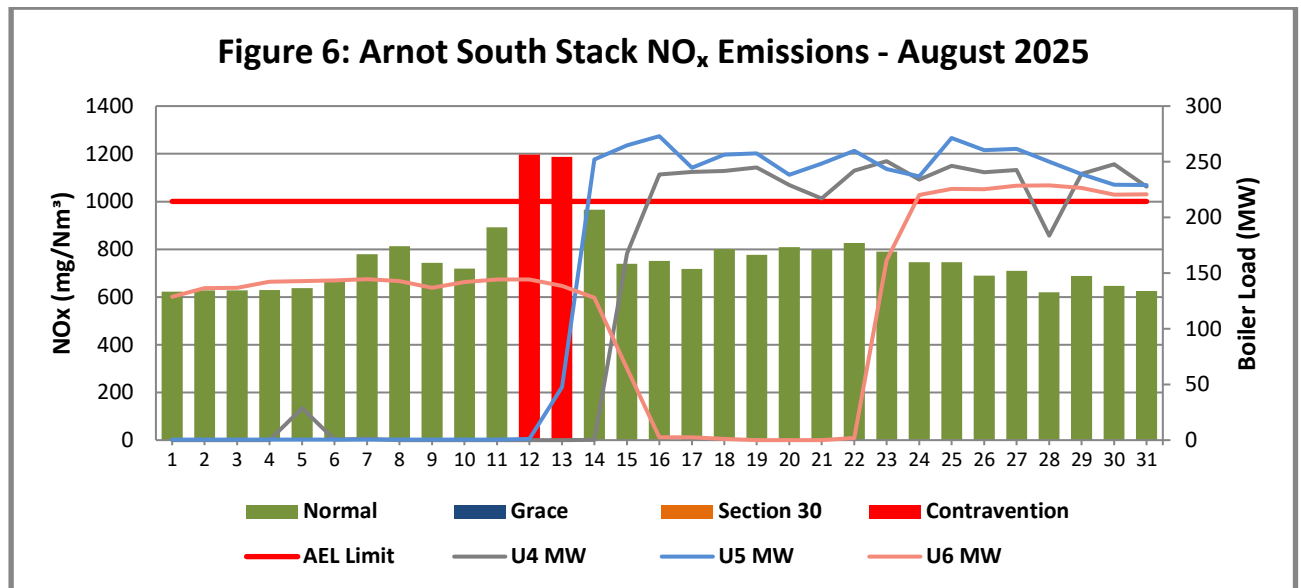
Figure 6: NO 2 emissions (daily averages) for the month of August 2025 against emission limit for the South Stack
