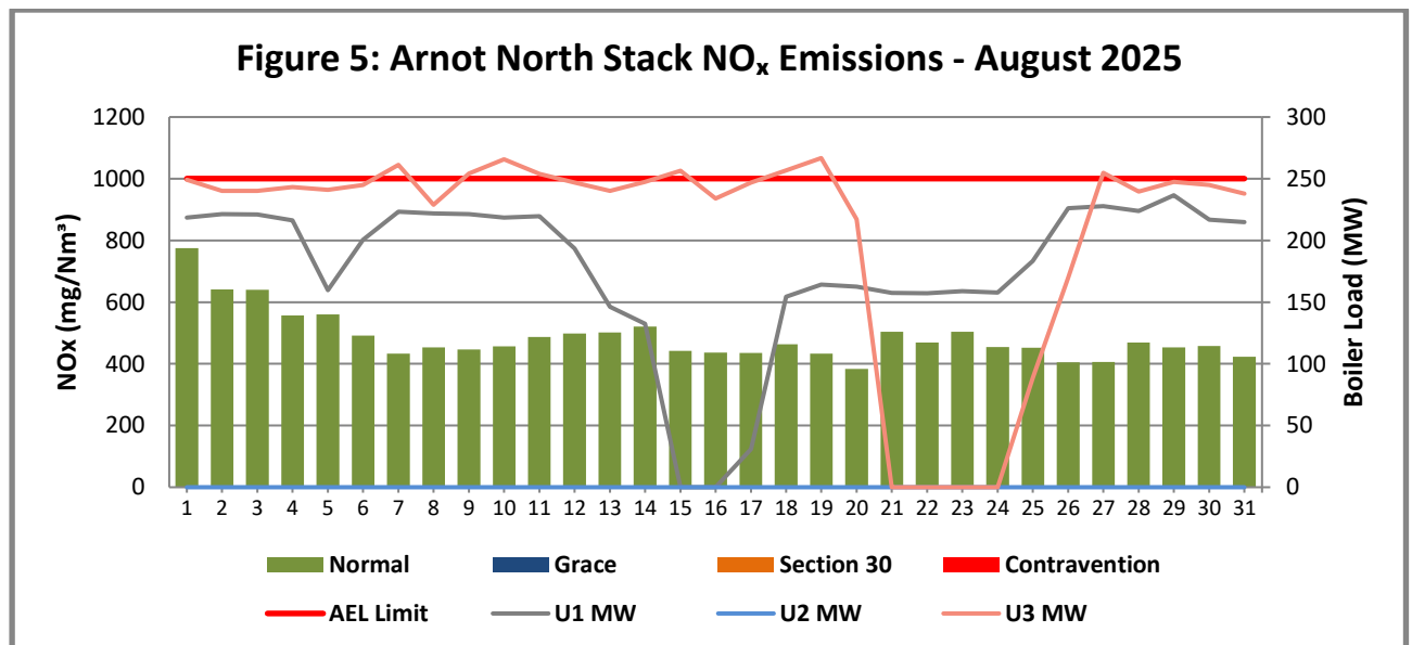
Figure 5: NO 2 emissions (daily averages) for the month of August 2025 against emission limit for the North Stack
