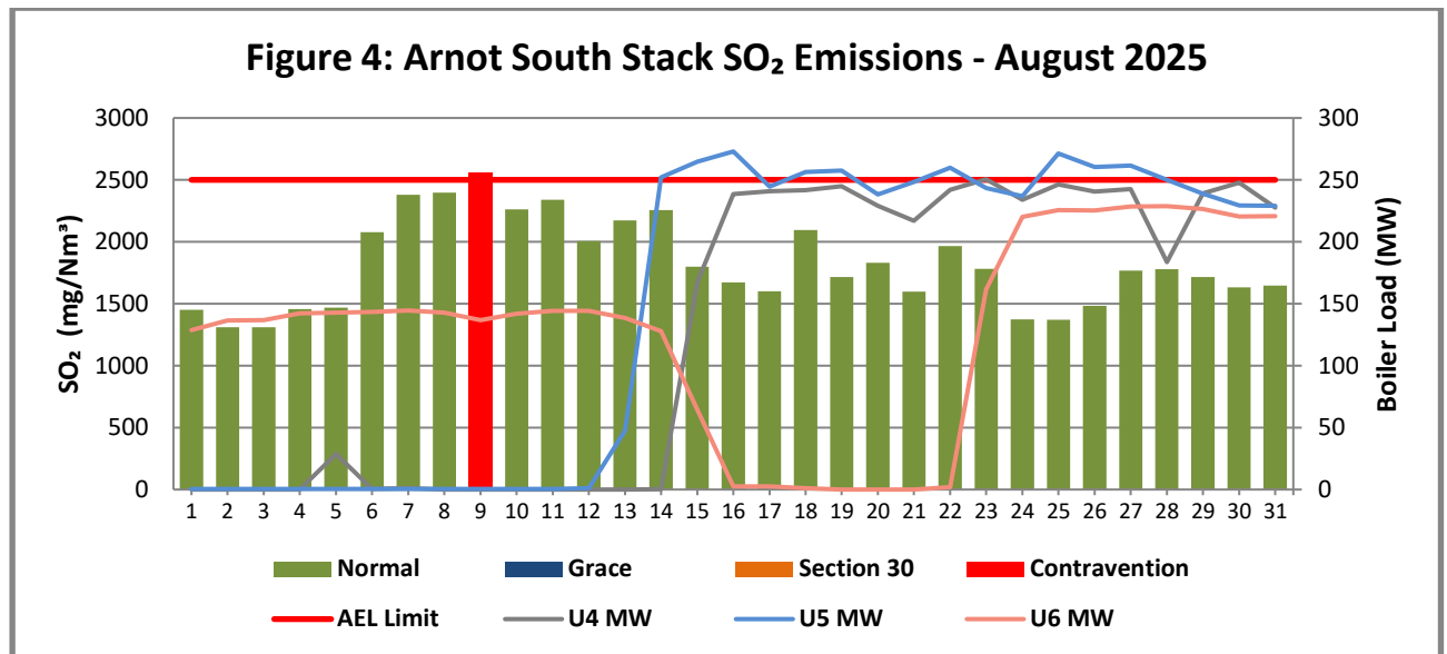
Figure 4: SO 2 emissions (daily averages) for the month of August 2025 against emission limit for the South Stack
