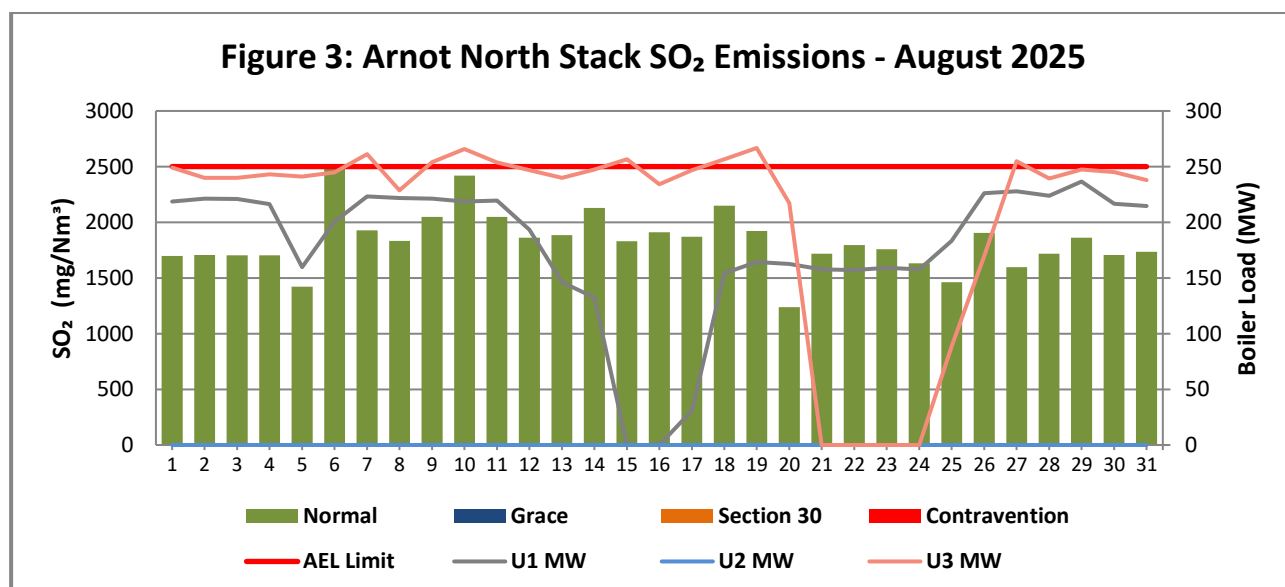
Figure 3: SO 2 emissions (daily averages) for the month of August 2025 against emission limit for the North Stack
