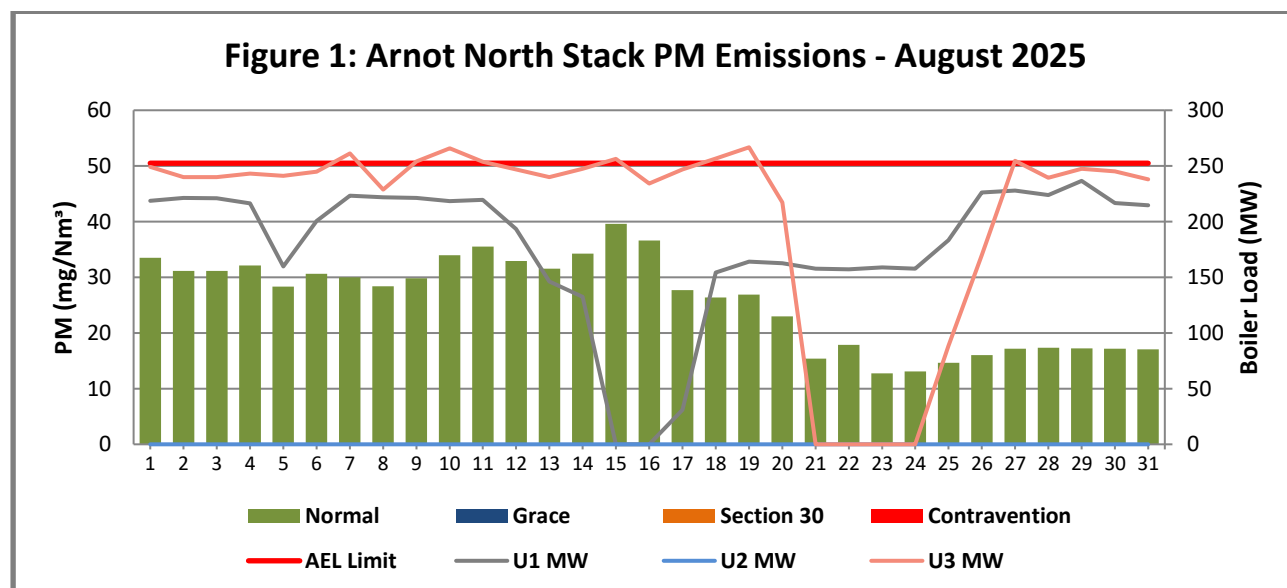
Figure 1: PM emissions (daily averages) for the month of August 2025 against the emission limit for the North Stack
