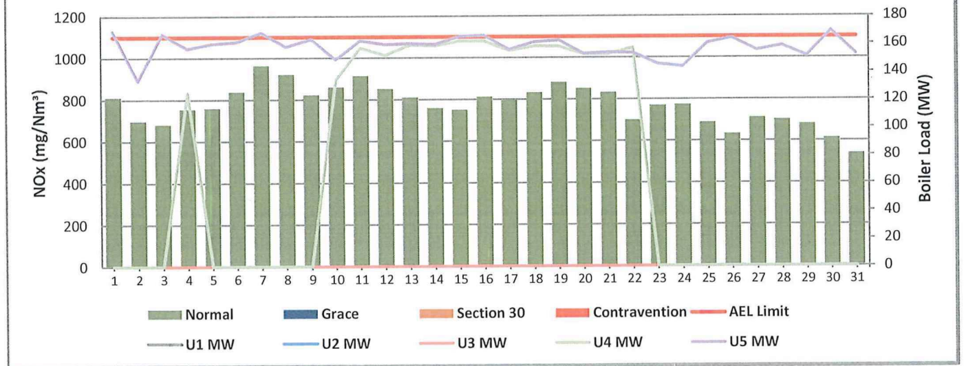
Figure 5: Hendrina North Stack NO x Emissions - August 2025
