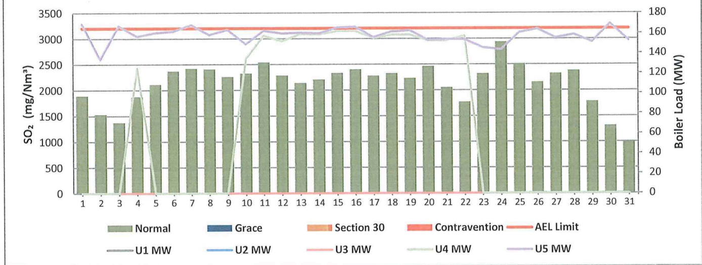
Figure 3: Hendrina North Stack SO 2 Emissions - August 2025
