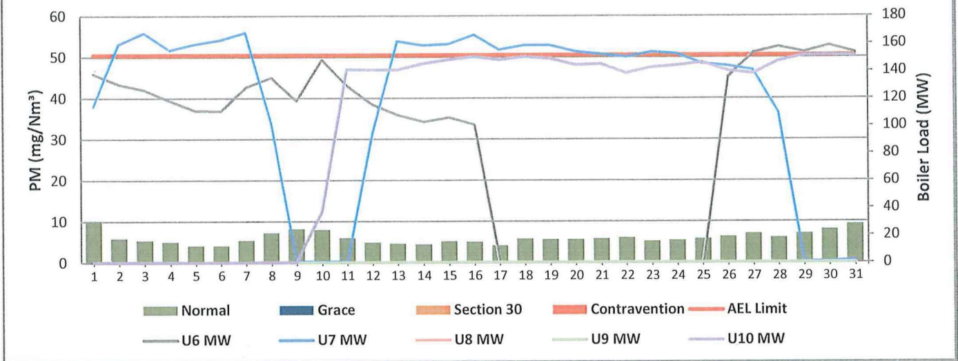
Figure 2: Hendrina South Stack PM Emissions - August 2025
