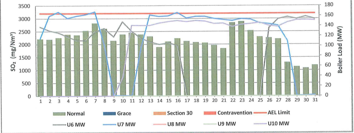
Figure 4: Hendrina South Stack SO 2 Emissions - August 2025
