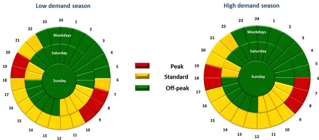
Figure 2: WEPS, Megaflex, Megaflex Gen, Miniflex, Homeflex, Ruraflex and Ruraflex Gen: low and high demand seasons TOU periods
