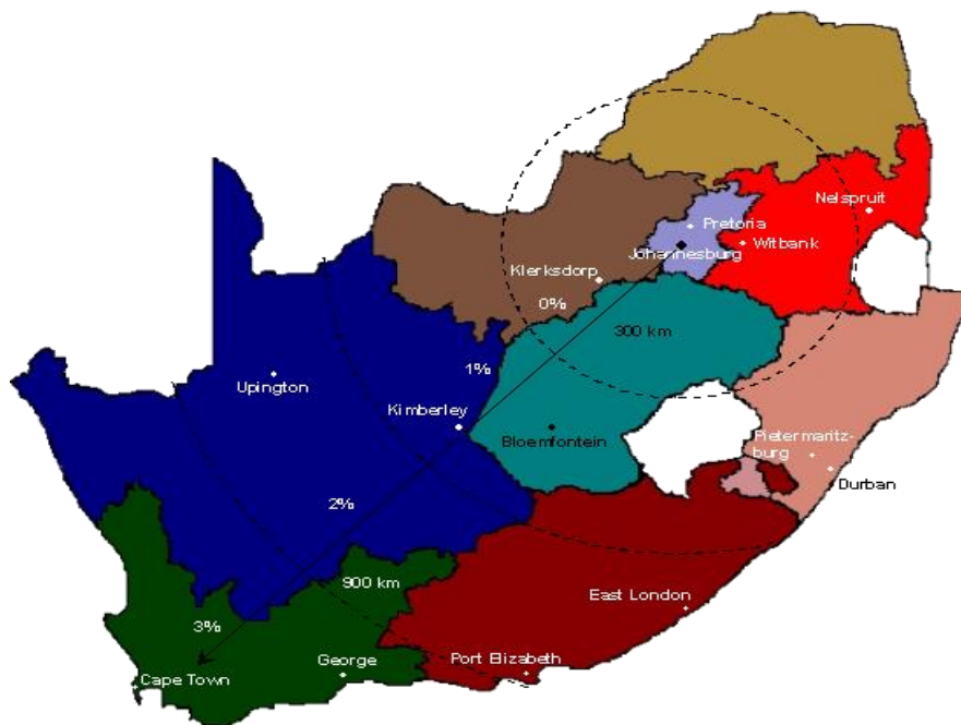
Figure 1: Transmission zones for loads
