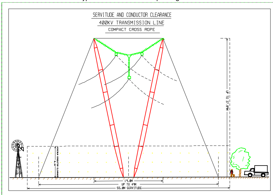
Figure 8 : Diagrammatic representation of the compact cross-rope suspension tower configuration
