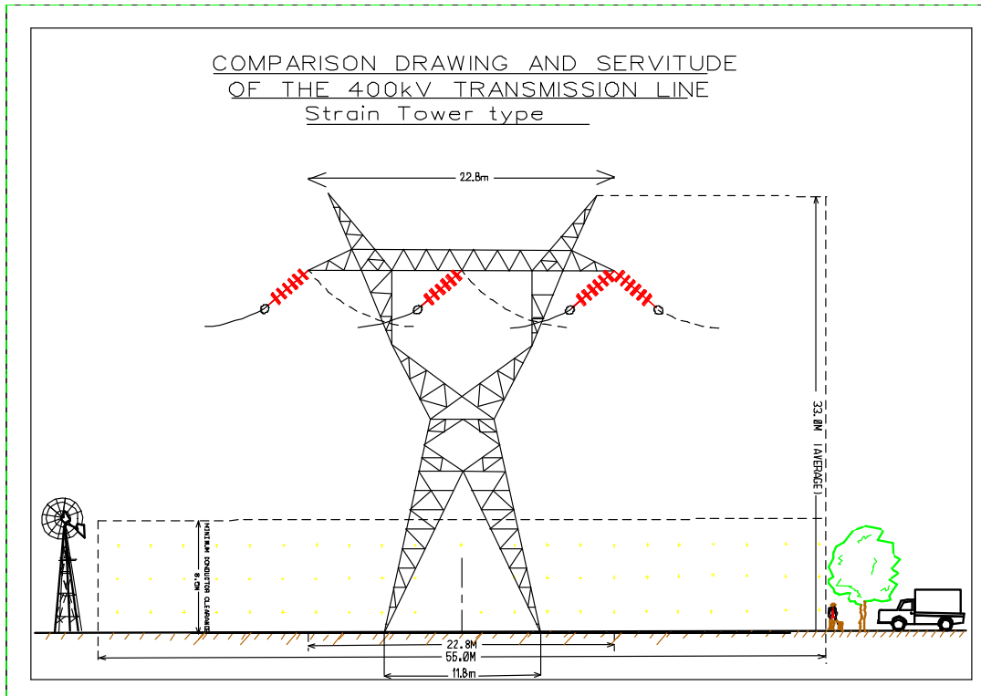
Figure 10 : Diagrammatic representation of the self supporting strain tower configuration
