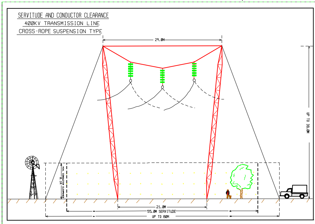
Figure 9 : Diagrammatic representation of the cross-rope suspension tower configuration
