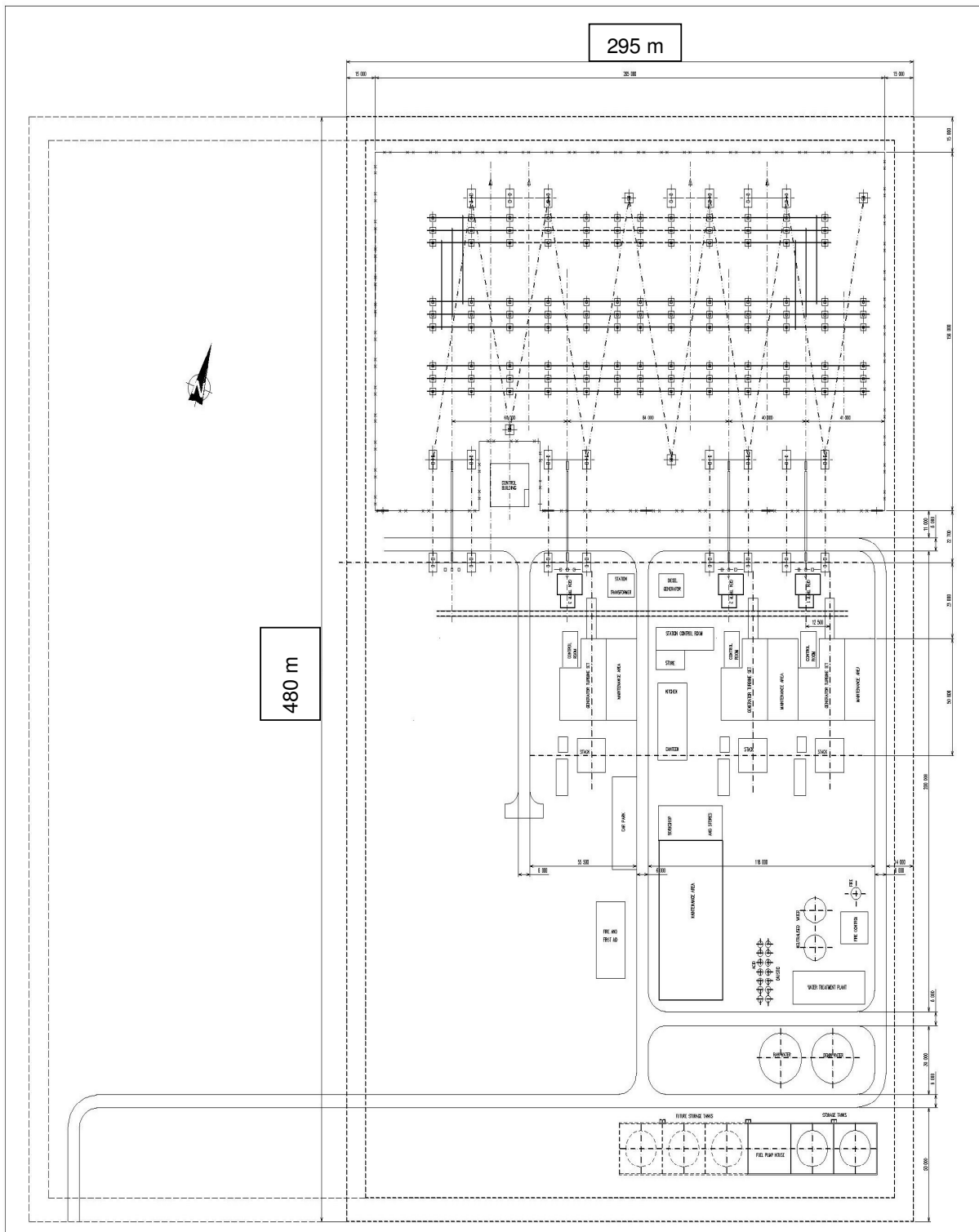
Figure 6 : Site layout plan for OCGT and transmission substation
