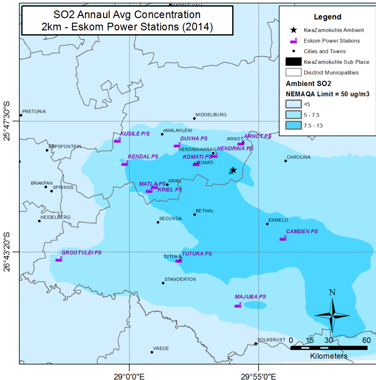
Figure 15: Annual average SO 2 concentrations (µg/m 3 ) resulting from SO 2 emissions from all Eskom’s coal-fired power stations in Mpumalanga.
