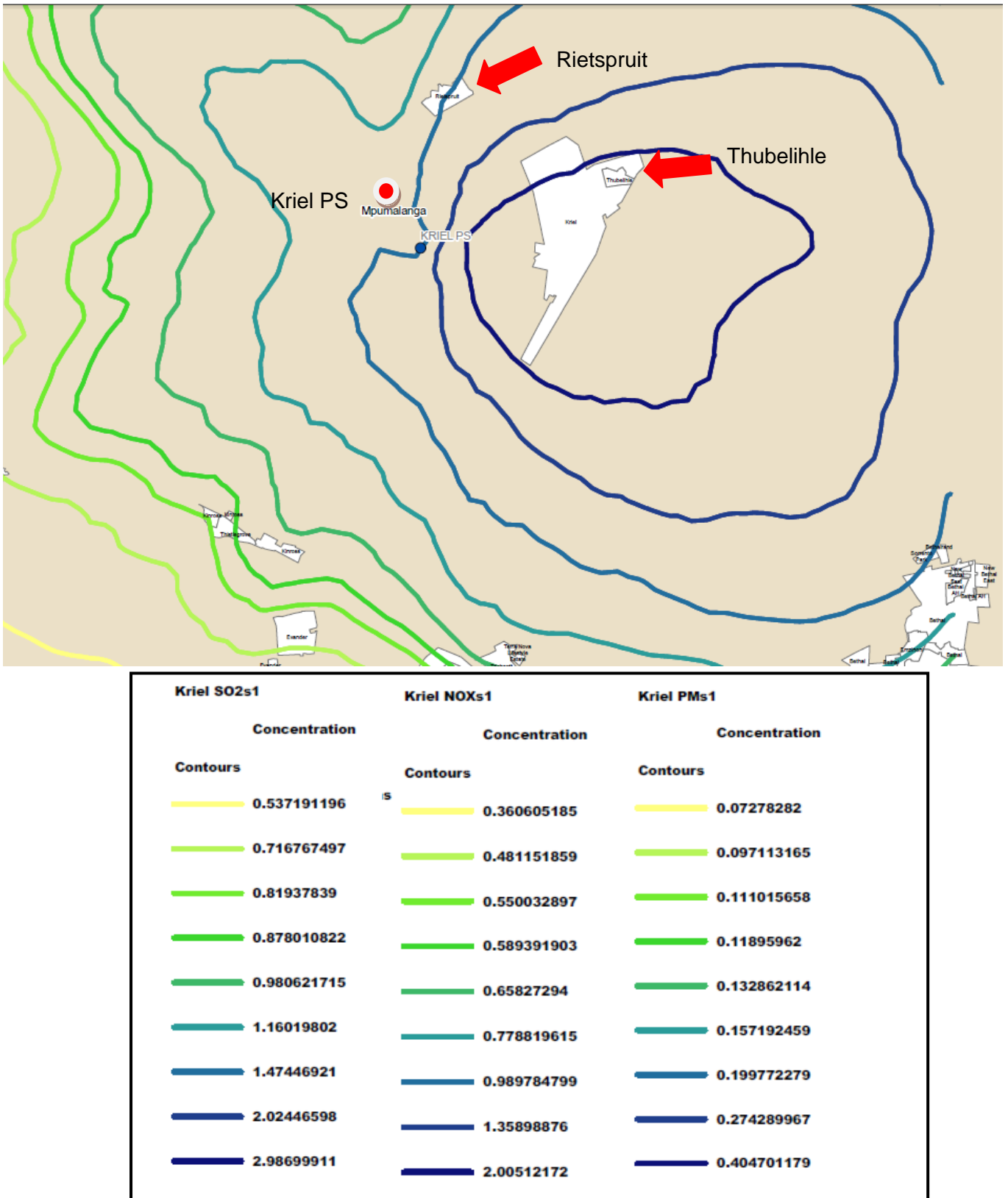
Figure 11: Area of impact of Kriel Power Station’s emissions (annual average concentrations in \mu\text{g}/\text{m}^3 from uMoya-NILU, 2014d), and locations of Thubelihle and Rietspruit
