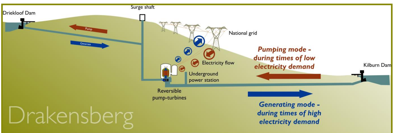
Operation of Drakensberg Pumped Storage Scheme
