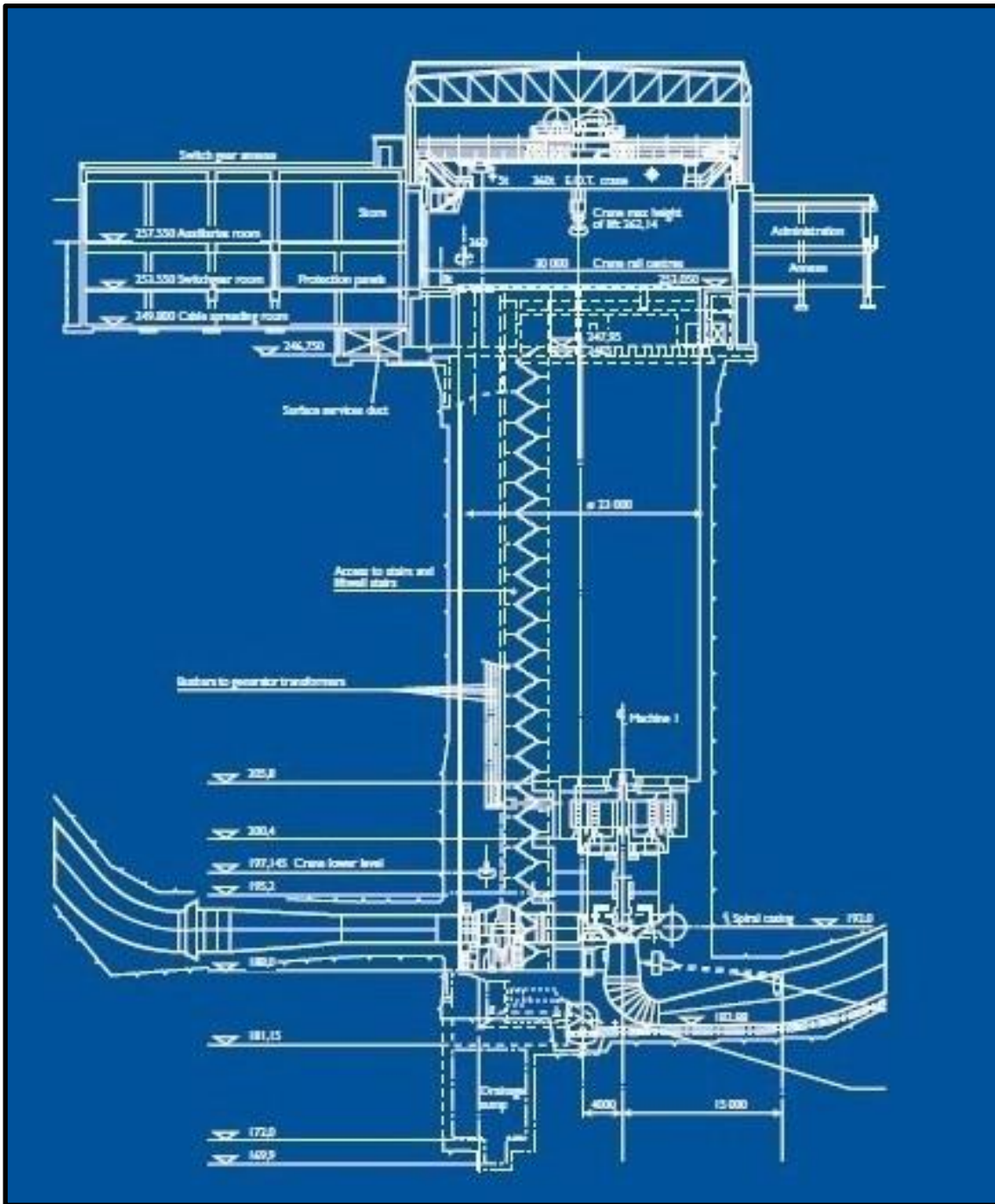
Machine Shaft
