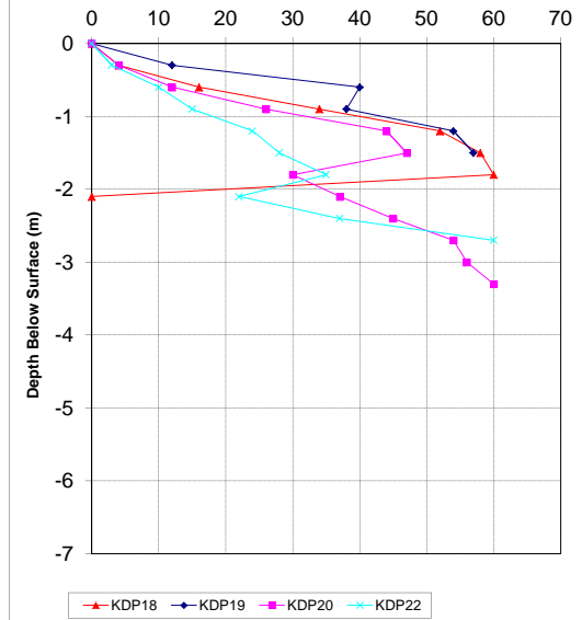
Koeberg DPSH Plots (5 of 6)
