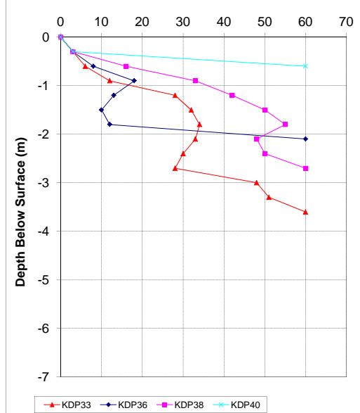
Koeberg DPSH Plots (5 of 6)
