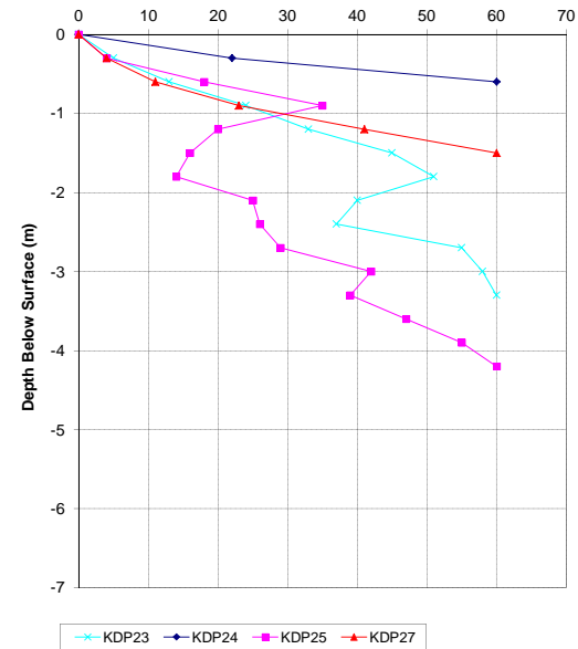
Koeberg DPSH Plots (4 of 6)
