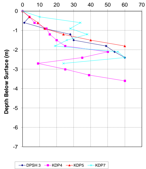
Koeberg DPSH Plots (4 of 6)
