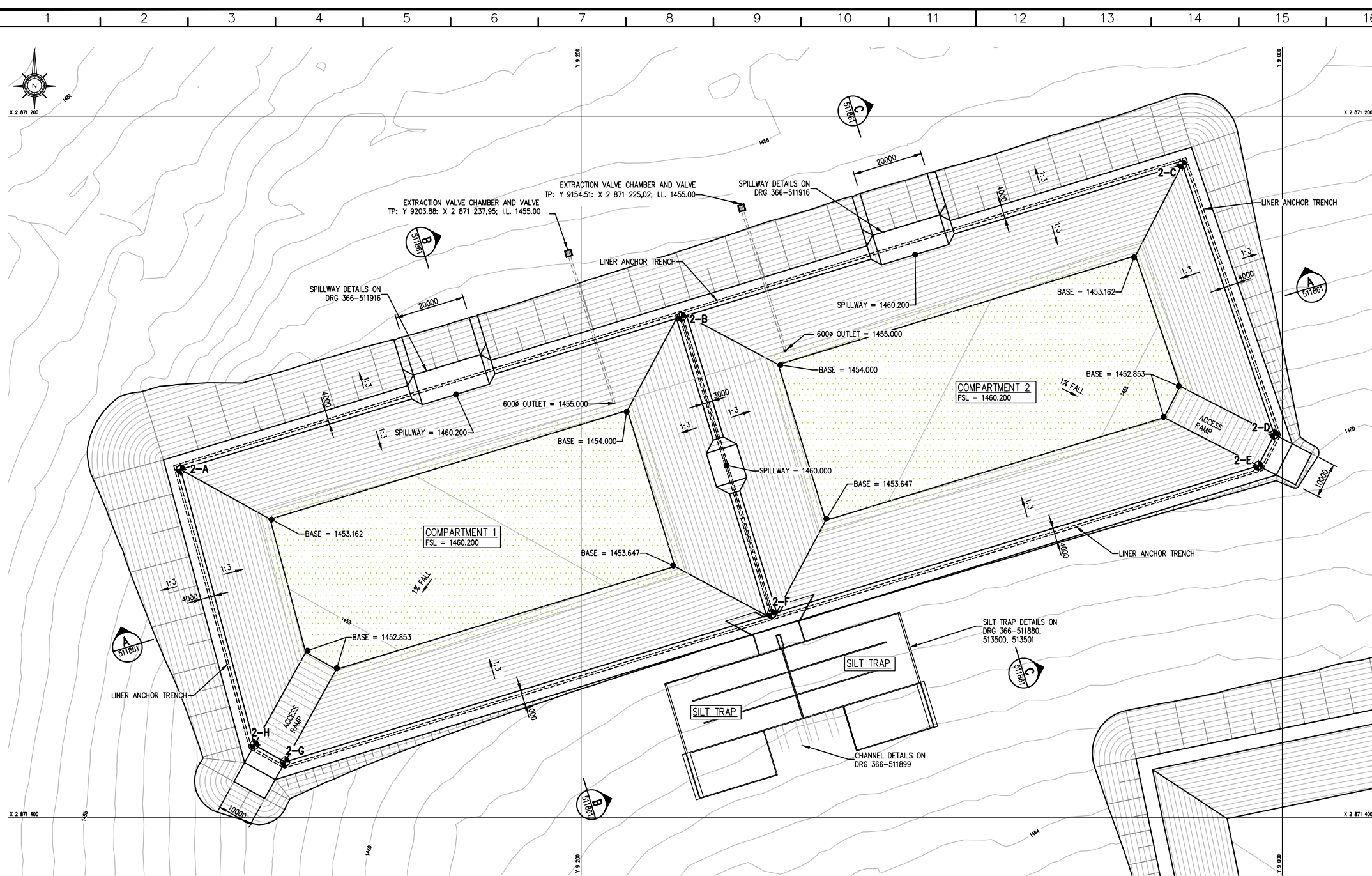
LAYOUT 1:500
