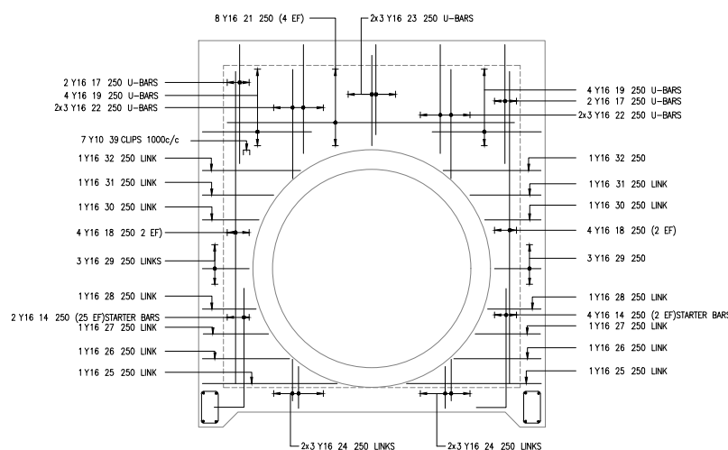
WALL 2 (250 THK) SCALE 1:100
