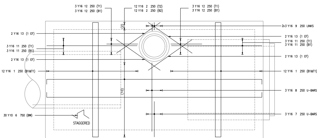
OUTLET CHAMBER ROOF LAYOUT SCALE 1:25
