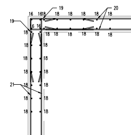
TYPICAL CORNER DETAIL
