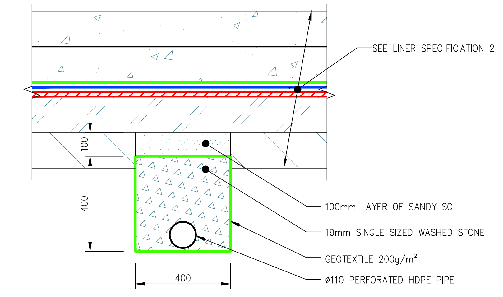
DETAIL 1 SCALE 1:10
