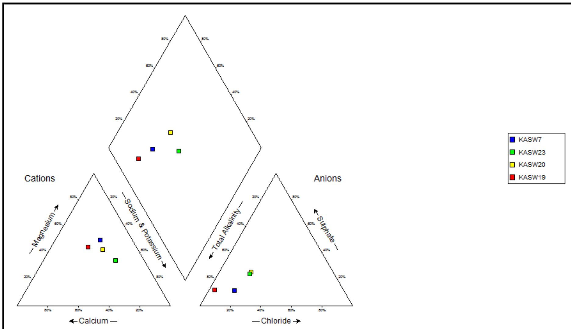
Figure 19: Piper diagram of the surface water samples
