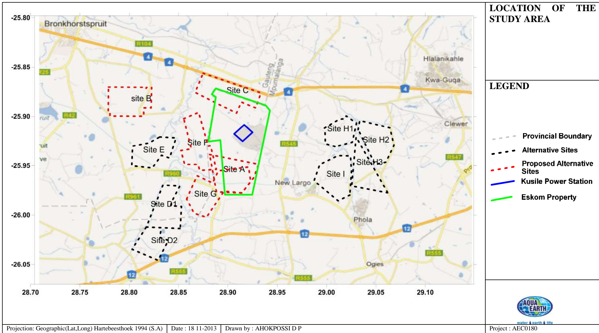
Figure 1: Locality map indicating possible ash dam disposal sites
