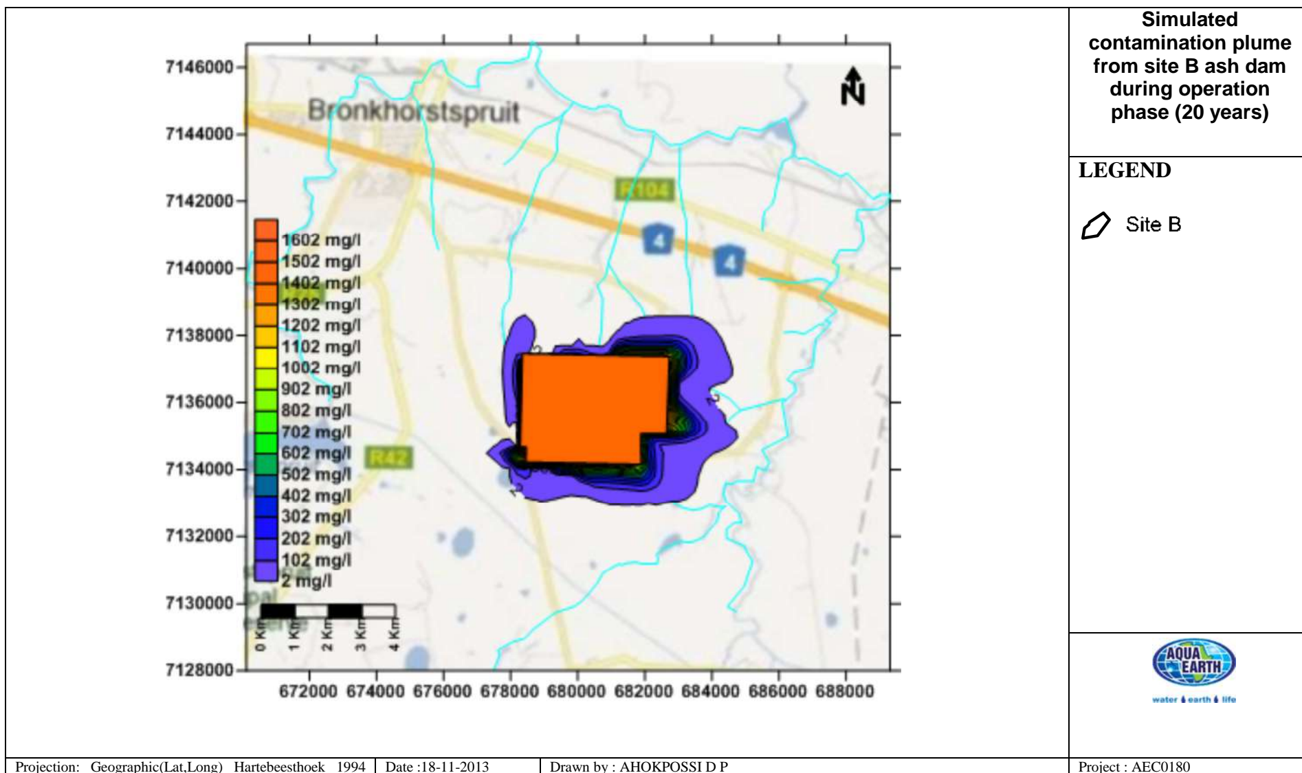
Figure 61: Simulated contamination plume from Alternative B ADF during operation phase (20 years)
