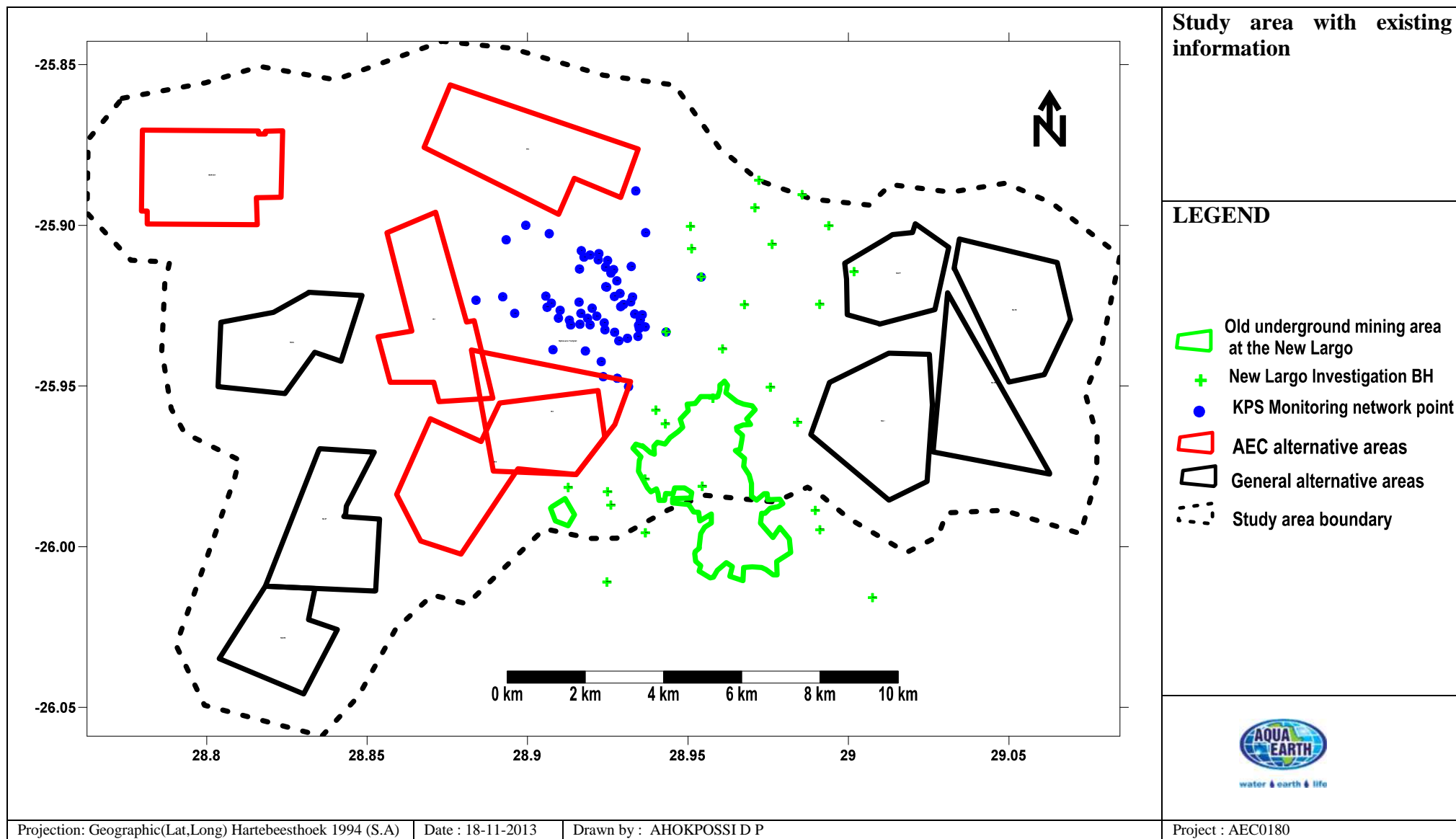
Figure 7: Location of existing geohydrological information in the study area
