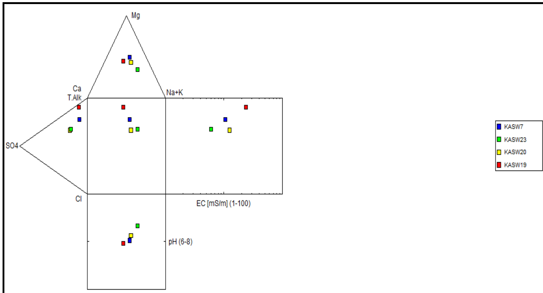
Figure 20: Expanded Durov diagram of the groundwater samples.
