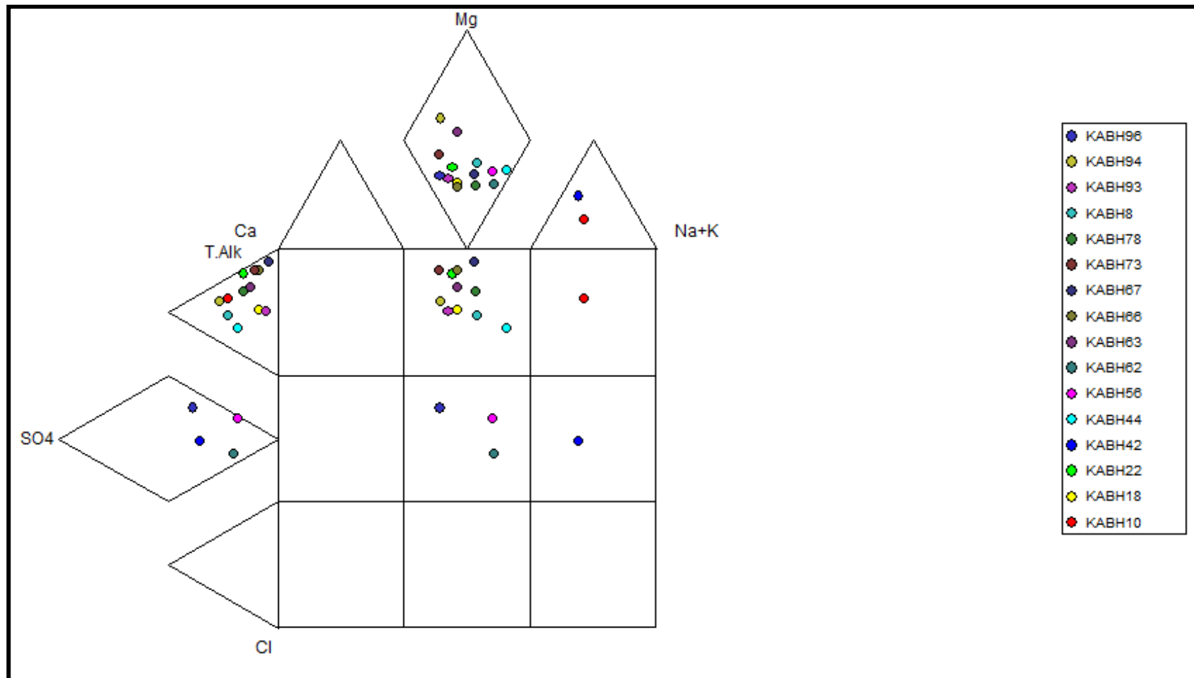
Figure 18 : Expanded Durov Diagram of the groundwater samples
