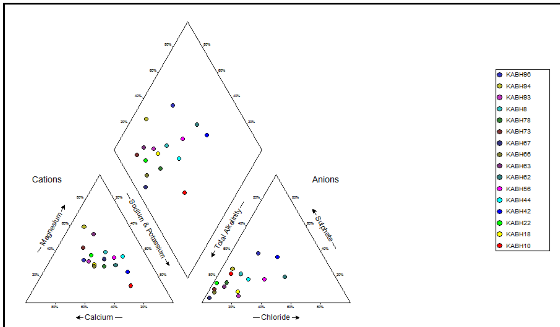
Figure 17: Piper diagram of the groundwater samples
