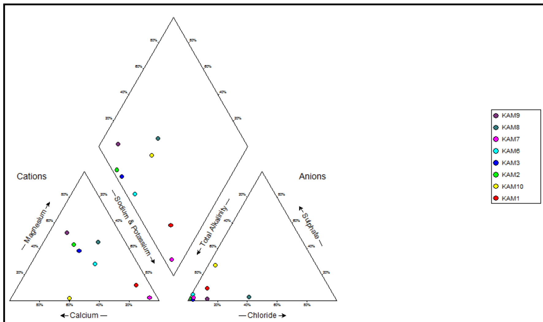
Figure 23: Piper diagram of the water quality collected from the new drilled boreholes
