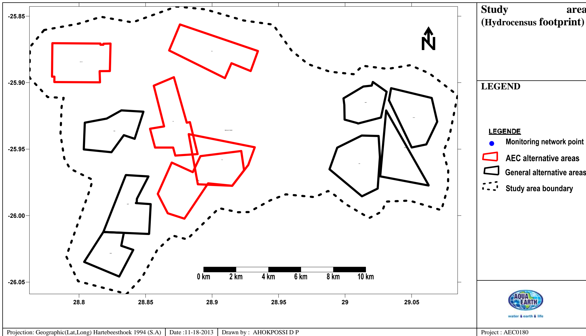
Figure 9: Plan showing hydrocensus footprint
