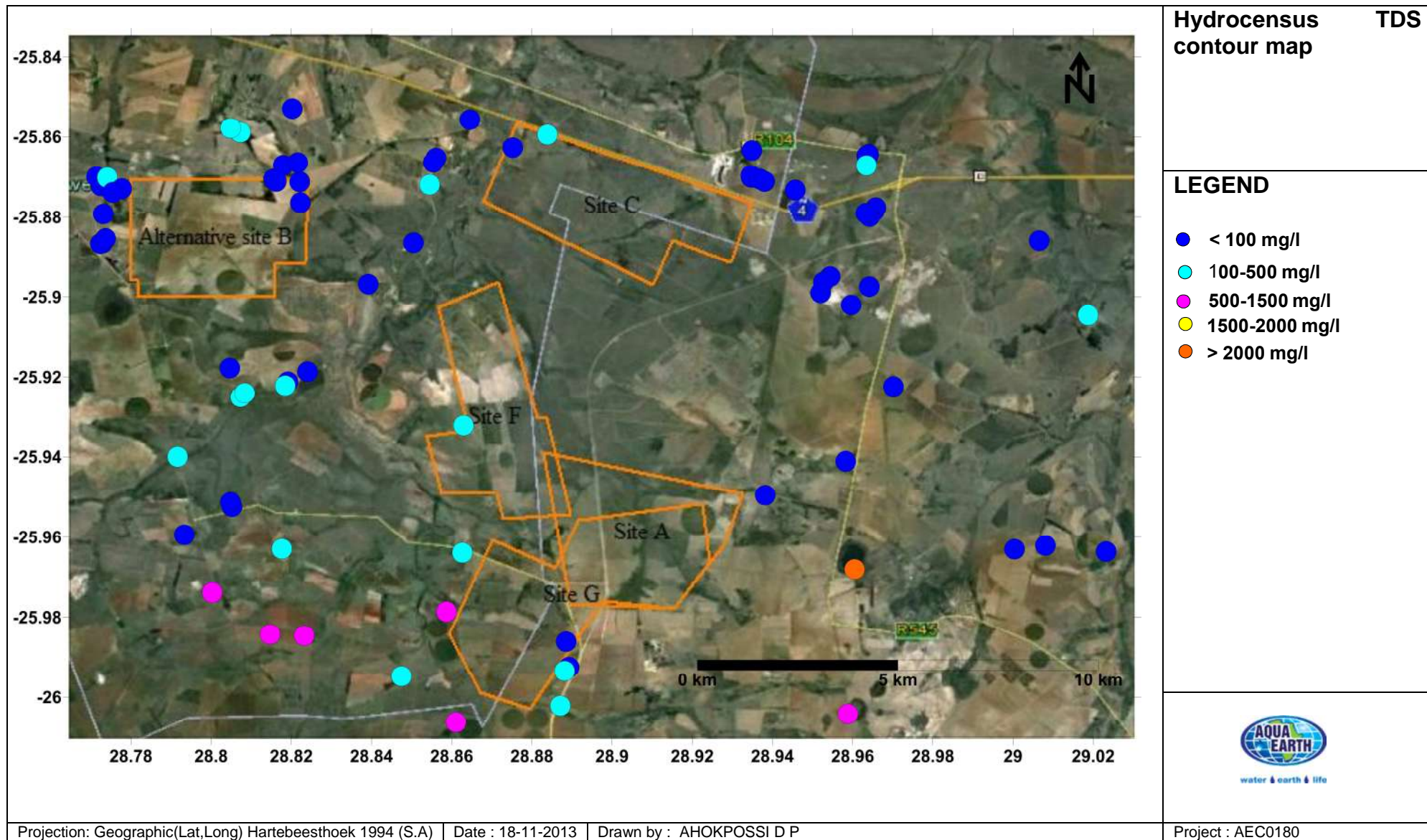
Figure 16: Hydrocensus results: TDS map
