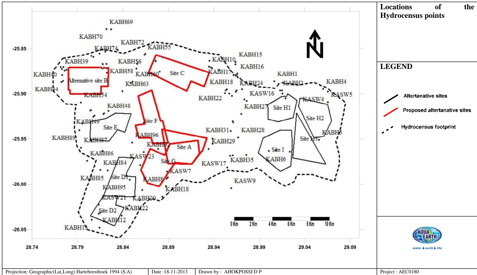
Figure 10: Plan showing hydrocensus points locations
