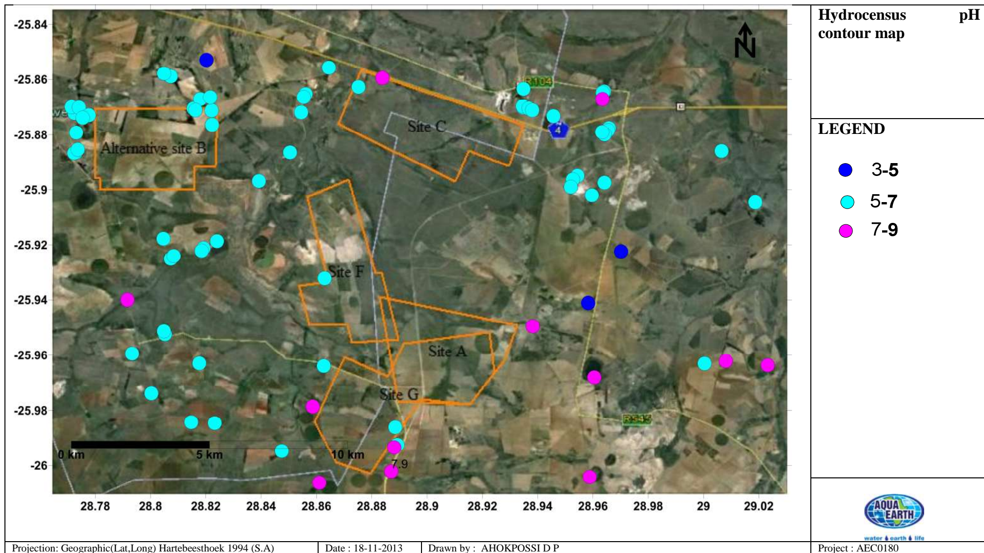
Figure 15: Hydrocensus results: pH map
