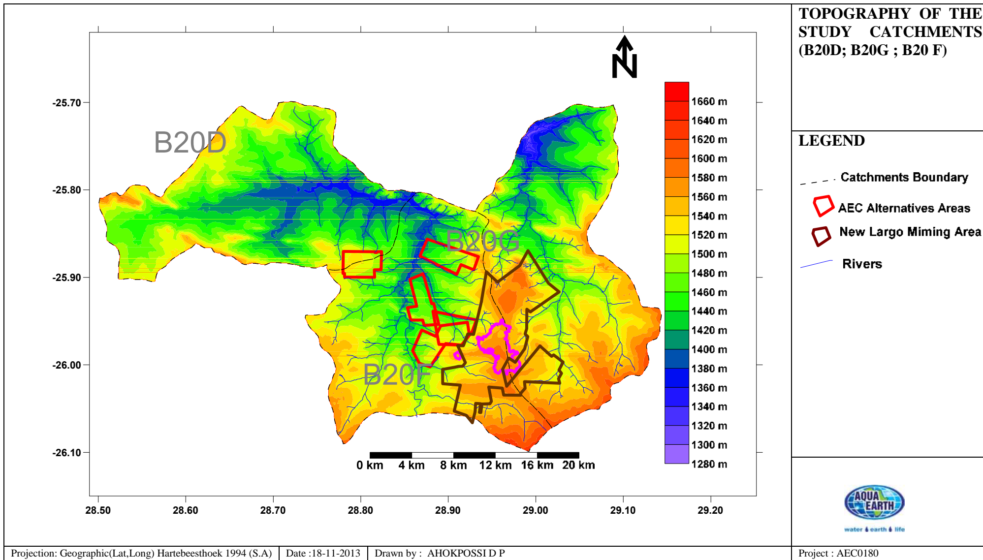
Figure 4: Topography of the study catchments
