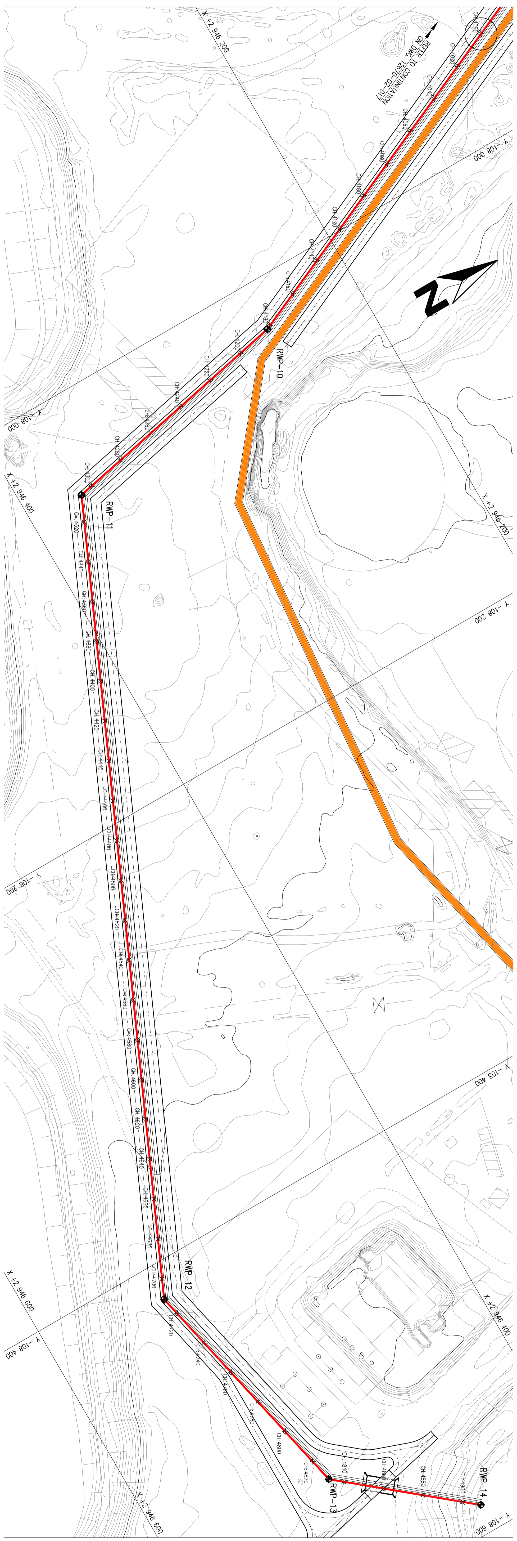
LAYOUT OF RETURN WATER PIPELINE 1:1000
