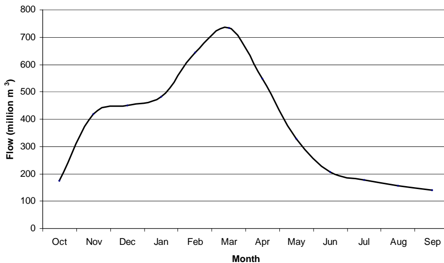
Figure 8.2: Monthly median flows, in millions of cubic metres of water, at the gauging point D7H005 in the Orange River at Upington. Source - Department of Water Affairs and Forestry.
