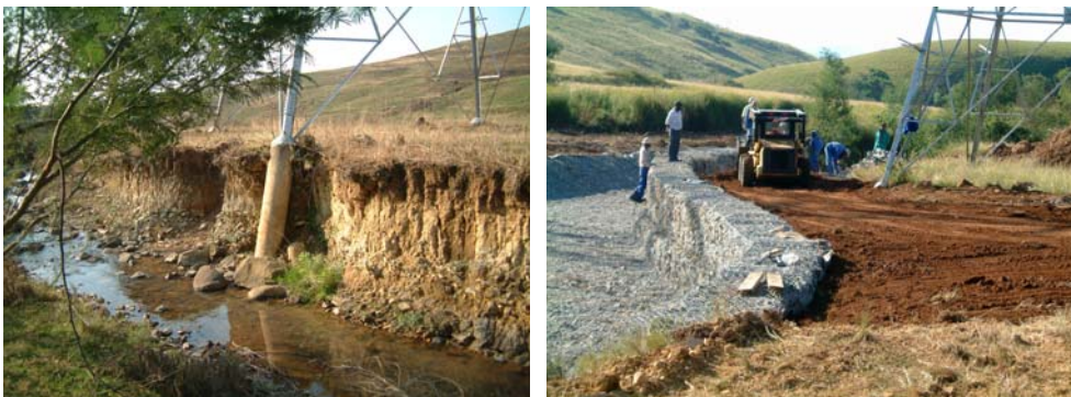
Figure 1: The photo on the left shows the foundation of a tower exposed by erosion. The photo on the right shows the extensive and costly remediation by using gabions and reno mattresses. Also note the use of good topsoil that will permit the re-establishment of vegetation around the tower (photos Jorge Correia).
