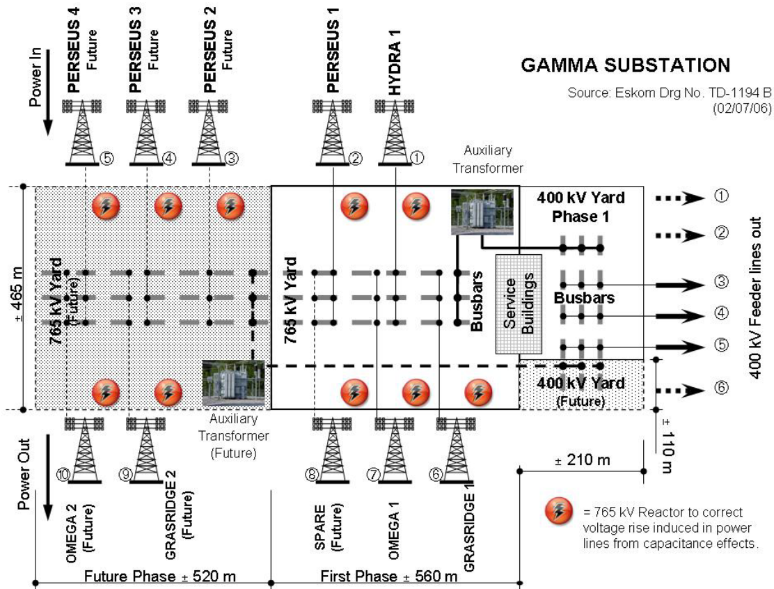
Figure 5 Schematic diagram of the proposed Gamma Sub-station layout
