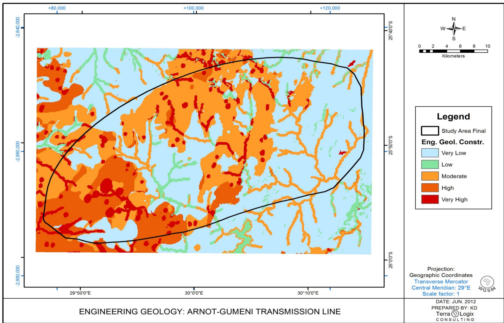
Figure 37: it represents the engineering geological constraints of the study area
