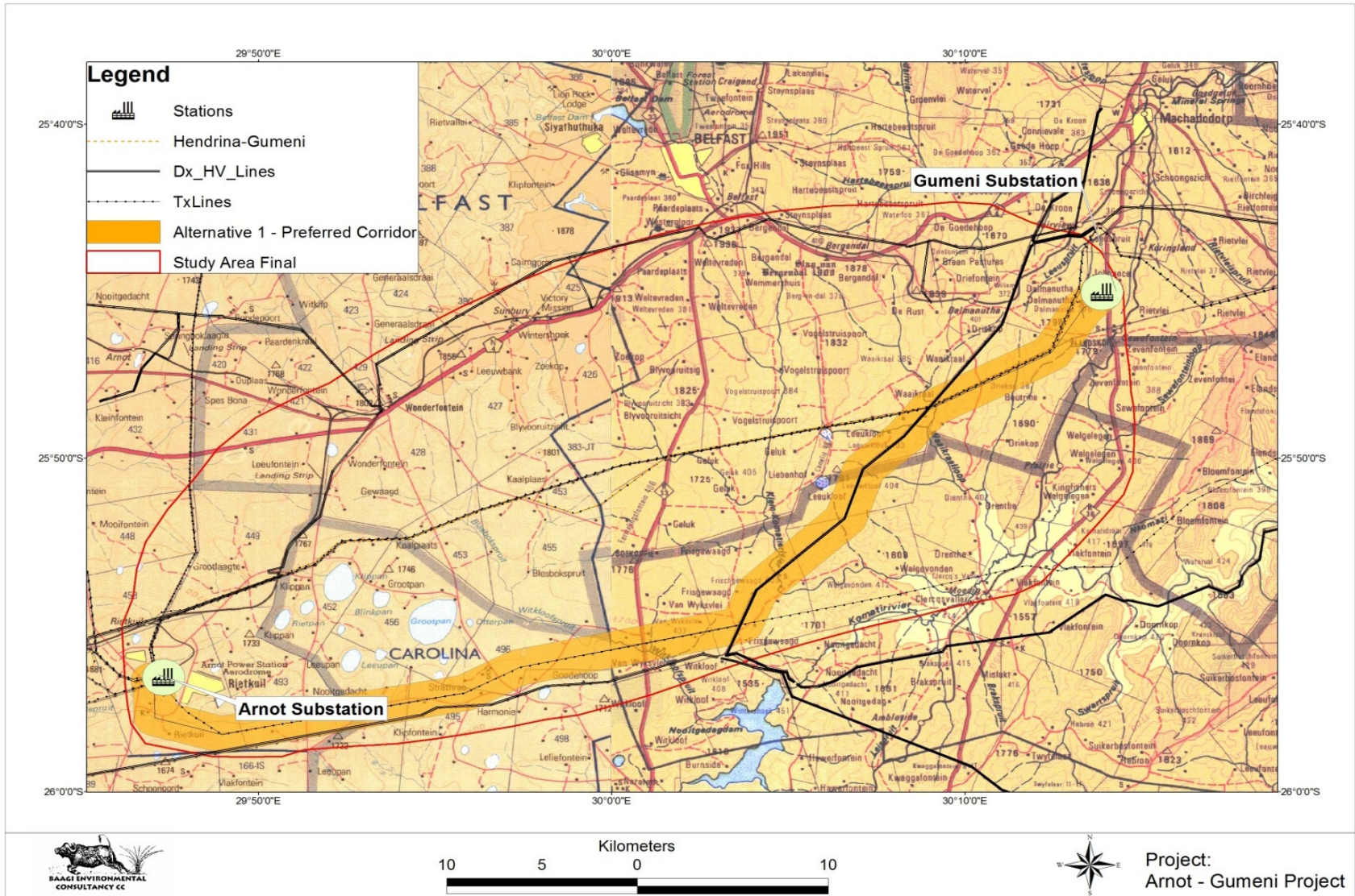
Figure 40: Configuration map of the preferred alternative 1 (Orange corridor)
