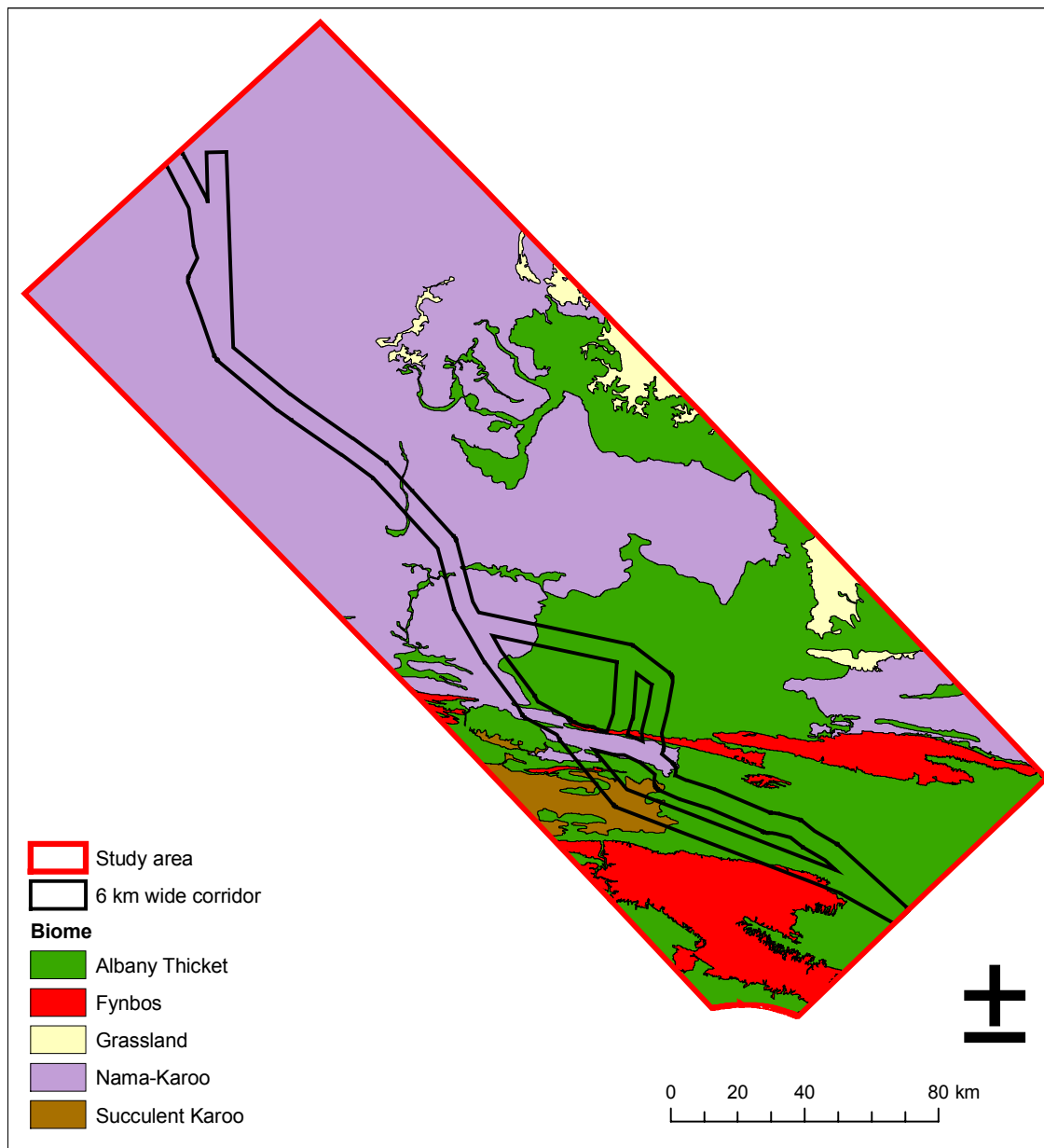
Figure 3. Biomes in the study area
