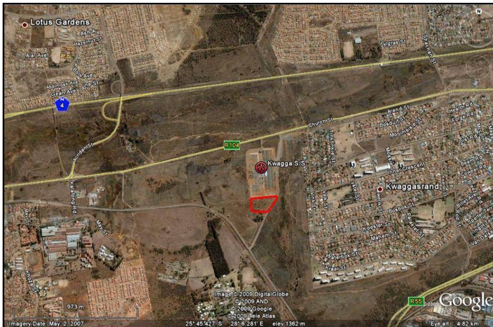
Figure 1: Proposed extensions at the Kwagga substation
