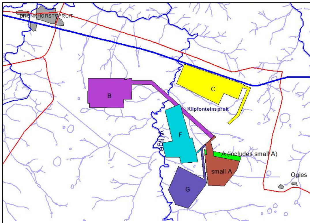
Figure 1-1. Location of the study area, site alternatives and potential conveyor routes.
