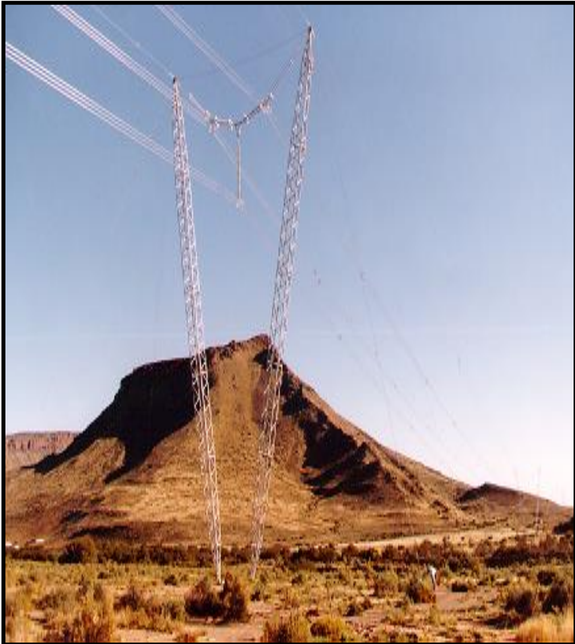
Figure 8: Guyed V structure
