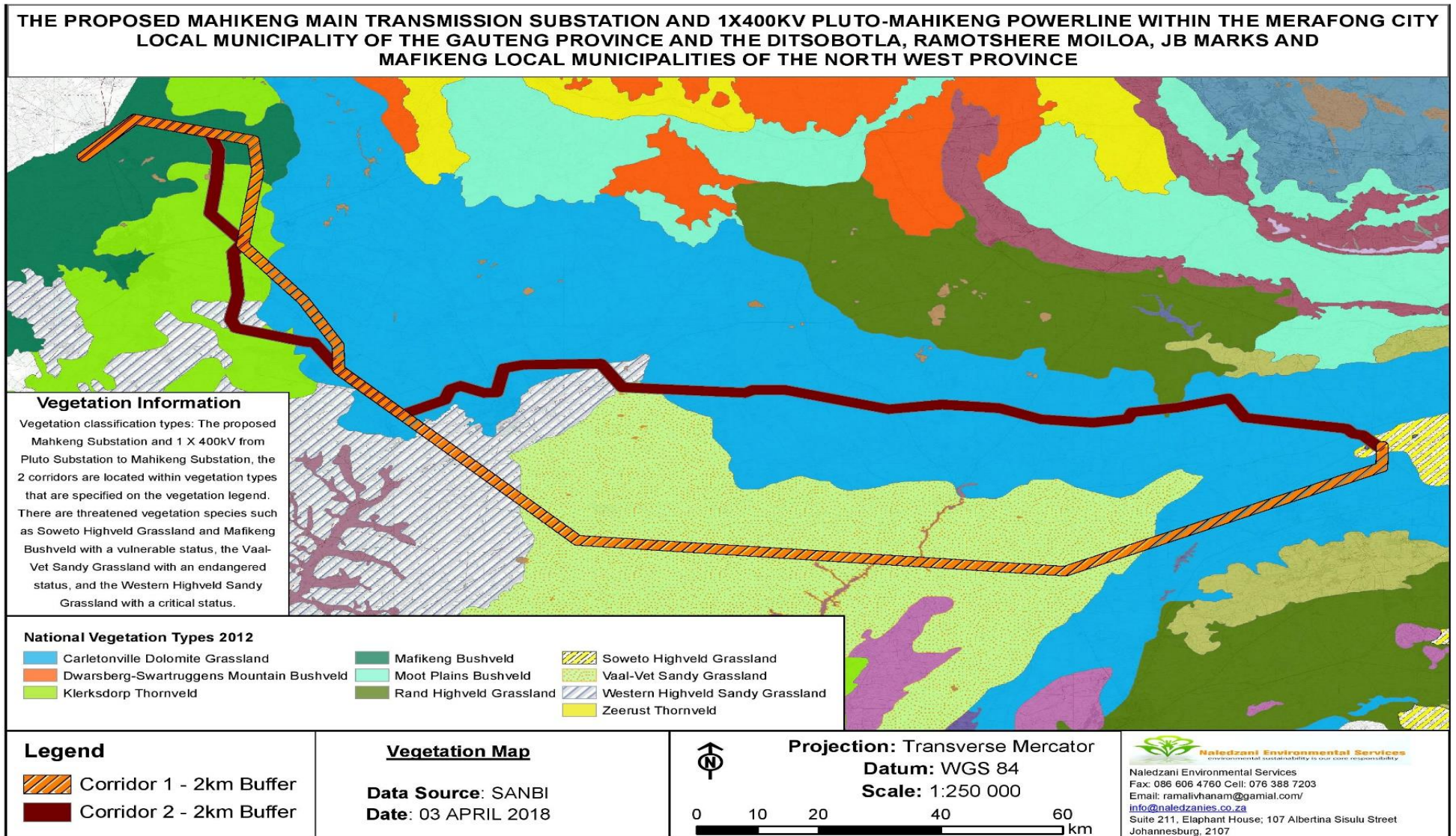
Figure 42: Vegetation Map
