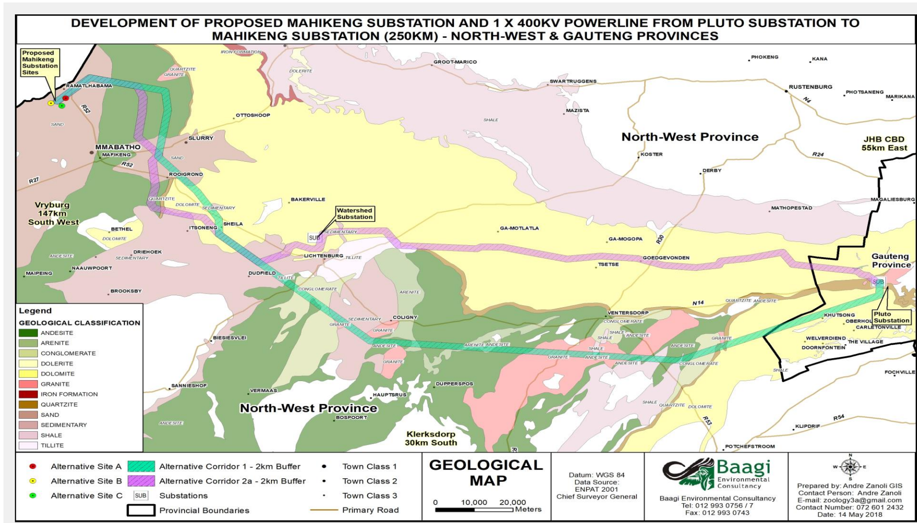
Figure 46: Geological Map
