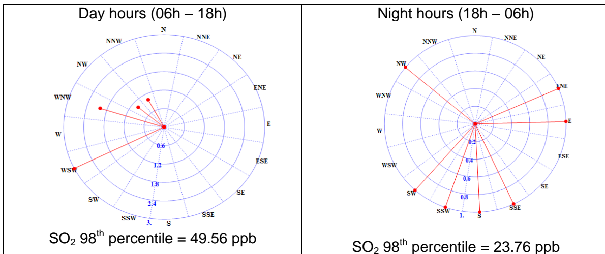
Figure 4: SO 2 highest hourly concentrations for event roses for February 2017
