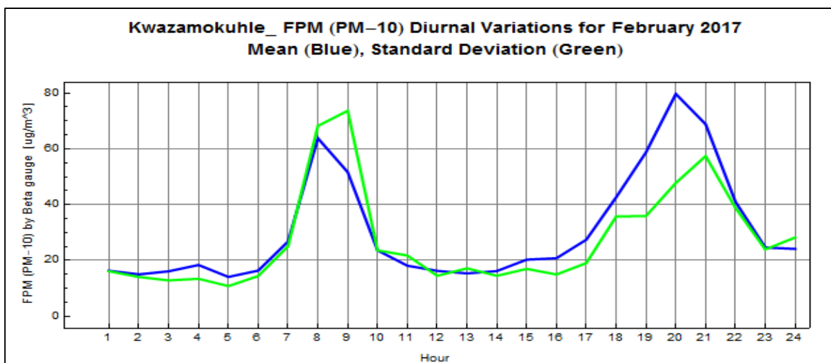
Figure 8: Diurnal variation of PM 10 concentrations at KwaZamokhule for February 2017
