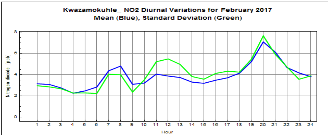
Figure 5: Diurnal variation of NO 2 hourly at KwaZamokuhle for February 2017
