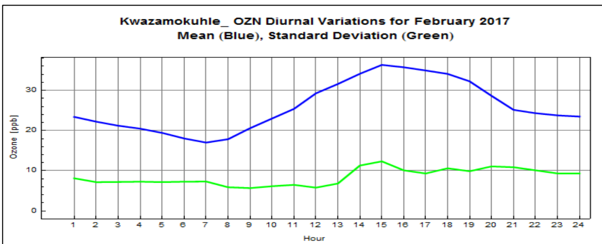
Figure 11: Diurnal variation of Ozone concentrations at KwaZamokuhle for February 2017
