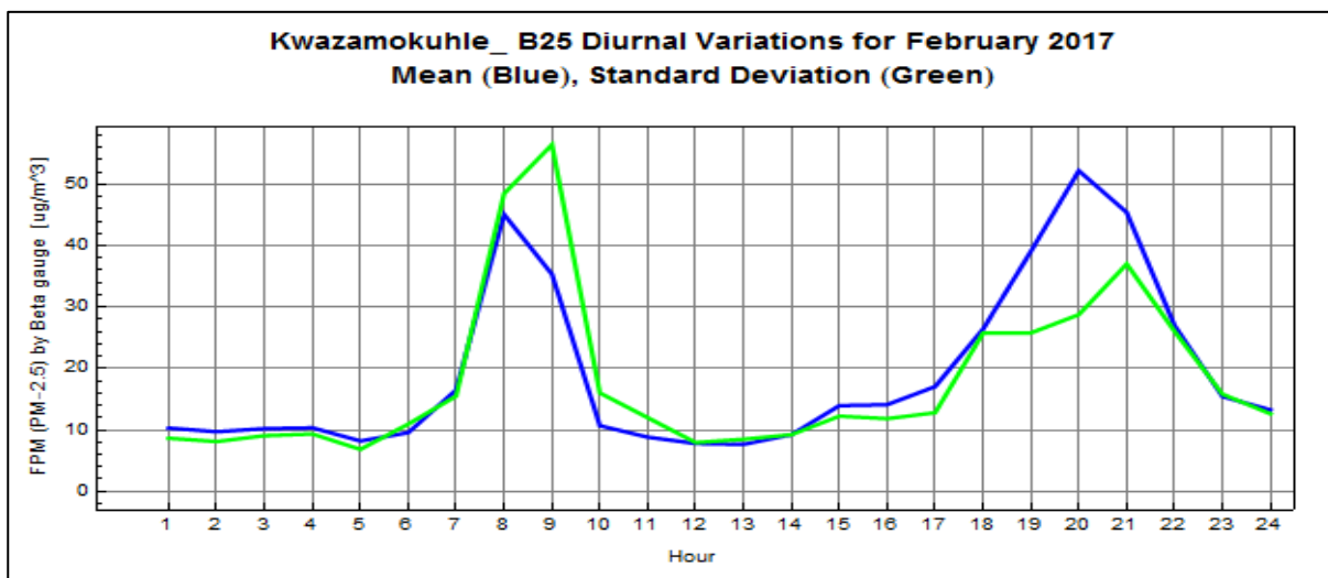
Figure 7: Diurnal variation of PM 2.5 concentrations at KwaZamokhule for February 2017
