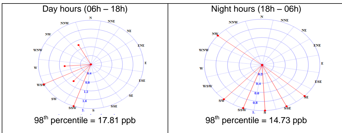
Figure 6: NO 2 hourly mean 98 th percentile event roses during day and night times
