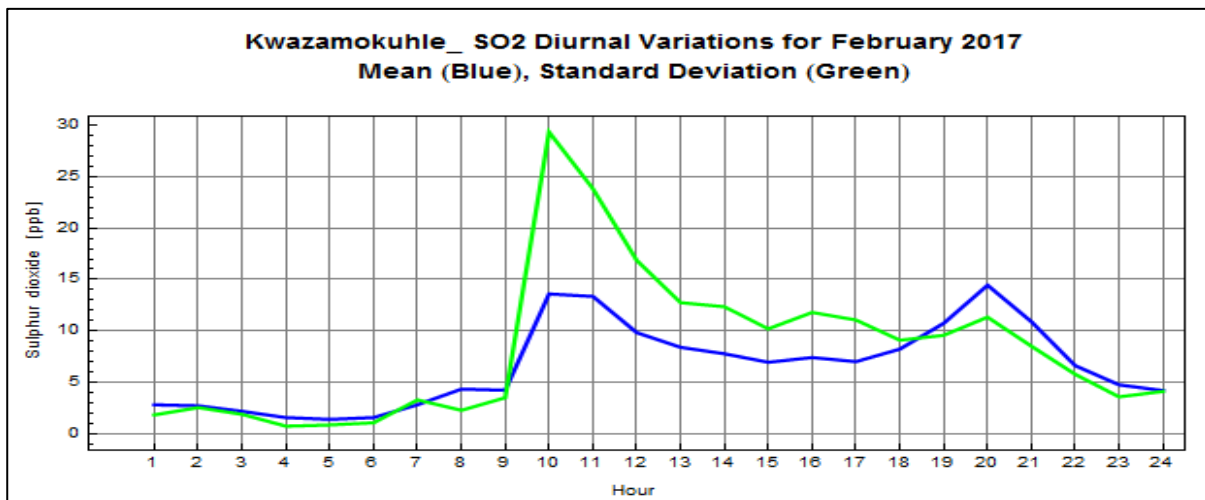
Figure 3: Diurnal variation of SO 2 hourly at KwaZamokuhle for February 2017
