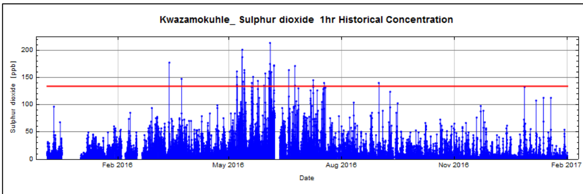
Figure 12: SO 2 1hr mean concentration
